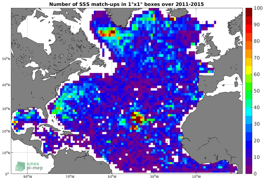
Figure 4: Number of SSS match-ups between Argo SSS and the Aquarius-L4-IPRC-V5-MONTHLY SSS product for the North Atlantic Ocean Pi-MEP region over 1^\circ \times 1^\circ boxes and for the full satellite product period.
