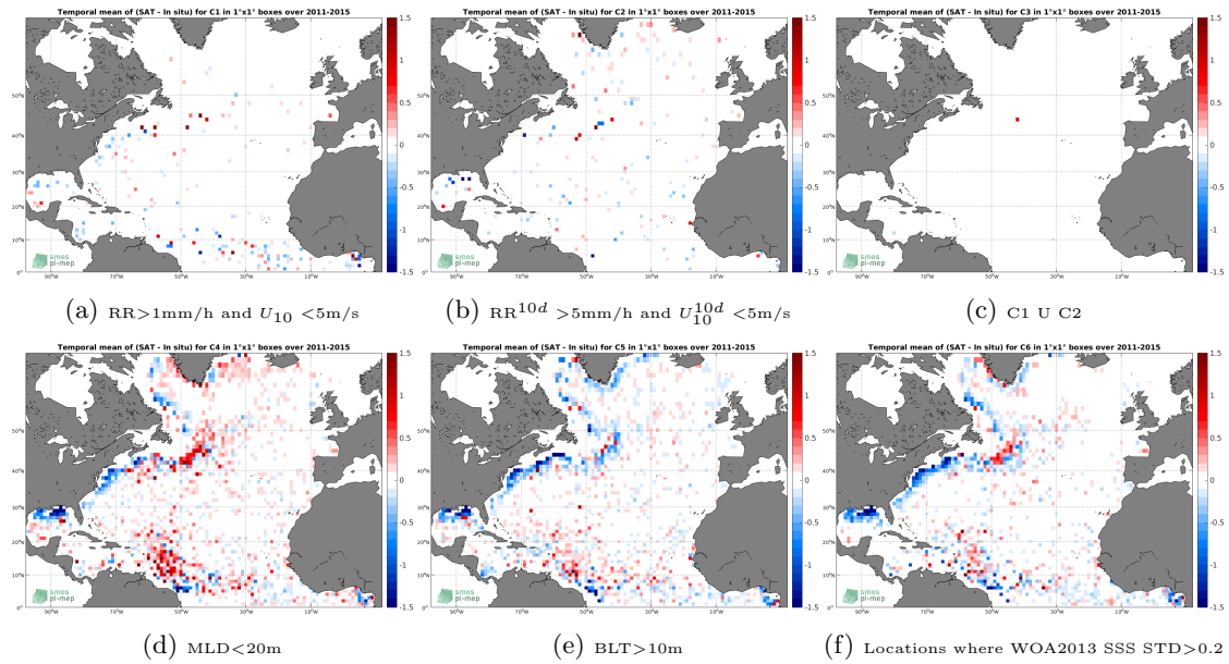
Figure 12: Temporal mean gridded over spatial boxes of size 1^\circ \times 1^\circ of \Delta\text{SSS} (Aquarius-L4-IPRC-V5-MONTHLY - Argo) for 6 different subdatasets corresponding to: RR > 1\text{mm/h} and U_{10} < 5\text{m/s} (a), RR^{10d} > 5\text{mm/h} and U_{10}^{10d} < 5\text{m/s} (b), C1 U C2 (c), MLD < 20\text{m} (d), BLT > 10\text{m} (e), Locations where WOA2013 SSS STD > 0.2 (f).
