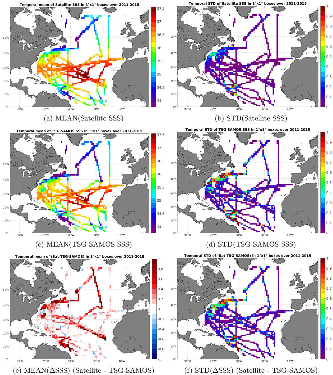
Figure 6: Temporal mean (left) and STD (right) of SSS from Aquarius-L4-IPRC-V4-WEEKLY (top), TSG-SAMOS (middle), and of \Delta SSS (Satellite - TSG-SAMOS). Only match-up pairs are used to generate these maps.
