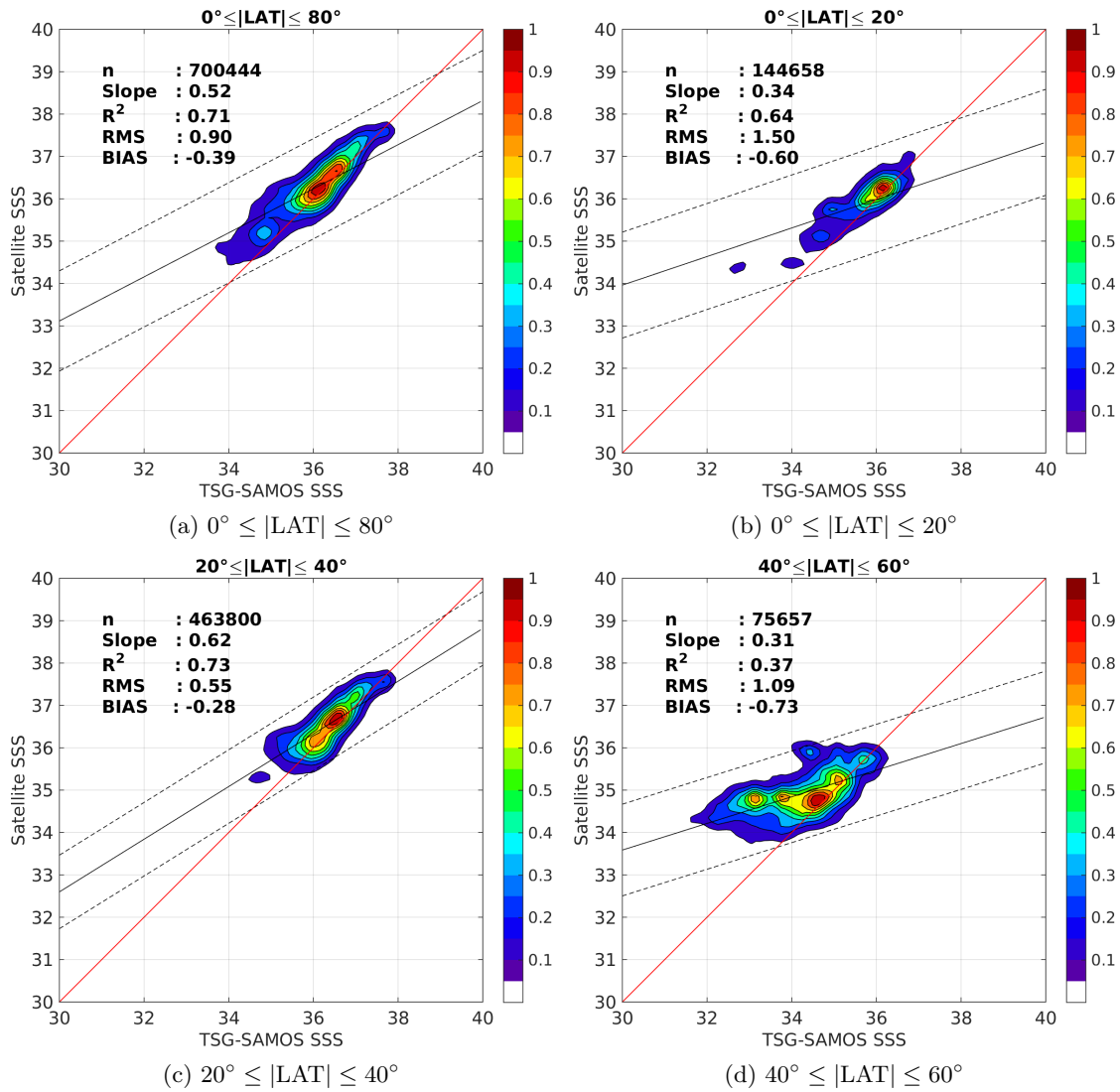
Figure 9: Contour maps of the concentration of Aquarius-L4-IPRC-V4-WEEKLY SSS (y-axis) versus TSG-SAMOS SSS (x-axis) at match-up pairs for different latitude bands. For each plot, the red line shows x=y . The black thin and dashed lines indicate a linear fit through the data cloud and the \pm 95\% confidence levels, respectively. The number match-up pairs n , the slope and R^2 coefficient of the linear fit, the root mean square (RMS) and the mean bias between satellite and in situ data are indicated for each latitude band in each plots.
