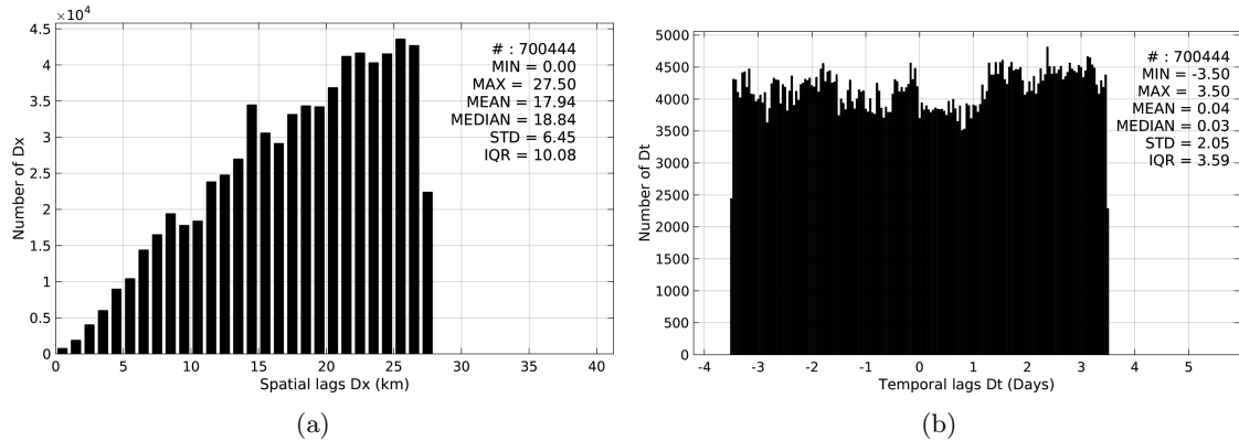
Figure 5: Histograms of the spatial (a) and temporal (b) lags between the time of the TSG-SAMOS measurements and the date of the corresponding Aquarius-L4-IPRC-V4-WEEKLY SSS product.
