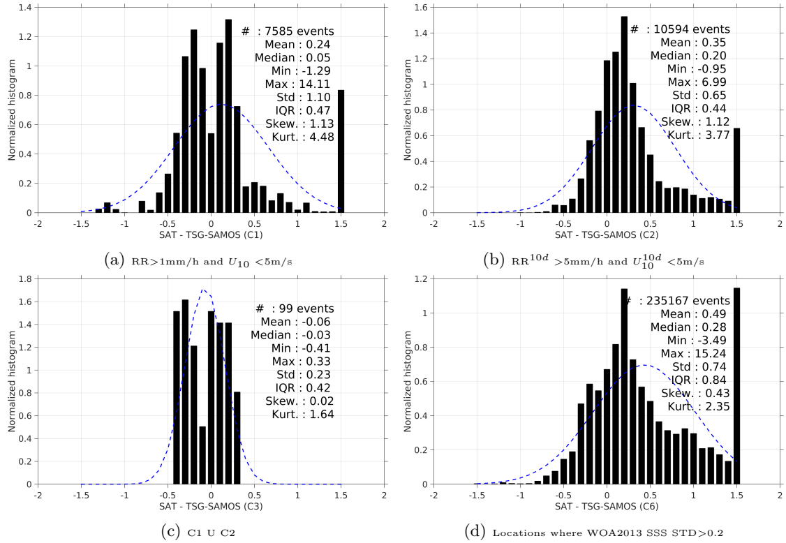
Figure 13: Normalized histogram of \Delta SSS (Aquarius-L4-IPRC-V4-WEEKLY - TSG-SAMOS) for 6 different subdatasets corresponding to: RR > 1\text{mm/h} and U_{10} < 5\text{m/s} (a), RR^{10d} > 5\text{mm/h} and U_{10}^{10d} < 5\text{m/s} (b), C1 U C2 (c), Locations where WOA2013 SSS STD > 0.2 (d).
