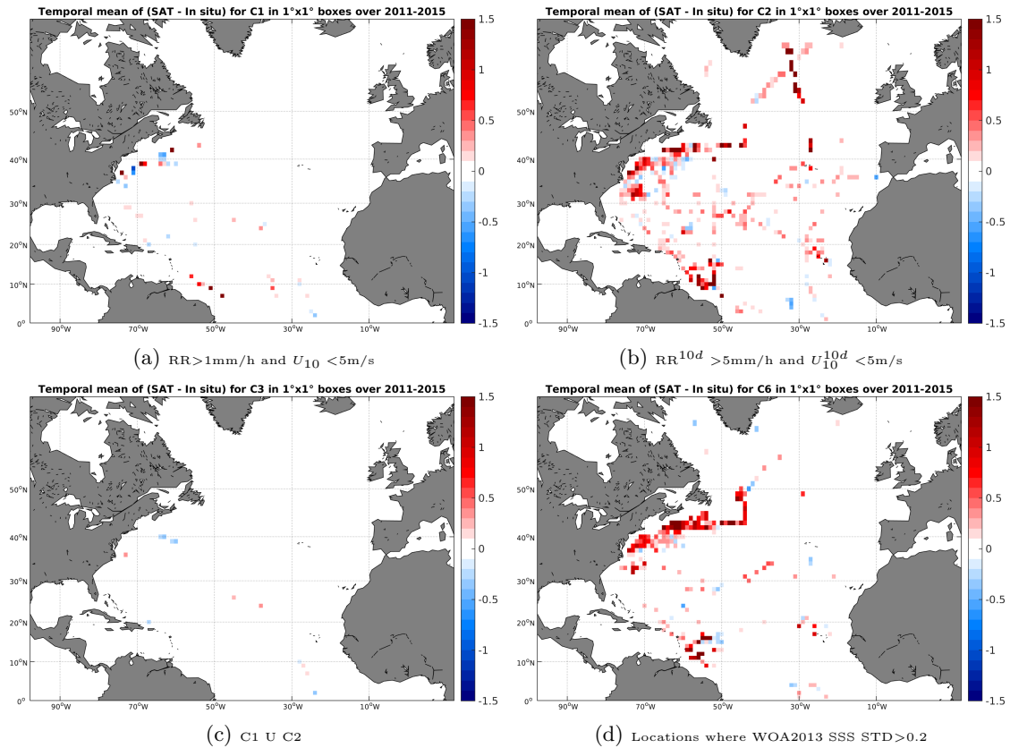
Figure 12: Temporal mean gridded over spatial boxes of size 1^\circ \times 1^\circ of \Delta SSS (Aquarius-L4-IPRC-V4-WEEKLY - TSG-SAMOS) for 4 different subdatasets corresponding to:RR>1mm/h and U_{10} < 5 m/s (a), RR 10d > 5mm/h and U_{10}^{10d} < 5 m/s (b), C1 U C2 (c),Locations where WOA2013 SSS STD>0.2 (d).
