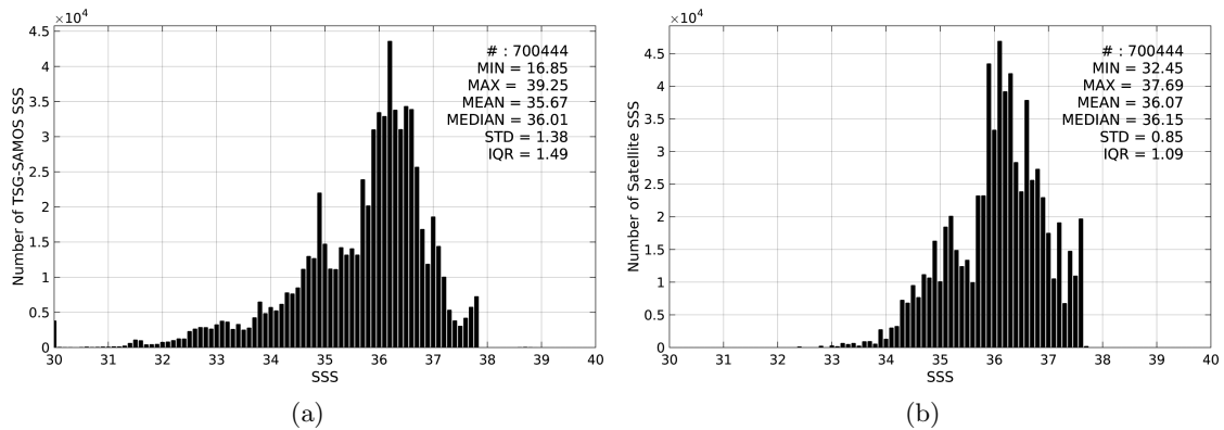
Figure 2: Histograms of SSS from TSG-SAMOS (a) and Aquarius-L4-IPRC-V4-WEEKLY (b) considering all match-up pairs per bins of 0.1 over the North Atlantic Ocean Pi-MEP region and for the full satellite product period.
