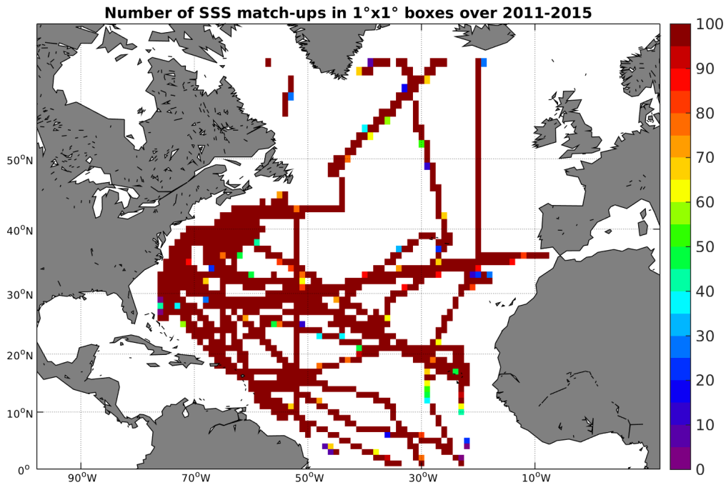
Figure 4: Number of SSS match-ups between TSG-SAMOS SSS and the Aquarius-L4-IPRC-V4-WEEKLY SSS product for the North Atlantic Ocean Pi-MEP region over 1^\circ \times 1^\circ boxes and for the full satellite product period.
