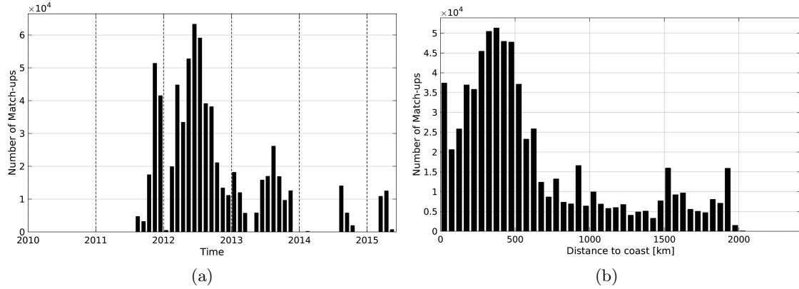
Figure 1: Number of match-ups between TSG-SAMOS and Aquarius-L4-IPRC-V4-WEEKLY SSS as a function of time (a) and as function of the distance to coast (b) over the North Atlantic Ocean Pi-MEP region and for the full satellite product period.
