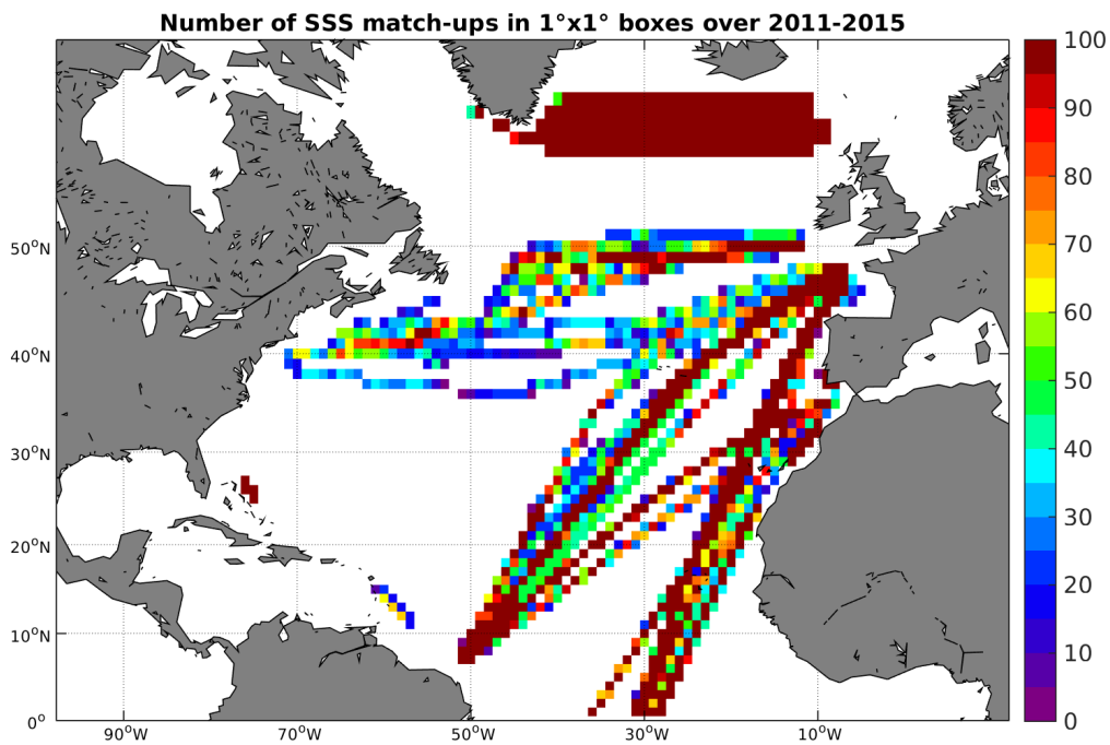
Figure 4: Number of SSS match-ups between TSG-LEGOS-DM SSS and the Aquarius-L4-IPRC-V4-WEEKLY SSS product for the North Atlantic Ocean Pi-MEP region over 1^\circ \times 1^\circ boxes and for the full satellite product period.
