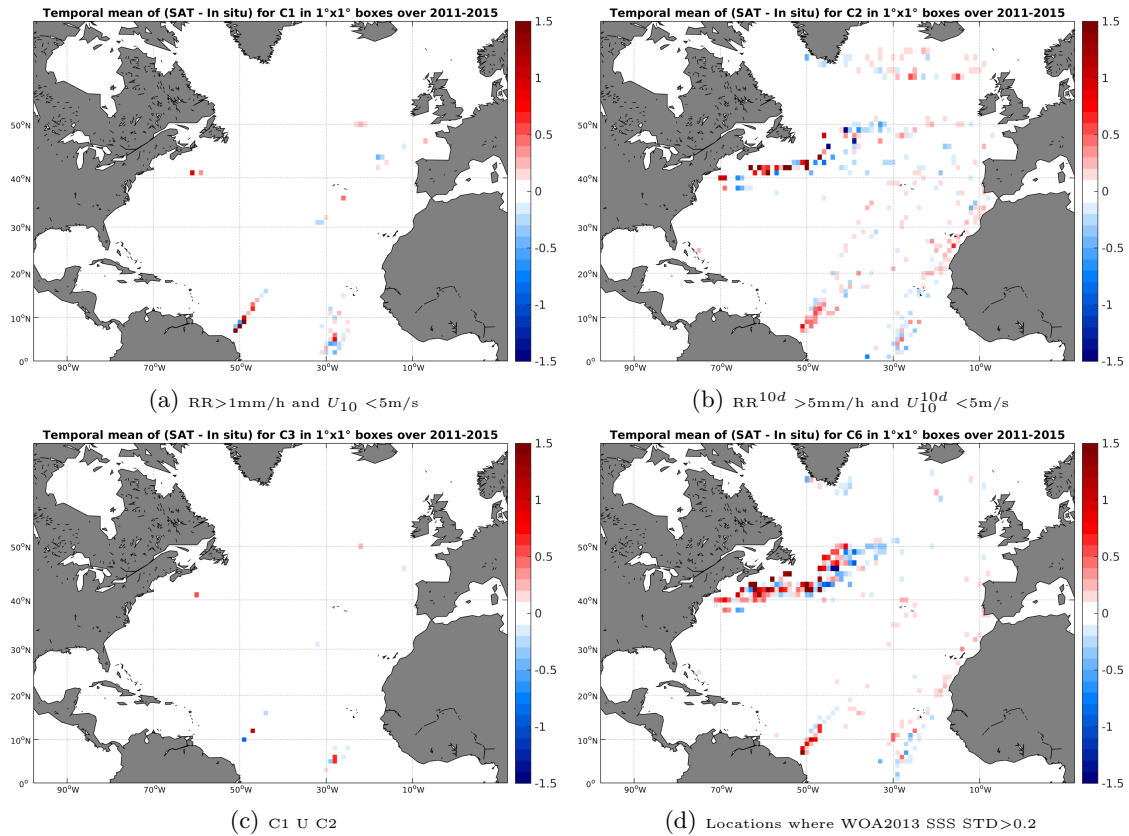
Figure 12: Temporal mean gridded over spatial boxes of size 1^\circ \times 1^\circ of \Delta SSS (Aquarius-L4-IPRC-V4-WEEKLY - TSG-LEGOS-DM) for 4 different subdatasets corresponding to:RR>1mm/h and U_{10} < 5m/s (a), RR^{10d} > 5mm/h and U_{10}^{10d} < 5m/s (b), C1 U C2 (c),Locations where WOA2013 SSS STD>0.2 (d).
