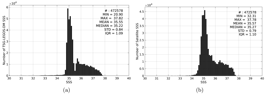
Figure 2: Histograms of SSS from TSG-LEGOS-DM (a) and Aquarius-L4-IPRC-V4-WEEKLY (b) considering all match-up pairs per bins of 0.1 over the North Atlantic Ocean Pi-MEP region and for the full satellite product period.
