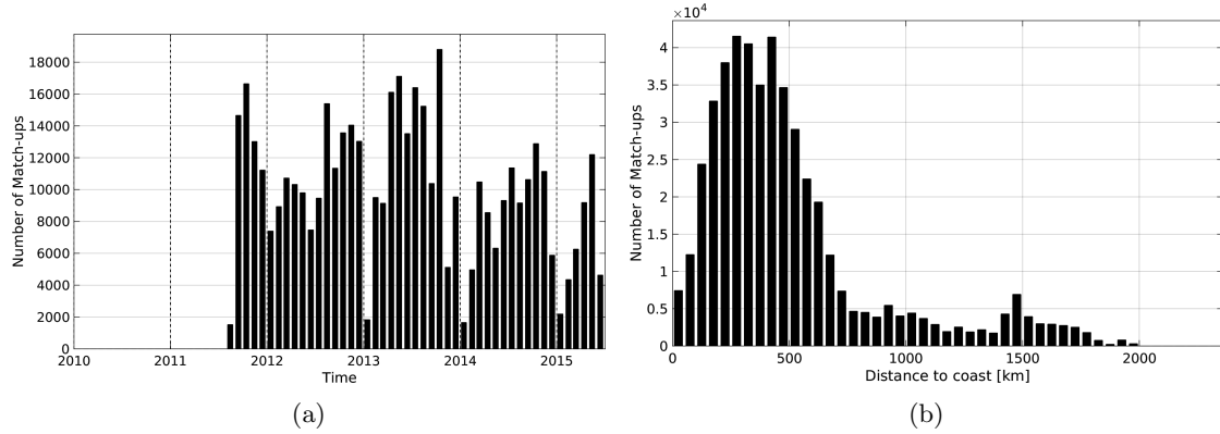
Figure 1: Number of match-ups between TSG-LEGOS-DM and Aquarius-L4-IPRC-V4-WEEKLY SSS as a function of time (a) and as function of the distance to coast (b) over the North Atlantic Ocean Pi-MEP region and for the full satellite product period.
