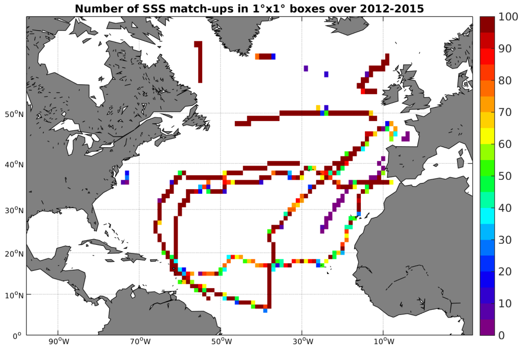
Figure 4: Number of SSS match-ups between TSG-GOSUD-Sailing-ship SSS and the Aquarius-L4-IPRC-V4-WEEKLY SSS product for the North Atlantic Ocean Pi-MEP region over 1^\circ \times 1^\circ boxes and for the full satellite product period.
