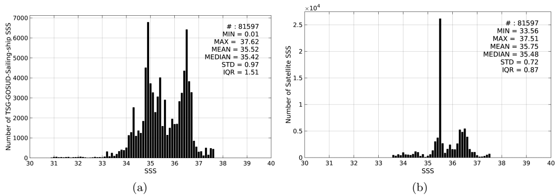
Figure 2: Histograms of SSS from TSG-GOSUD-Sailing-ship (a) and Aquarius-L4-IPRC-V4-WEEKLY (b) considering all match-up pairs per bins of 0.1 over the North Atlantic Ocean Pi-MEP region and for the full satellite product period.
