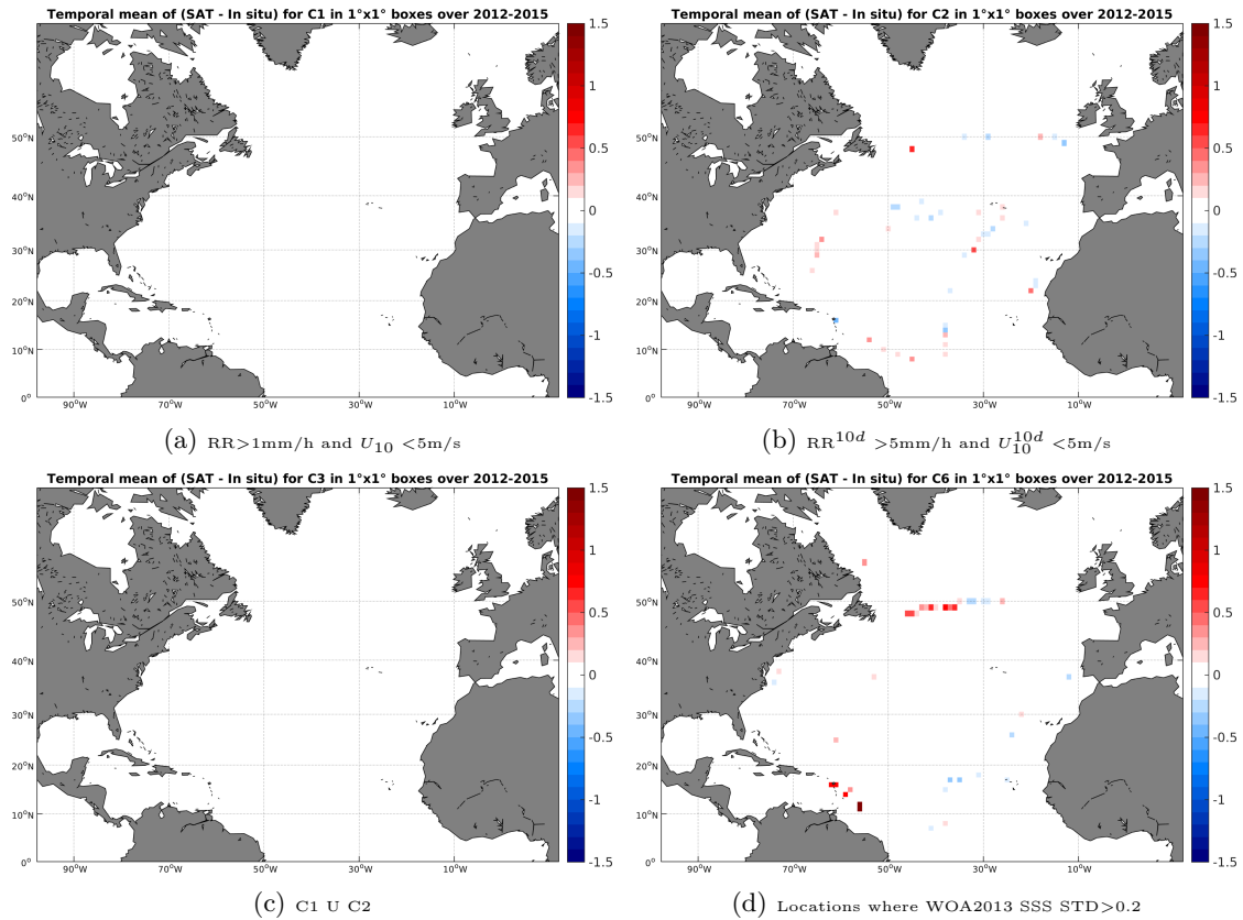
Figure 12: Temporal mean gridded over spatial boxes of size 1^\circ \times 1^\circ of \Delta SSS (Aquarius-L4-IPRC-V4-WEEKLY - TSG-GOSUD-Sailing-ship) for 4 different subdatasets corresponding to: RR > 1\text{mm/h} and U_{10} < 5\text{m/s} (a), RR^{10d} > 5\text{mm/h} and U_{10}^{10d} < 5\text{m/s} (b), C1 U C2 (c), Locations where WOA2013 SSS STD > 0.2 (d).
