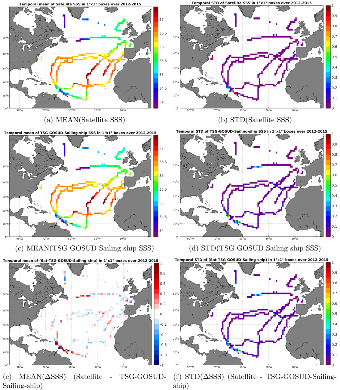
Figure 6: Temporal mean (left) and STD (right) of SSS from Aquarius-L4-IPRC-V4-WEEKLY (top), TSG-GOSUD-Sailing-ship (middle), and of \Delta SSS (Satellite - TSG-GOSUD-Sailing-ship). Only match-up pairs are used to generate these maps.
