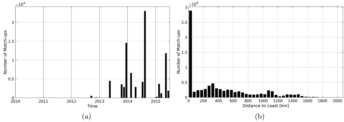
Figure 1: Number of match-ups between TSG-GOSUD-Sailing-ship and Aquarius-L4-IPRC-V4-WEEKLY SSS as a function of time (a) and as function of the distance to coast (b) over the North Atlantic Ocean Pi-MEP region and for the full satellite product period.
