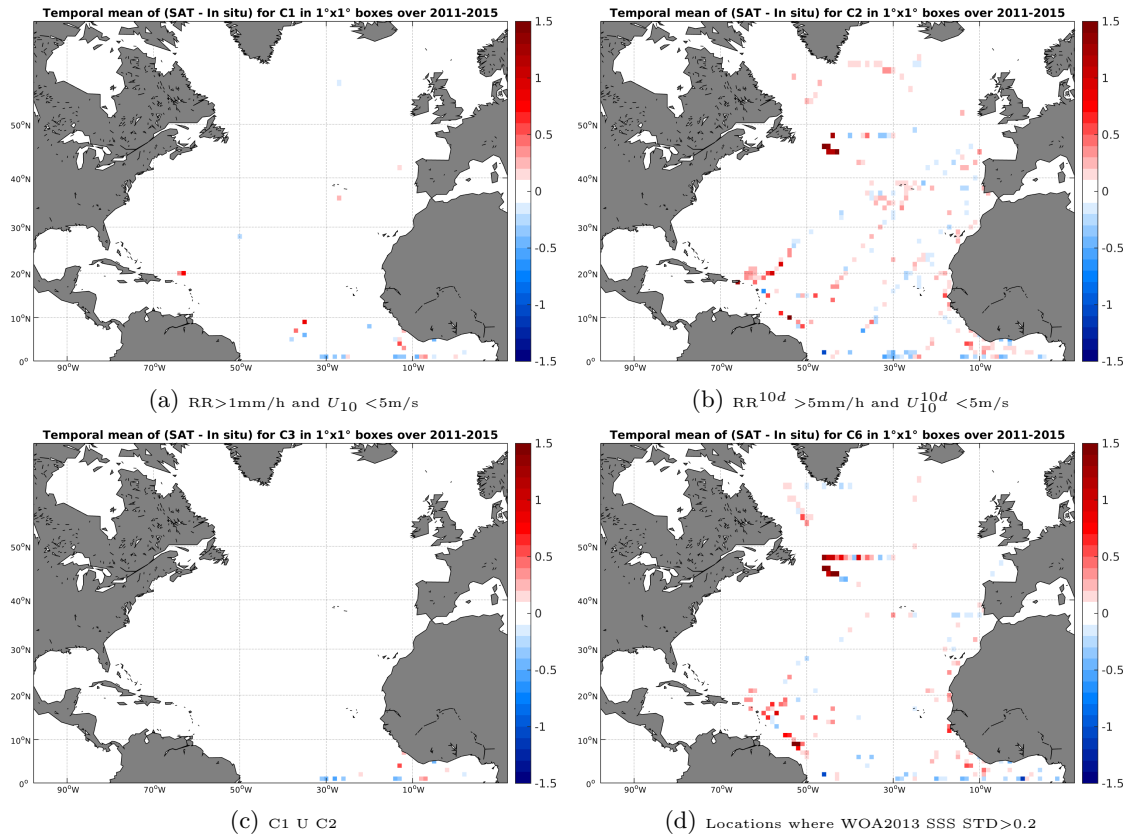
Figure 12: Temporal mean gridded over spatial boxes of size 1°x1° of \Delta SSS (Aquarius-L4-IPRC-V4-WEEKLY - TSG-GOSUD-Research-vessel) for 4 different subdatasets corresponding to: RR > 1\text{mm/h} and U_{10} < 5\text{m/s} (a), RR^{10d} > 5\text{mm/h} and U_{10}^{10d} < 5\text{m/s} (b), C1 U C2 (c), Locations where WOA2013 SSS STD > 0.2 (d).
