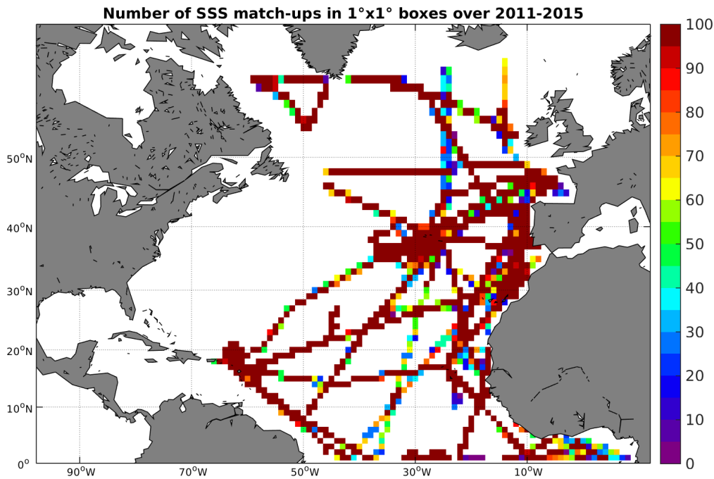
Figure 4: Number of SSS match-ups between TSG-GOSUD-Research-vessel SSS and the Aquarius-L4-IPRC-V4-WEEKLY SSS product for the North Atlantic Ocean Pi-MEP region over 1°x1° boxes and for the full satellite product period.
