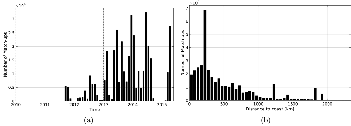
Figure 1: Number of match-ups between TSG-GOSUD-Research-vessel and Aquarius-L4-IPRC-V4-WEEKLY SSS as a function of time (a) and as function of the distance to coast (b) over the North Atlantic Ocean Pi-MEP region and for the full satellite product period.
