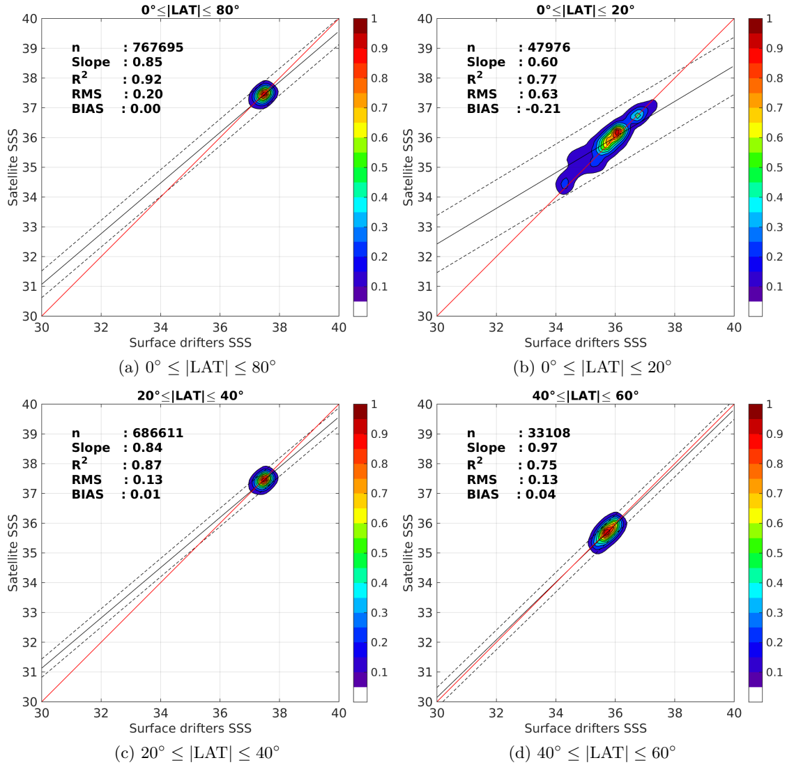
Figure 8: Contour maps of the concentration of Aquarius-L4-IPRC-V4-WEEKLY SSS (y-axis) versus Surface drifters SSS (x-axis) at match-up pairs for different latitude bands. For each plot, the red line shows x=y . The black thin and dashed lines indicate a linear fit through the data cloud and the \pm 95\% confidence levels, respectively. The number match-up pairs n , the slope and R^2 coefficient of the linear fit, the root mean square (RMS) and the mean bias between satellite and in situ data are indicated for each latitude band in each plots.
