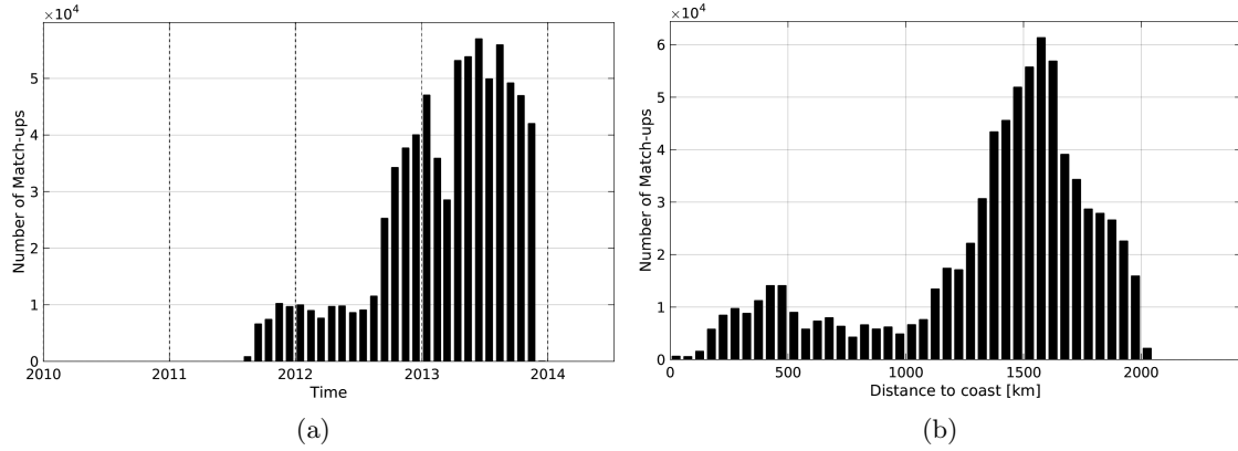
Figure 1: Number of match-ups between Surface drifters and Aquarius-L4-IPRC-V4-WEEKLY SSS as a function of time (a) and as function of the distance to coast (b) over the North Atlantic Ocean Pi-MEP region and for the full satellite product period.
