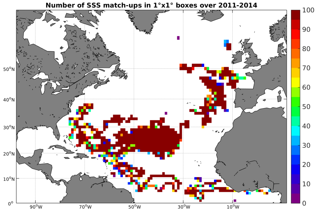
Figure 3: Number of SSS match-ups between Surface drifters SSS and the Aquarius-L4-IPRC-V4-WEEKLY SSS product for the North Atlantic Ocean Pi-MEP region over 1^\circ \times 1^\circ boxes and for the full satellite product period.
