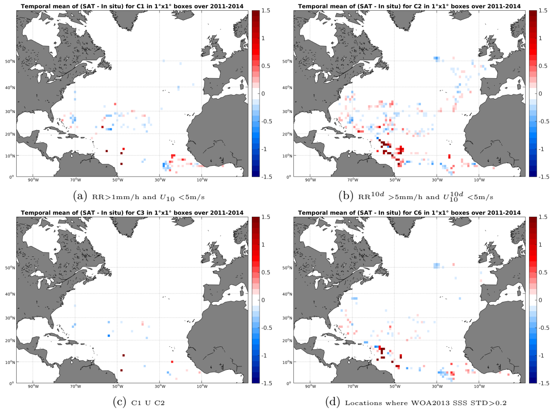
Figure 11: Temporal mean gridded over spatial boxes of size 1^\circ \times 1^\circ of \Delta SSS (Aquarius-L4-IPRC-V4-WEEKLY - Surface drifters) for 4 different subdatasets corresponding to: RR > 1mm/h and U_{10} < 5\text{m/s} (a), RR^{10d} > 5\text{mm/h} and U_{10}^{10d} < 5\text{m/s} (b), C1 U C2 (c), Locations where WOA2013 SSS STD > 0.2 (d).
