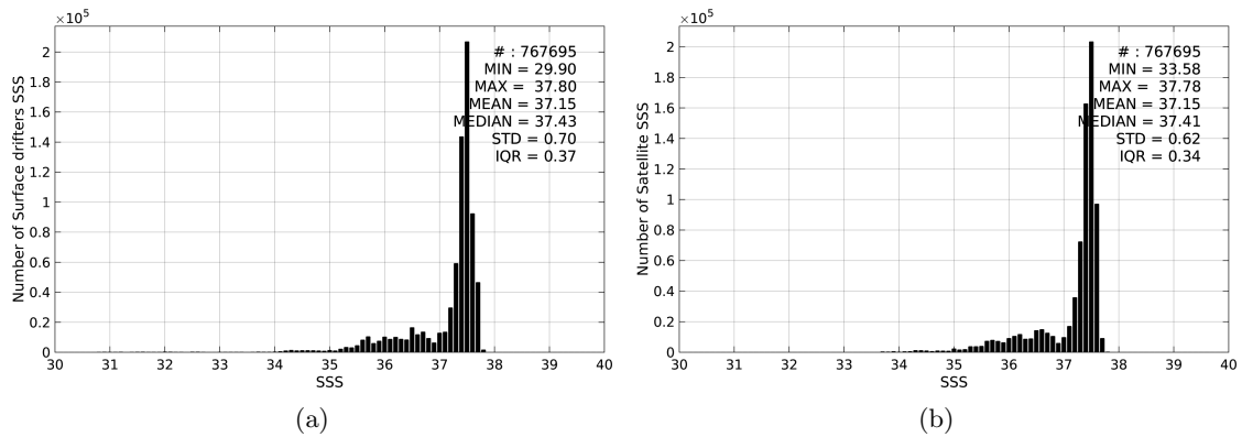
Figure 2: Histograms of SSS from Surface drifters (a) and Aquarius-L4-IPRC-V4-WEEKLY (b) considering all match-up pairs per bins of 0.1 over the North Atlantic Ocean Pi-MEP region and for the full satellite product period.
