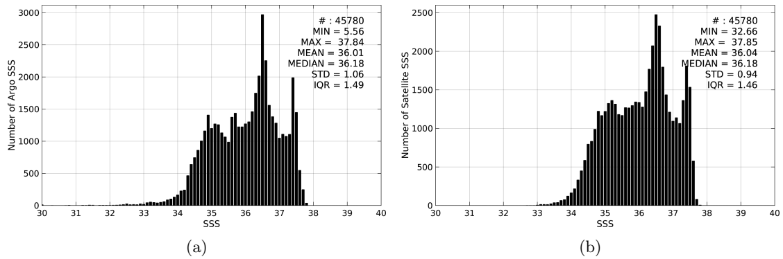
Figure 2: Histograms of SSS from Argo (a) and Aquarius-L4-IPRC-V4-WEEKLY (b) considering all match-up pairs per bins of 0.1 over the North Atlantic Ocean Pi-MEP region and for the full satellite product period.
