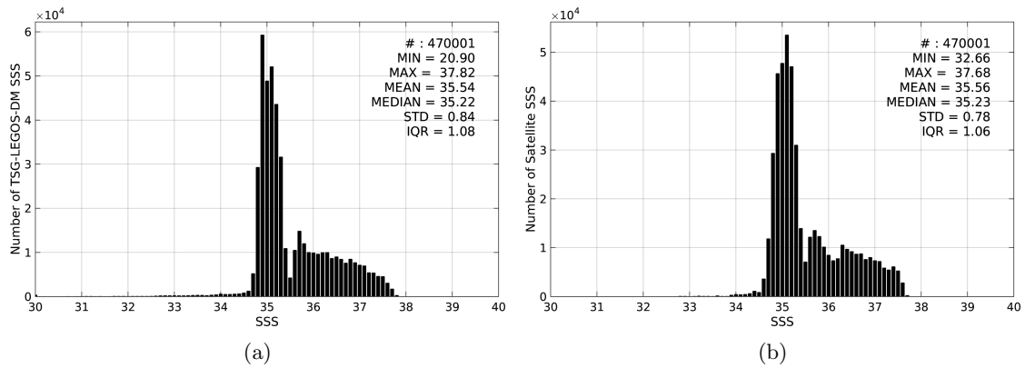
Figure 2: Histograms of SSS from TSG-LEGOS-DM (a) and Aquarius-L4-IPRC-V4-MONTHLY (b) considering all match-up pairs per bins of 0.1 over the North Atlantic Ocean Pi-MEP region and for the full satellite product period.
