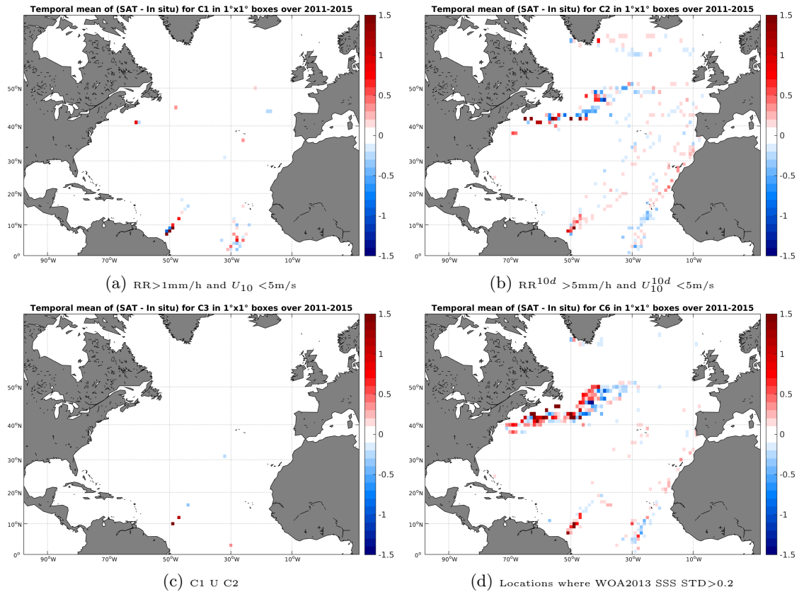
Figure 12: Temporal mean gridded over spatial boxes of size 1^\circ \times 1^\circ of \Delta SSS (Aquarius-L4-IPRC-V4-MONTHLY - TSG-LEGOS-DM) for 4 different subdatasets corresponding to:RR>1mm/h and U_{10} < 5 m/s (a), RR 10d > 5mm/h and U_{10}^{10d} < 5 m/s (b), C1 U C2 (c),Locations where WOA2013 SSS STD>0.2 (d).
