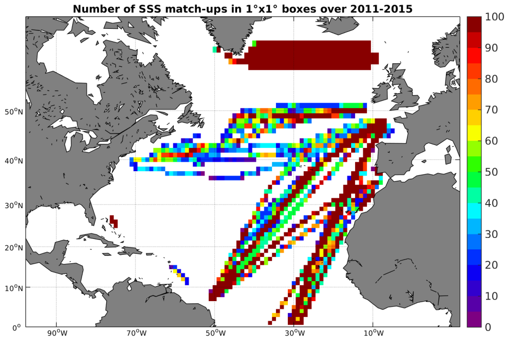
Figure 4: Number of SSS match-ups between TSG-LEGOS-DM SSS and the Aquarius-L4-IPRC-V4-MONTHLY SSS product for the North Atlantic Ocean Pi-MEP region over 1^\circ \times 1^\circ boxes and for the full satellite product period.
