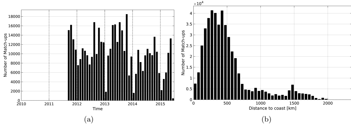
Figure 1: Number of match-ups between TSG-LEGOS-DM and Aquarius-L4-IPRC-V4-MONTHLY SSS as a function of time (a) and as function of the distance to coast (b) over the North Atlantic Ocean Pi-MEP region and for the full satellite product period.
