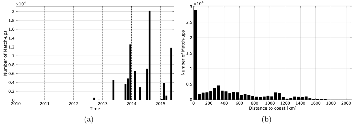
Figure 1: Number of match-ups between TSG-GOSUD-Sailing-ship and Aquarius-L4-IPRC-V4-MONTHLY SSS as a function of time (a) and as function of the distance to coast (b) over the North Atlantic Ocean Pi-MEP region and for the full satellite product period.
