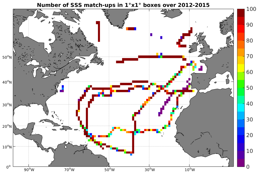
Figure 4: Number of SSS match-ups between TSG-GOSUD-Sailing-ship SSS and the Aquarius-L4-IPRC-V4-MONTHLY SSS product for the North Atlantic Ocean Pi-MEP region over 1^\circ \times 1^\circ boxes and for the full satellite product period.
