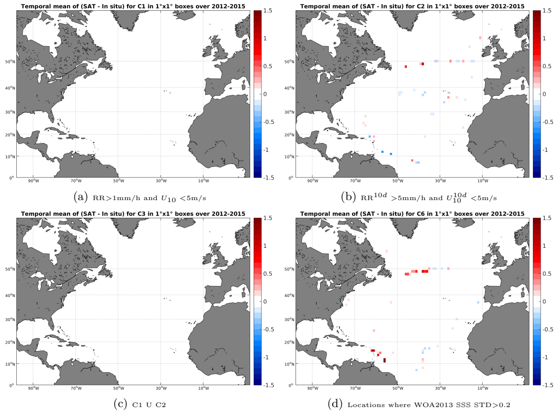
Figure 12: Temporal mean gridded over spatial boxes of size 1^\circ \times 1^\circ of \Delta SSS (Aquarius-L4-IPRC-V4-MONTHLY - TSG-GOSUD-Sailing-ship) for 4 different subdatasets corresponding to: RR > 1mm/h and U_{10} < 5\text{m/s} (a), RR^{10d} > 5\text{mm/h} and U_{10}^{10d} < 5\text{m/s} (b), C1 U C2 (c), Locations where WOA2013 SSS STD > 0.2 (d).
