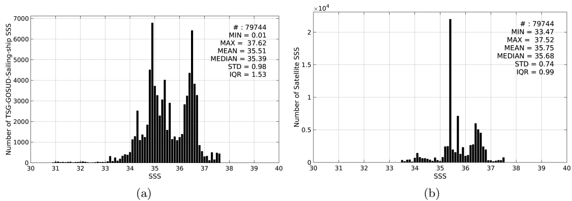
Figure 2: Histograms of SSS from TSG-GOSUD-Sailing-ship (a) and Aquarius-L4-IPRC-V4-MONTHLY (b) considering all match-up pairs per bins of 0.1 over the North Atlantic Ocean Pi-MEP region and for the full satellite product period.
