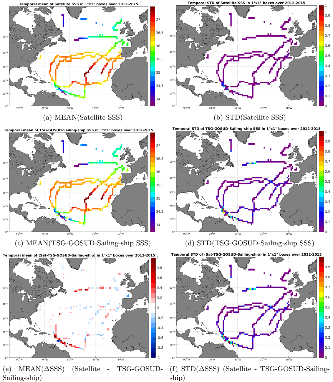
Figure 6: Temporal mean (left) and STD (right) of SSS from Aquarius-L4-IPRC-V4-MONTHLY (top), TSG-GOSUD-Sailing-ship (middle), and of \Delta SSS (Satellite - TSG-GOSUD-Sailing-ship). Only match-up pairs are used to generate these maps.
