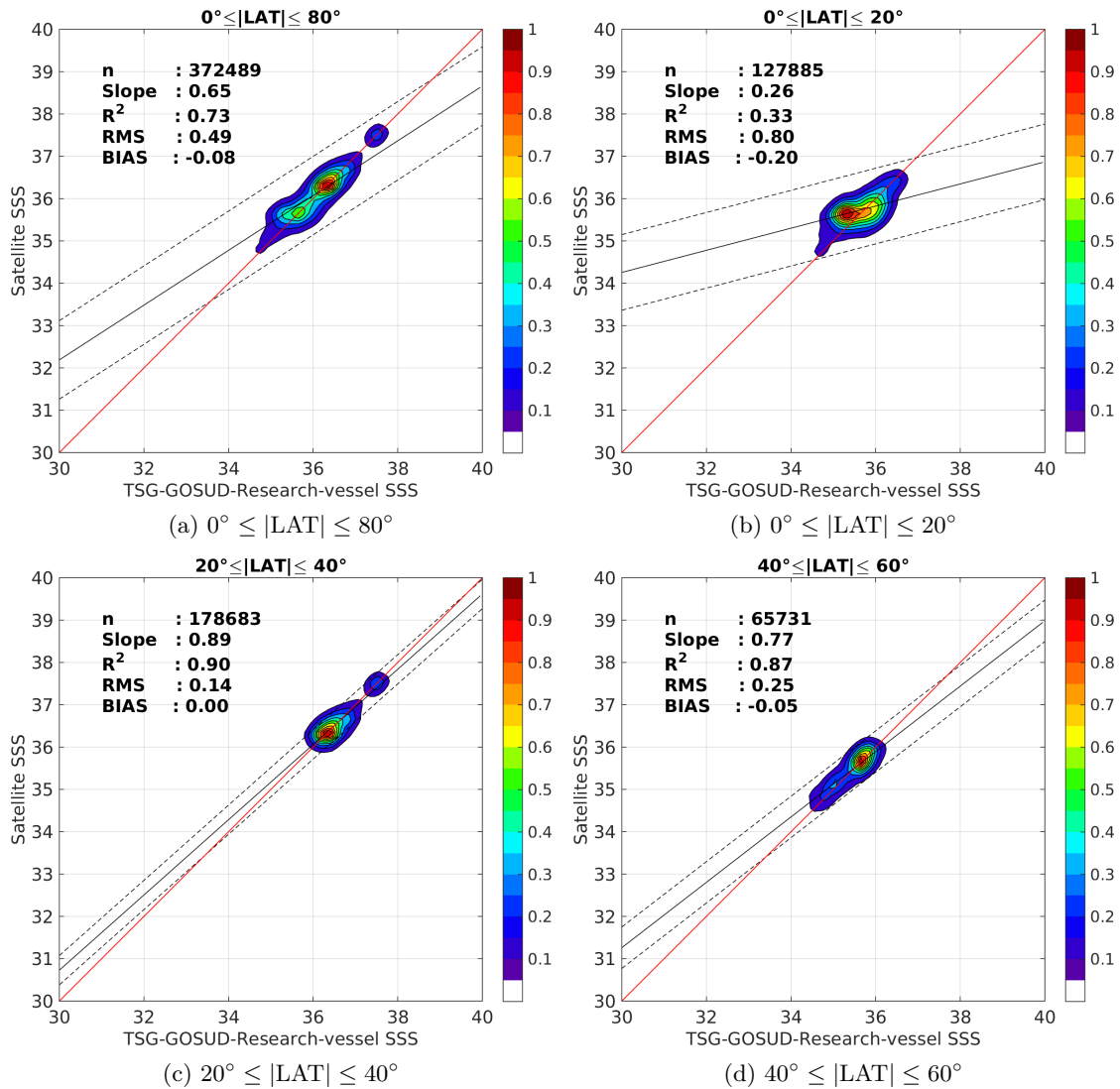
Figure 9: Contour maps of the concentration of Aquarius-L4-IPRC-V4-MONTHLY SSS (y-axis) versus TSG-GOSUD-Research-vessel SSS (x-axis) at match-up pairs for different latitude bands. For each plot, the red line shows x=y . The black thin and dashed lines indicate a linear fit through the data cloud and the \pm 95\% confidence levels, respectively. The number match-up pairs n , the slope and R^2 coefficient of the linear fit, the root mean square (RMS) and the mean bias between satellite and in situ data are indicated for each latitude band in each plots.
