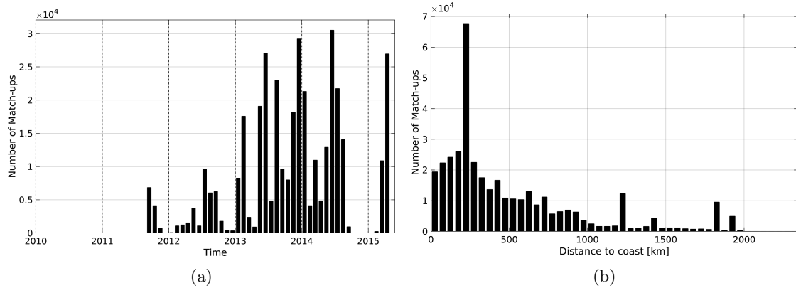
Figure 1: Number of match-ups between TSG-GOSUD-Research-vessel and Aquarius-L4-IPRC-V4-MONTHLY SSS as a function of time (a) and as function of the distance to coast (b) over the North Atlantic Ocean Pi-MEP region and for the full satellite product period.
