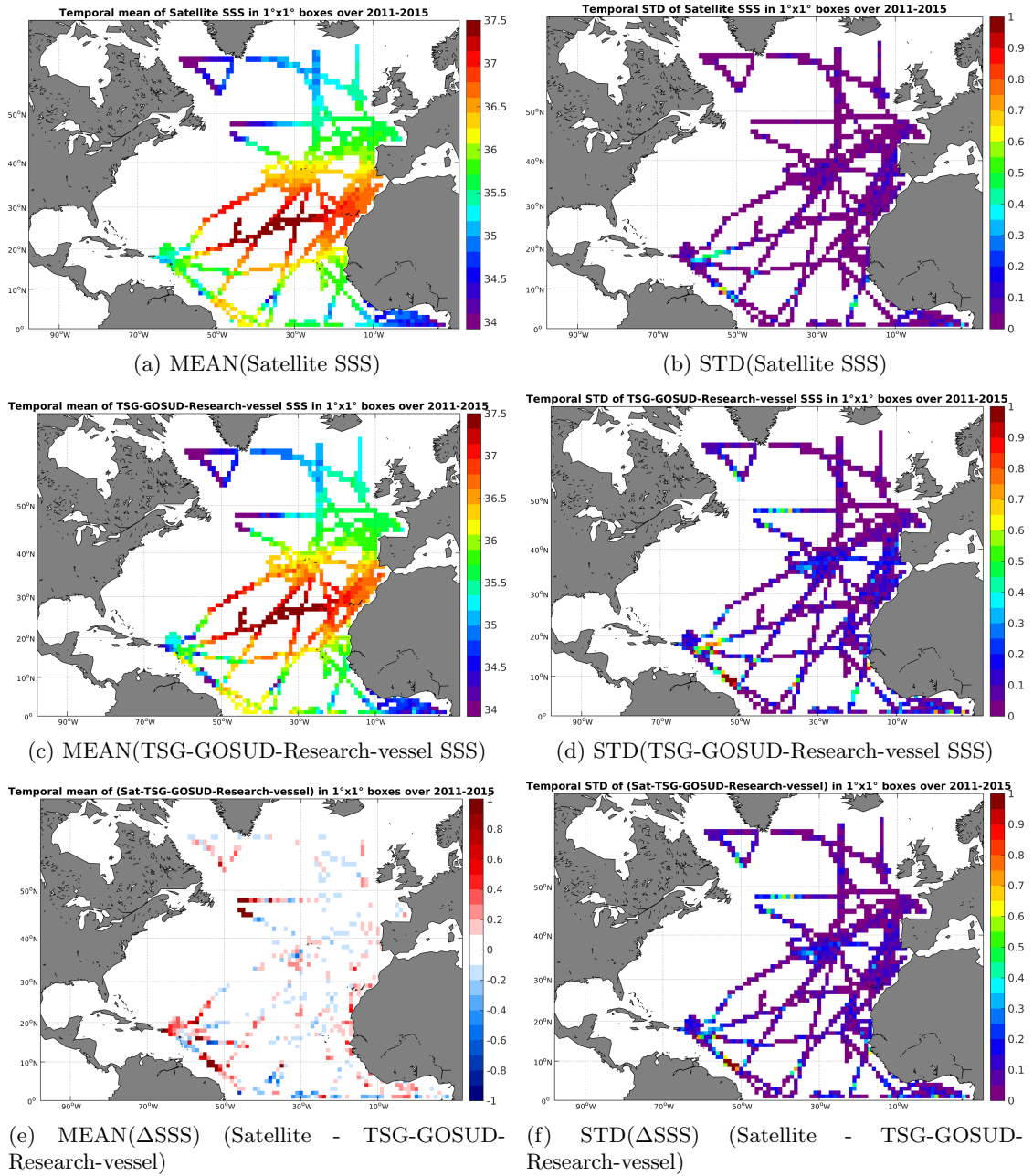
Figure 6: Temporal mean (left) and STD (right) of SSS from Aquarius-L4-IPRC-V4-MONTHLY (top), TSG-GOSUD-Research-vessel (middle), and of \Delta SSS (Satellite - TSG-GOSUD-Research-vessel). Only match-up pairs are used to generate these maps.
