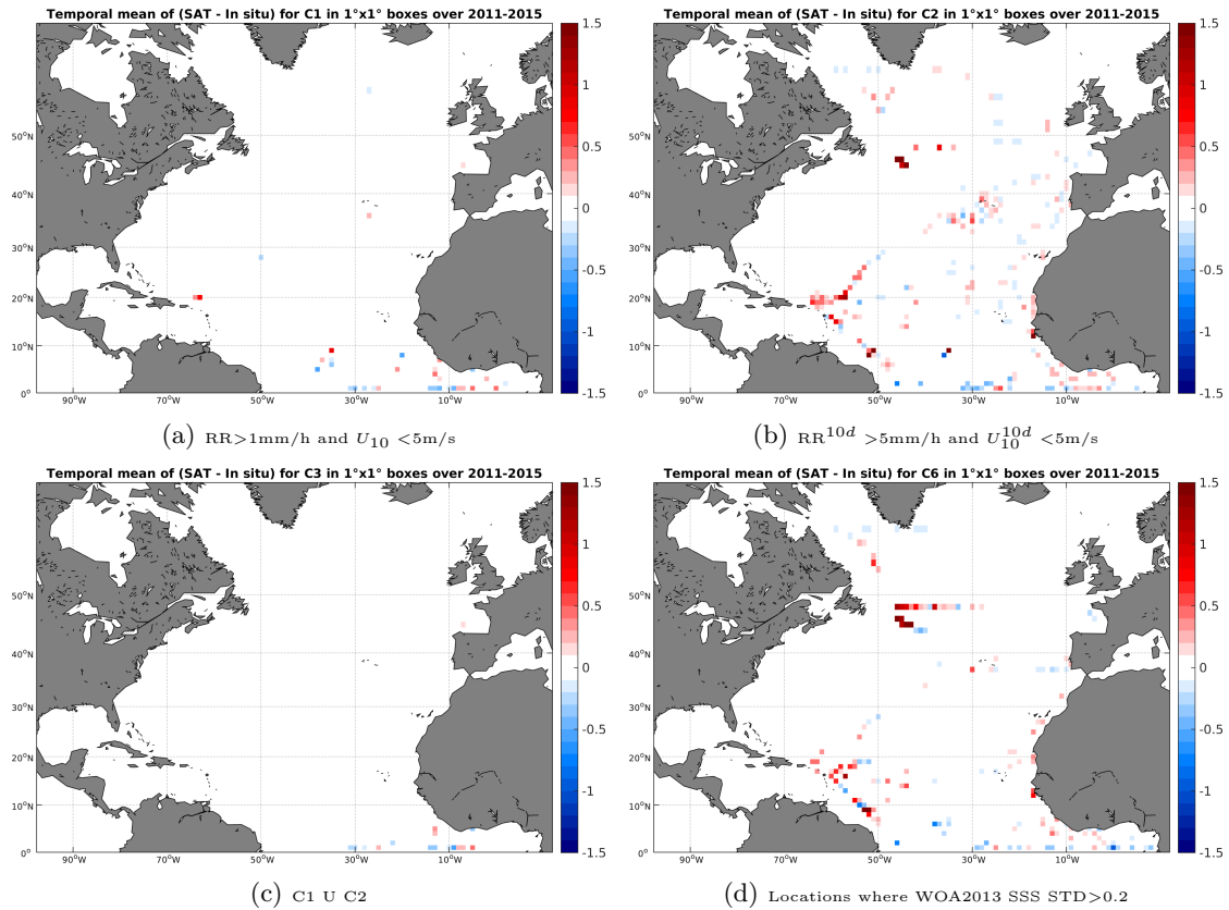
Figure 12: Temporal mean gridded over spatial boxes of size 1^\circ \times 1^\circ of \Delta SSS (Aquarius-L4-IPRC-V4-MONTHLY - TSG-GOSUD-Research-vessel) for 4 different subdatasets corresponding to: RR > 1\text{mm/h} and U_{10} < 5\text{m/s} (a), RR^{10d} > 5\text{mm/h} and U_{10}^{10d} < 5\text{m/s} (b), C1 U C2 (c), Locations where WOA2013 SSS STD > 0.2 (d).
