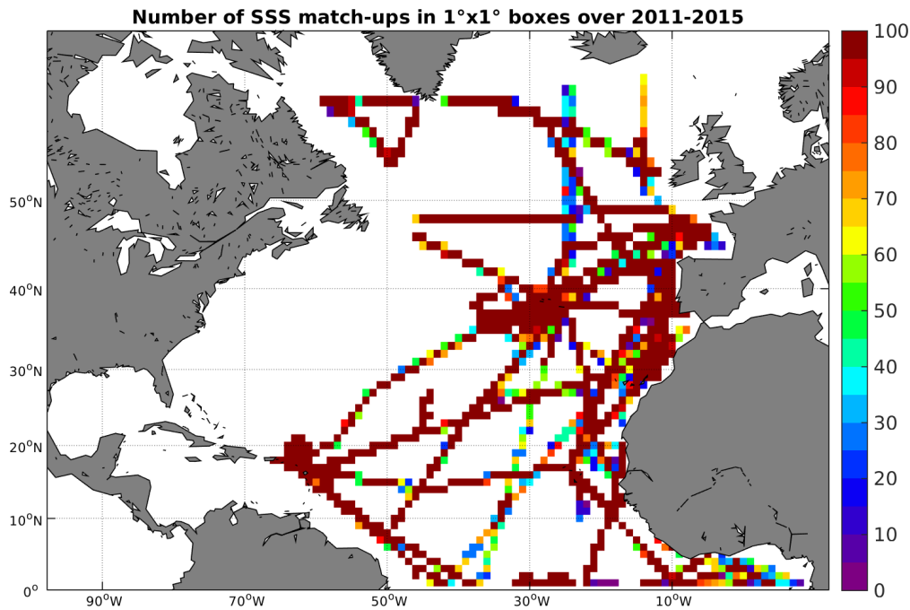
Figure 4: Number of SSS match-ups between TSG-GOSUD-Research-vessel SSS and the Aquarius-L4-IPRC-V4-MONTHLY SSS product for the North Atlantic Ocean Pi-MEP region over 1^\circ \times 1^\circ boxes and for the full satellite product period.
