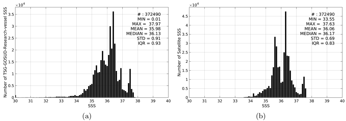
Figure 2: Histograms of SSS from TSG-GOSUD-Research-vessel (a) and Aquarius-L4-IPRC-V4-MONTHLY (b) considering all match-up pairs per bins of 0.1 over the North Atlantic Ocean Pi-MEP region and for the full satellite product period.
