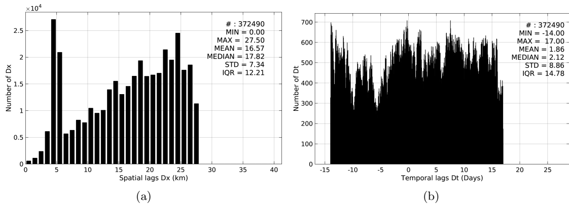
Figure 5: Histograms of the spatial (a) and temporal (b) lags between the time of the TSG-GOSUD-Research-vessel measurements and the date of the corresponding Aquarius-L4-IPRC-V4-MONTHLY SSS product.
