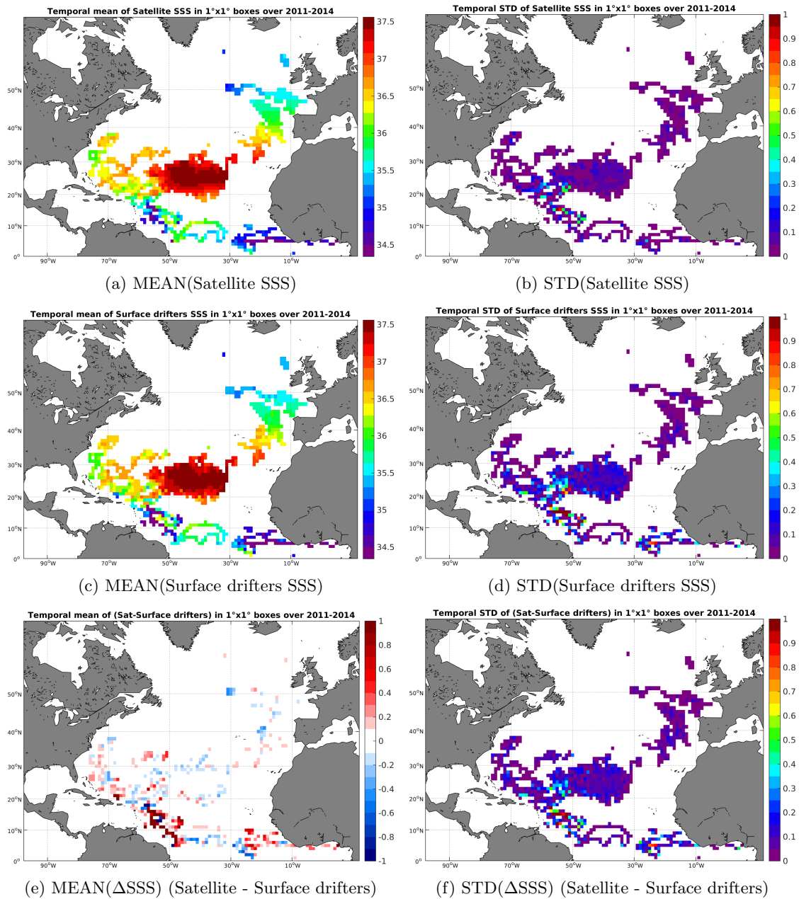
Figure 5: Temporal mean (left) and STD (right) of SSS from Aquarius-L4-IPRC-V4-MONTHLY (top), Surface drifters (middle), and of \Delta SSS (Satellite - Surface drifters). Only match-up pairs are used to generate these maps.
