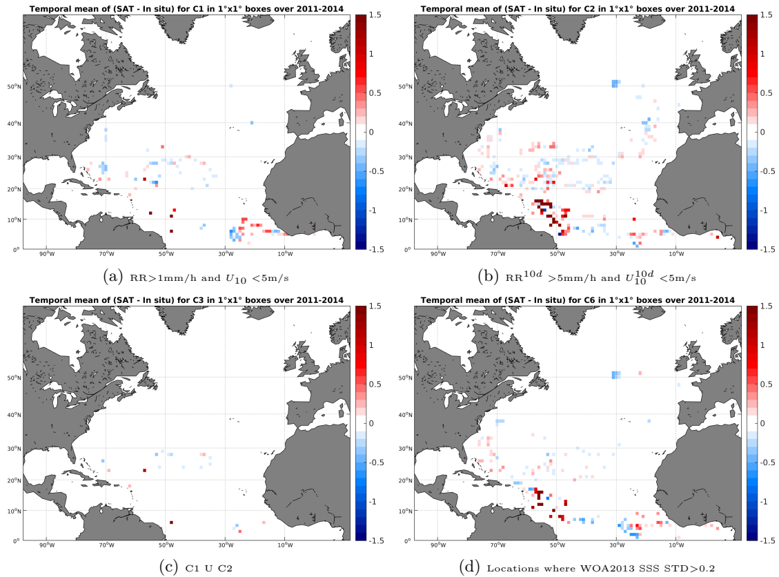
Figure 11: Temporal mean gridded over spatial boxes of size 1^\circ \times 1^\circ of \Delta SSS (Aquarius-L4-IPRC-V4-MONTHLY - Surface drifters) for 4 different subdatasets corresponding to: RR > 1mm/h and U_{10} < 5 m/s (a), RR^{10d} > 5 mm/h and U_{10}^{10d} < 5 m/s (b), C1 U C2 (c), Locations where WOA2013 SSS STD > 0.2 (d).
