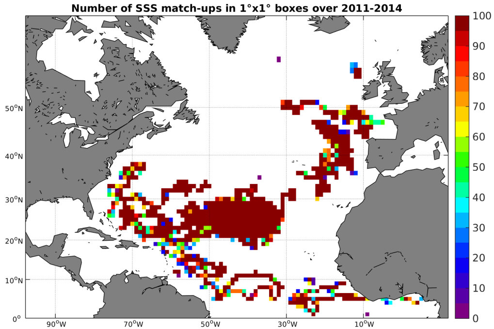
Figure 3: Number of SSS match-ups between Surface drifters SSS and the Aquarius-L4-IPRC-V4-MONTHLY SSS product for the North Atlantic Ocean Pi-MEP region over 1^\circ \times 1^\circ boxes and for the full satellite product period.
