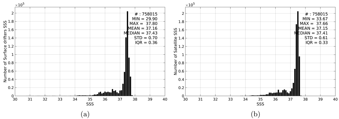
Figure 2: Histograms of SSS from Surface drifters (a) and Aquarius-L4-IPRC-V4-MONTHLY (b) considering all match-up pairs per bins of 0.1 over the North Atlantic Ocean Pi-MEP region and for the full satellite product period.
