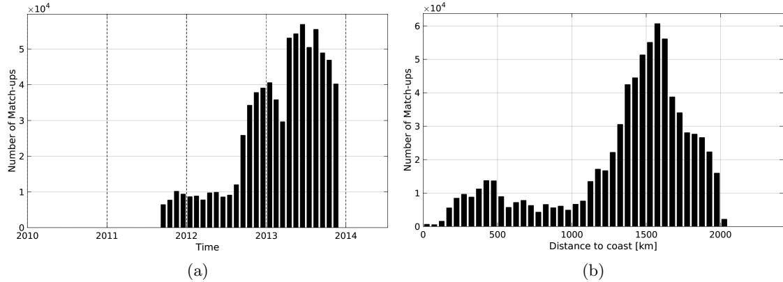
Figure 1: Number of match-ups between Surface drifters and Aquarius-L4-IPRC-V4-MONTHLY SSS as a function of time (a) and as function of the distance to coast (b) over the North Atlantic Ocean Pi-MEP region and for the full satellite product period.
