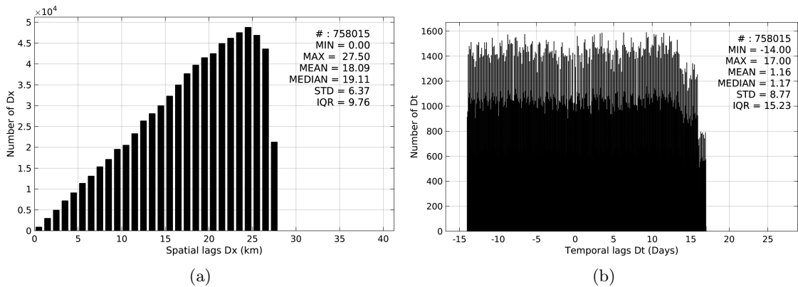
Figure 4: Histograms of the spatial (a) and temporal (b) lags between the time of the Surface drifters measurements and the date of the corresponding Aquarius-L4-IPRC-V4-MONTHLY SSS product.
