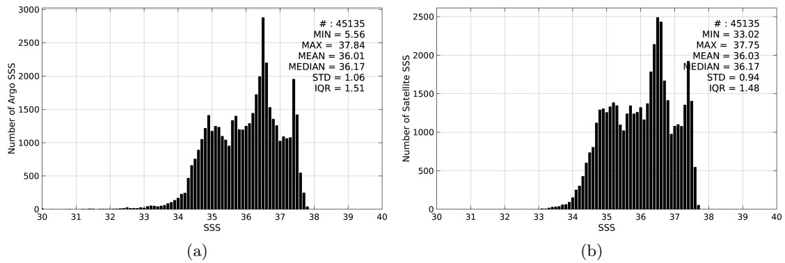
Figure 2: Histograms of SSS from Argo (a) and Aquarius-L4-IPRC-V4-MONTHLY (b) considering all match-up pairs per bins of 0.1 over the North Atlantic Ocean Pi-MEP region and for the full satellite product period.
