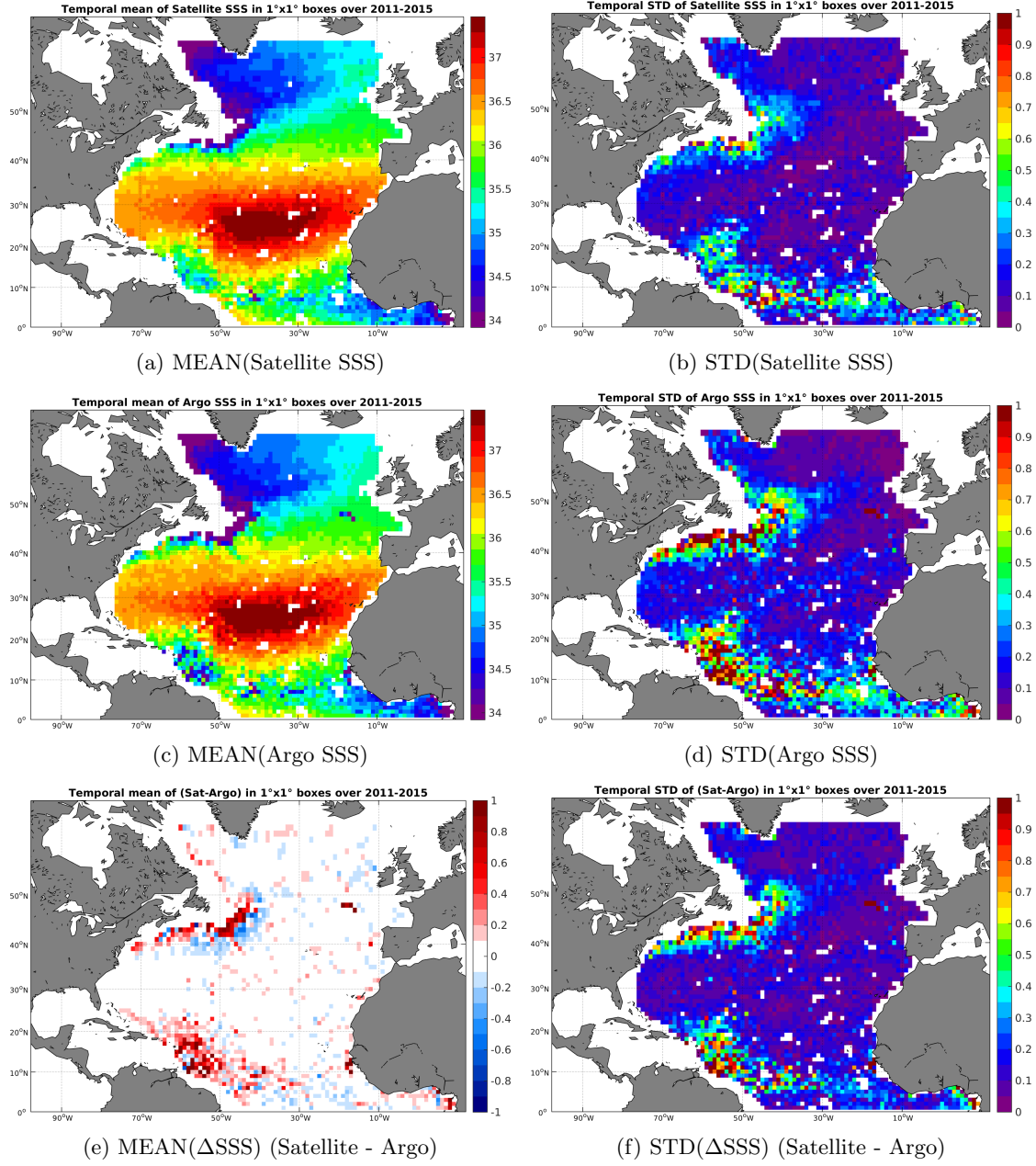
Figure 6: Temporal mean (left) and STD (right) of SSS from Aquarius-L4-IPRC-V4-MONTHLY (top), Argo (middle), and of \Delta SSS (Satellite - Argo). Only match-up pairs are used to generate these maps.
