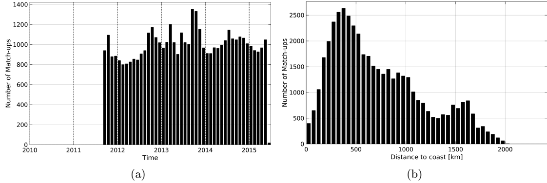
Figure 1: Number of match-ups between Argo and Aquarius-L4-IPRC-V4-MONTHLY SSS as a function of time (a) and as function of the distance to coast (b) over the North Atlantic Ocean Pi-MEP region and for the full satellite product period.
