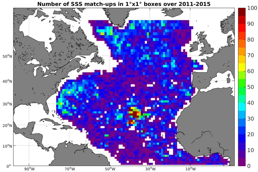
Figure 4: Number of SSS match-ups between Argo SSS and the Aquarius-L4-IPRC-V4-MONTHLY SSS product for the North Atlantic Ocean Pi-MEP region over 1^\circ \times 1^\circ boxes and for the full satellite product period.
