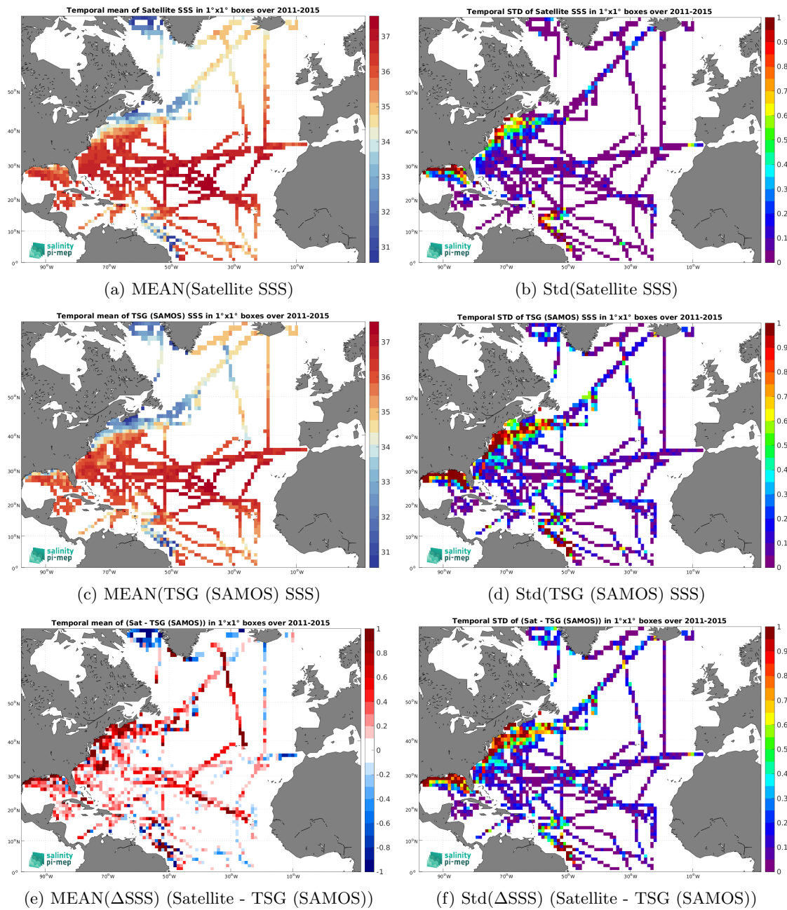
Figure 6: Temporal mean (left) and Std (right) of SSS from Aquarius SSS L3 OR v5 - 7-Day running (NASA-GSFC) (top), TSG (SAMOS) (middle), and of \Delta SSS (Satellite - TSG (SAMOS)). Only match-up pairs are used to generate these maps.
