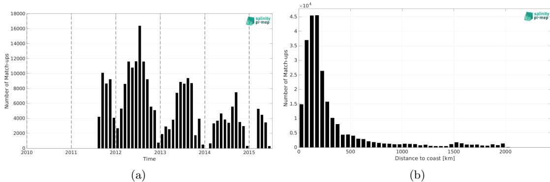
Figure 1: Number of match-ups between TSG (SAMOS) and Aquarius SSS L3 OR v5 - 7-Day running (NASA-GSFC) SSS as a function of time (a) and as function of the distance to coast (b) over the North Atlantic Ocean Pi-MEP region and for the full satellite product period.
