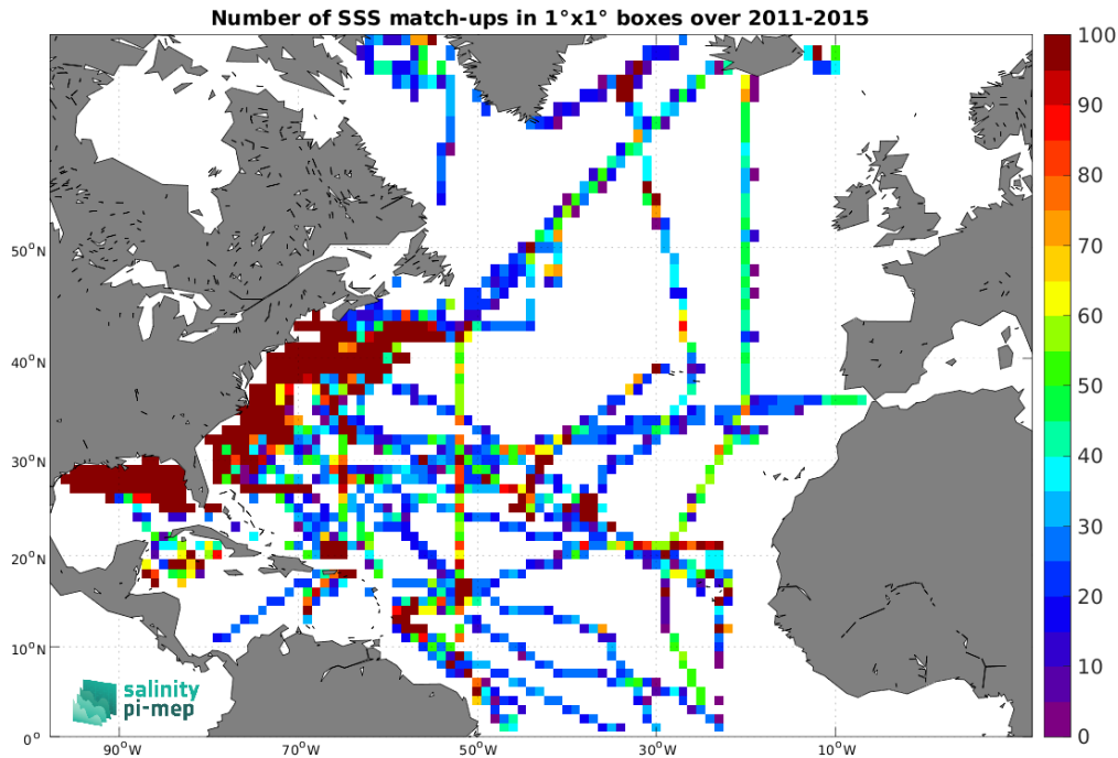
Figure 4: Number of SSS match-ups between TSG (SAMOS) SSS and the Aquarius SSS L3 OR v5 - 7-Day running (NASA-GSFC) SSS product for the North Atlantic Ocean Pi-MEP region over 1^\circ \times 1^\circ boxes and for the full satellite product period.
