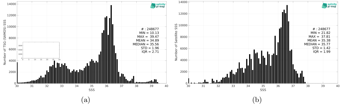
Figure 2: Histograms of SSS from TSG (SAMOS) (a) and Aquarius SSS L3 OR v5 - 7-Day running (NASA-GSFC) (b) considering all match-up pairs per bins of 0.1 over the North Atlantic Ocean Pi-MEP region and for the full satellite product period.
