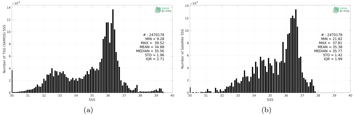
Figure 2: Histograms of SSS from TSG (SAMOS) (a) and Aquarius SSS L3 OR v5 - 7-Day running (NASA-GSFC) (b) considering all match-up pairs per bins of 0.1 over the North Atlantic Ocean Pi-MEP region and for the full satellite product period.
