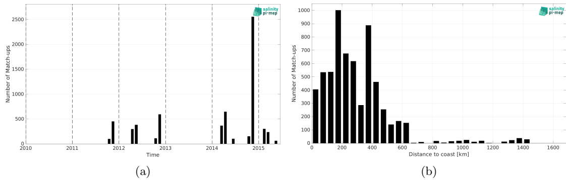
Figure 2: Number of match-ups between TSG (Polarstern) and Aquarius SSS L3 OR v5 - 7-Day running (NASA-GSFC) SSS as a function of time (a) and as function of the distance to coast (b) over the North Atlantic Ocean Pi-MEP region and for the full satellite product period.
