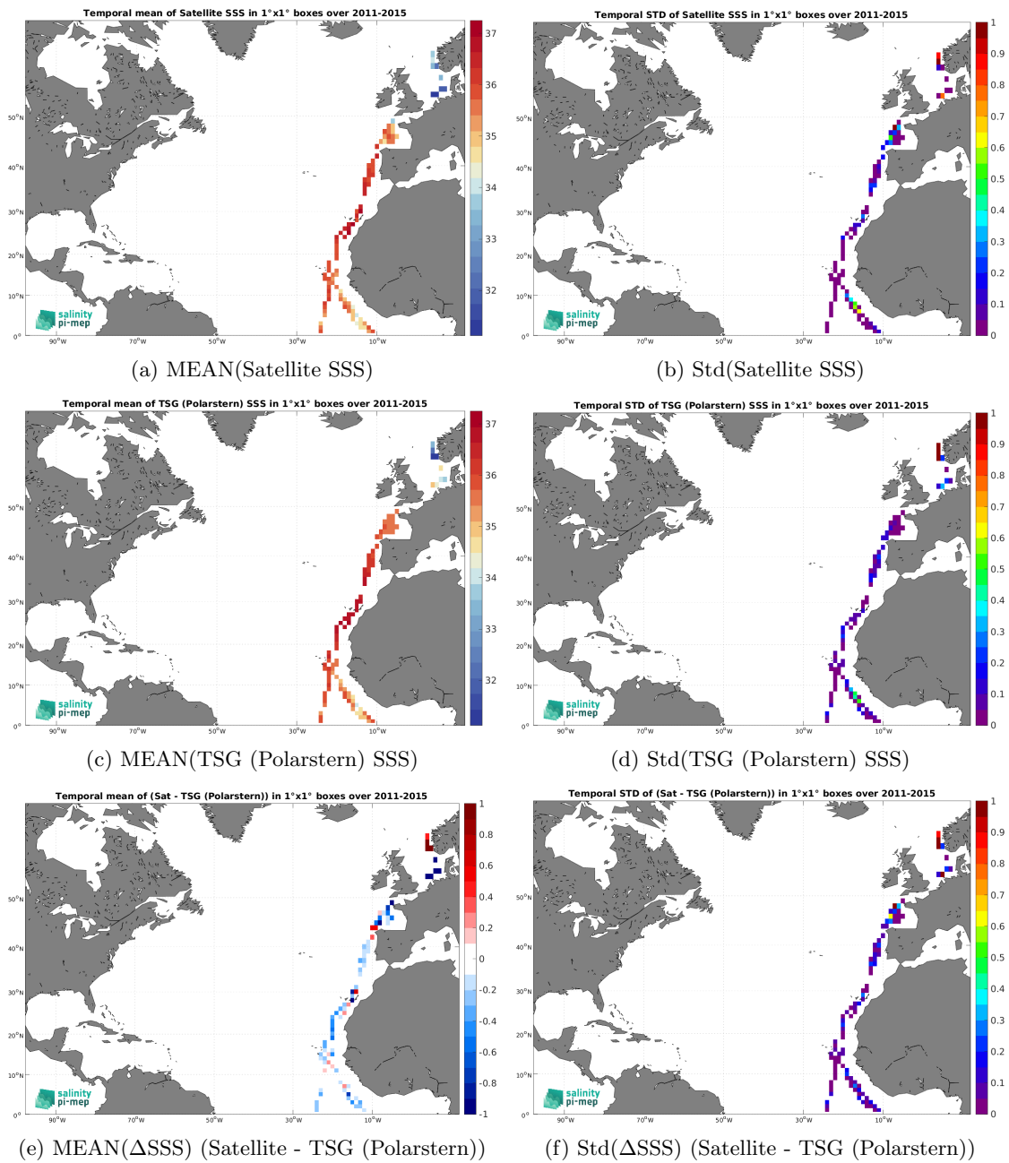
Figure 7: Temporal mean (left) and Std (right) of SSS from Aquarius SSS L3 OR v5 - 7-Day running (NASA-GSFC) (top), TSG (Polarstern) (middle), and of \Delta SSS (Satellite - TSG (Polarstern)). Only match-up pairs are used to generate these maps.
