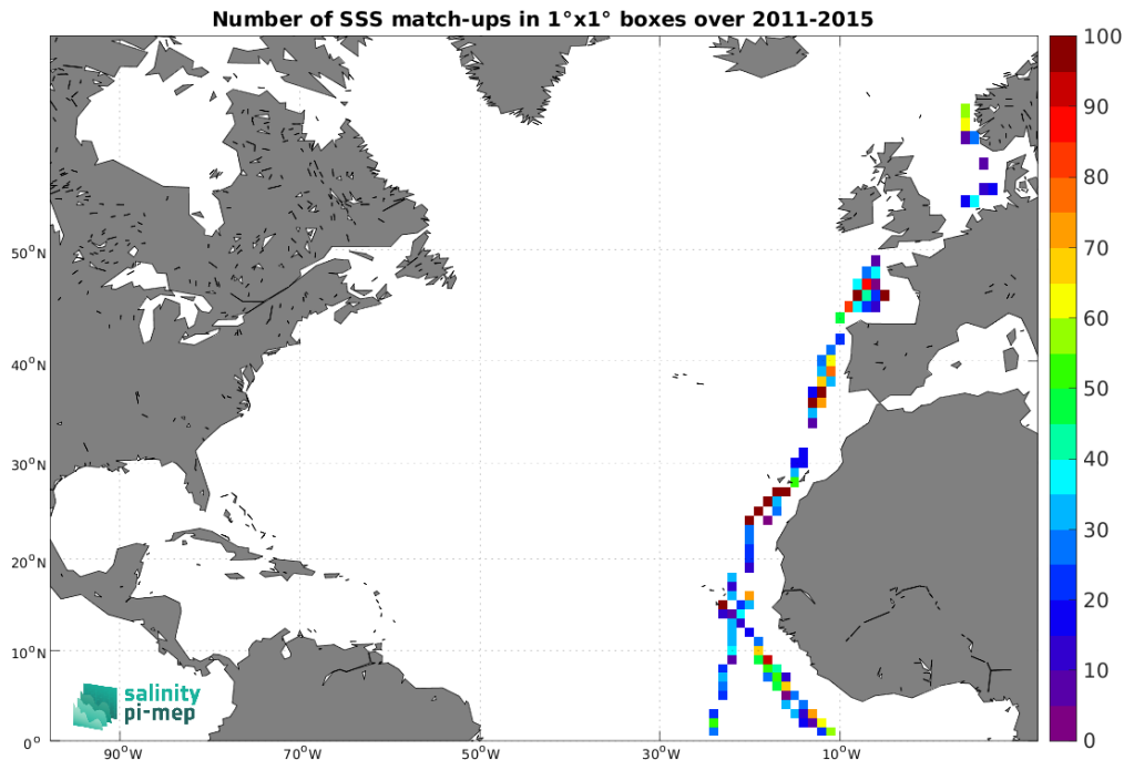
Figure 5: Number of SSS match-ups between TSG (Polarstern) SSS and the Aquarius SSS L3 OR v5 - 7-Day running (NASA-GSFC) SSS product for the North Atlantic Ocean Pi-MEP region over 1^\circ \times 1^\circ boxes and for the full satellite product period.
