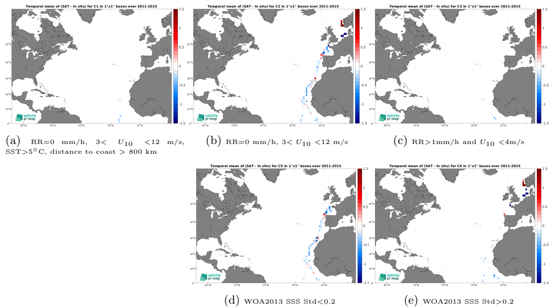
Figure 14: Temporal mean gridded over spatial boxes of size 1^\circ \times 1^\circ of \Delta\text{SSS} (Aquarius SSS L3 OR v5 - 7-Day running (NASA-GSFC) - TSG (Polarstern)) for 5 different subdatasets corresponding to:RR=0 mm/h, 3 < U_{10} < 12 m/s, SST >5^\circ\text{C} , distance to coast > 800 km (a), RR=0 mm/h, 3 < U_{10} < 12 m/s (b), RR >1 mm/h and U_{10} < 4 m/s (c), WOA2013 SSS Std <0.2 (d), WOA2013 SSS Std >0.2 (e).
