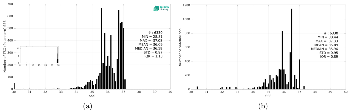
Figure 3: Histograms of SSS from TSG (Polarstern) (a) and Aquarius SSS L3 OR v5 - 7-Day running (NASA-GSFC) (b) considering all match-up pairs per bins of 0.1 over the North Atlantic Ocean Pi-MEP region and for the full satellite product period.
