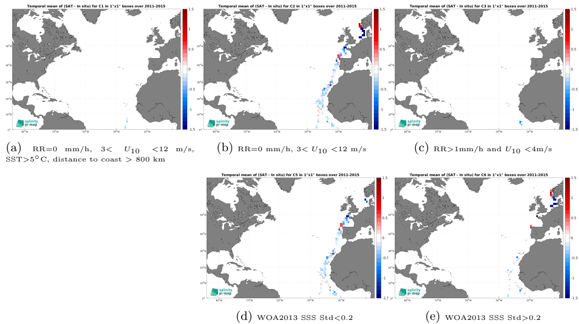
Figure 12: Temporal mean gridded over spatial boxes of size 1^\circ \times 1^\circ of \Delta\text{SSS} (Aquarius SSS L3 OR v5 - 7-Day running (NASA-GSFC) - TSG (Polarstern)) for 5 different subdatasets corresponding to:RR=0 mm/h, 3 < U_{10} < 12 m/s, SST >5^\circ\text{C} , distance to coast > 800 km (a), RR=0 mm/h, 3 < U_{10} < 12 m/s (b), RR >1 mm/h and U_{10} < 4 m/s (c), WOA2013 SSS Std <0.2 (d), WOA2013 SSS Std >0.2 (e).
