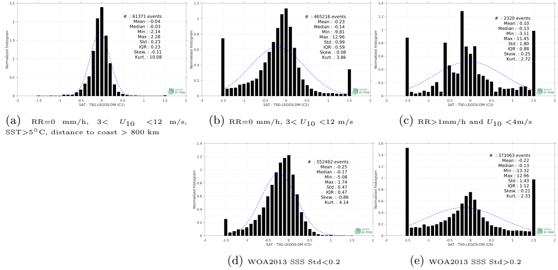
Figure 13: Normalized histogram of \Delta SSS (Aquarius-L3-OR-V5-7DAY-RUNNING-1DEG - TSG-LEGOS-DM) for 5 different subdatasets corresponding to: RR=0 mm/h, 3 < U_{10} < 12 m/s, SST>5°C, distance to coast > 800 km (a), RR=0 mm/h, 3 < U_{10} < 12 m/s (b), RR>1mm/h and U_{10} < 4 m/s (c), WOA2013 SSS Std<0.2 (d), WOA2013 SSS Std>0.2 (e).
