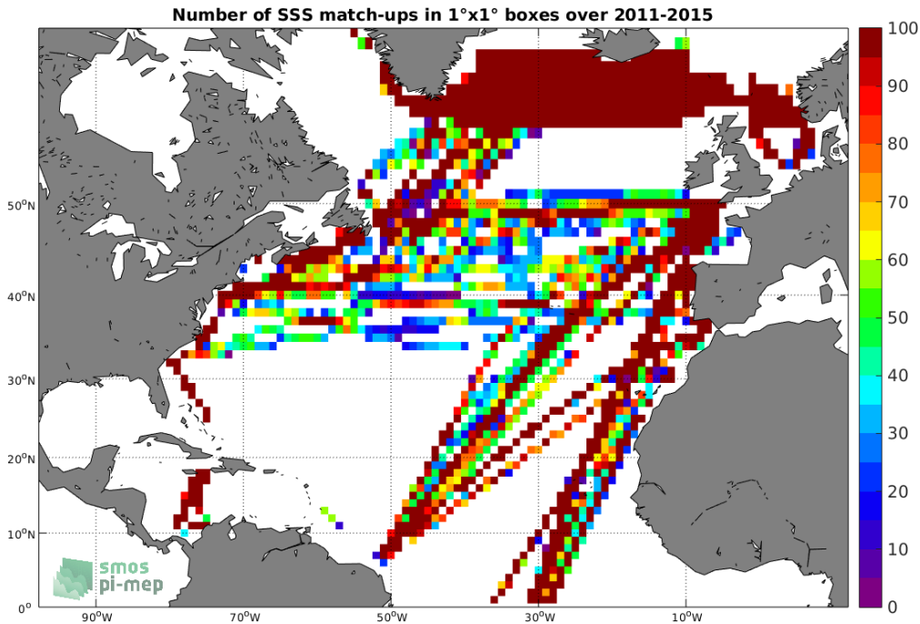
Figure 4: Number of SSS match-ups between TSG-LEGOS-DM SSS and the Aquarius-L3-OR-V5-7DAY-RUNNING-1DEG SSS product for the North Atlantic Ocean Pi-MEP region over 1^\circ \times 1^\circ boxes and for the full satellite product period.
