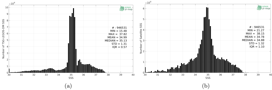
Figure 2: Histograms of SSS from TSG-LEGOS-DM (a) and Aquarius-L3-OR-V5-7DAY-RUNNING-1DEG (b) considering all match-up pairs per bins of 0.1 over the North Atlantic Ocean Pi-MEP region and for the full satellite product period.
