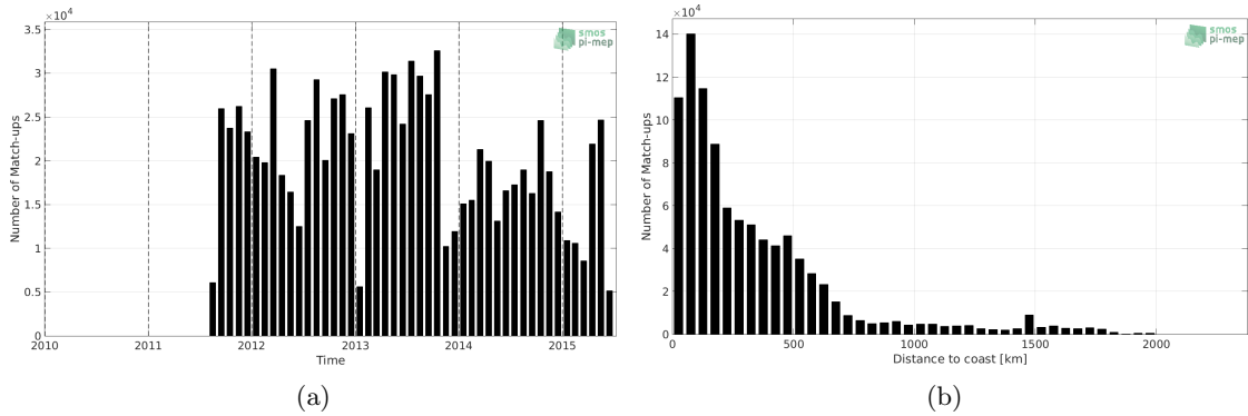
Figure 1: Number of match-ups between TSG-LEGOS-DM and Aquarius-L3-OR-V5-7DAY-RUNNING-1DEG SSS as a function of time (a) and as function of the distance to coast (b) over the North Atlantic Ocean Pi-MEP region and for the full satellite product period.
