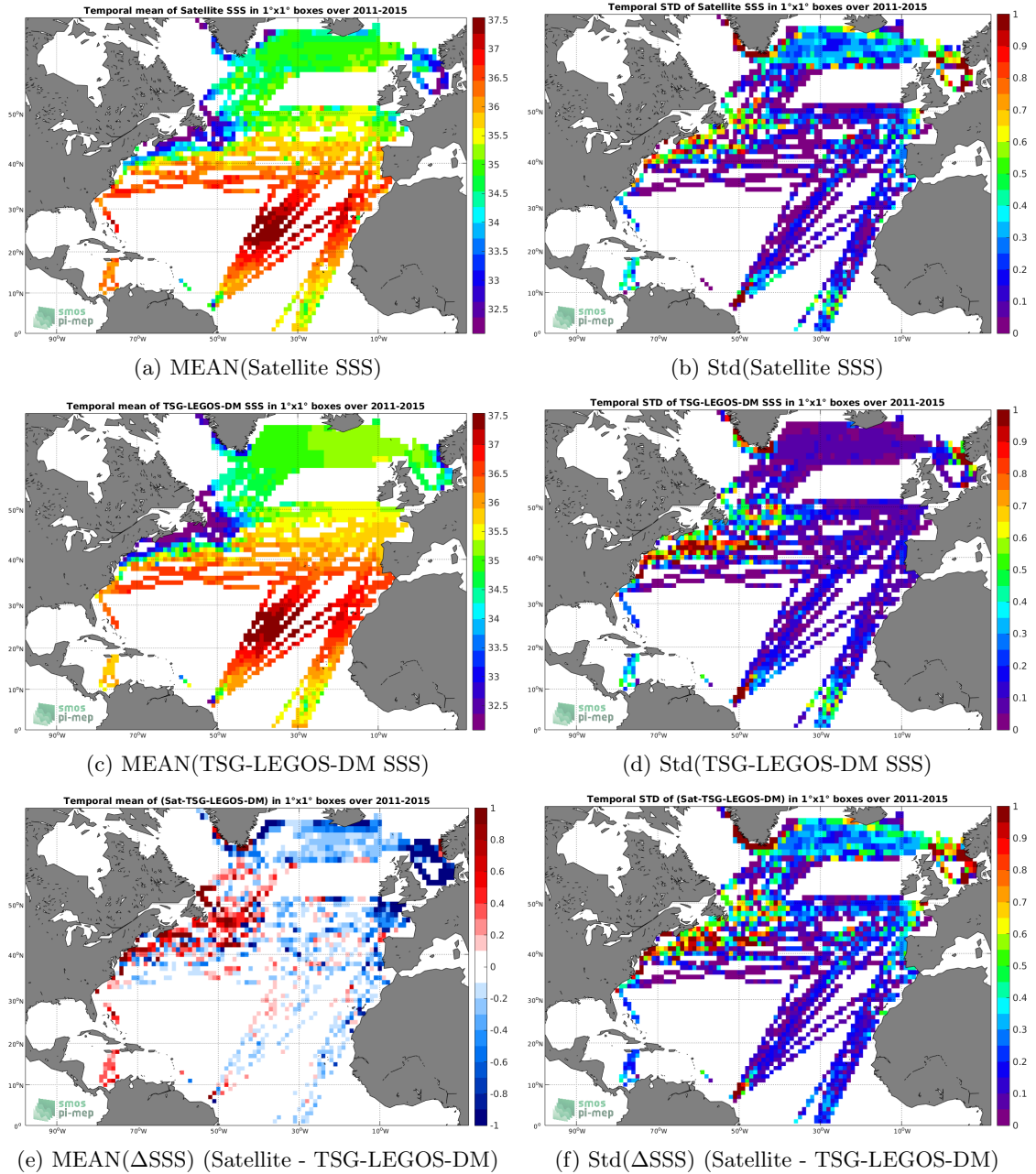
Figure 6: Temporal mean (left) and Std (right) of SSS from Aquarius-L3-OR-V5-7DAY-RUNNING-1DEG (top), TSG-LEGOS-DM (middle), and of \Delta SSS (Satellite - TSG-LEGOS-DM). Only match-up pairs are used to generate these maps.
