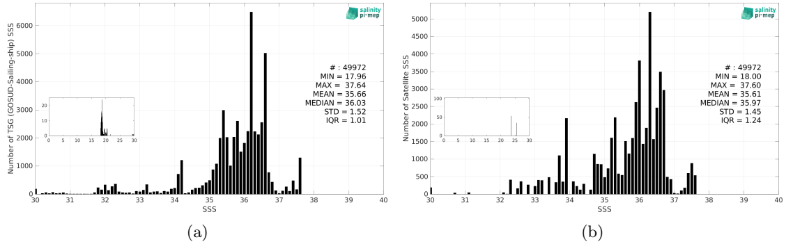
Figure 3: Histograms of SSS from TSG (GOSUD-Sailing-ship) (a) and Aquarius SSS L3 OR v5 - 7-Day running (NASA-GSFC) (b) considering all match-up pairs per bins of 0.1 over the North Atlantic Ocean Pi-MEP region and for the full satellite product period.
