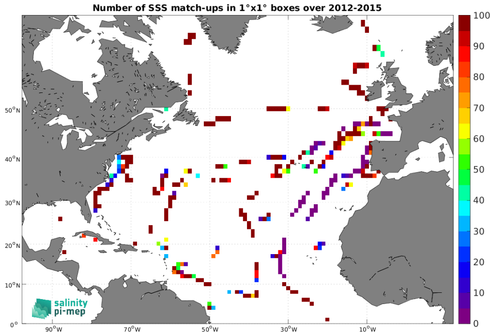
Figure 5: Number of SSS match-ups between TSG (GOSUD-Sailing-ship) SSS and the Aquarius SSS L3 OR v5 - 7-Day running (NASA-GSFC) SSS product for the North Atlantic Ocean Pi-MEP region over 1^\circ \times 1^\circ boxes and for the full satellite product period.
