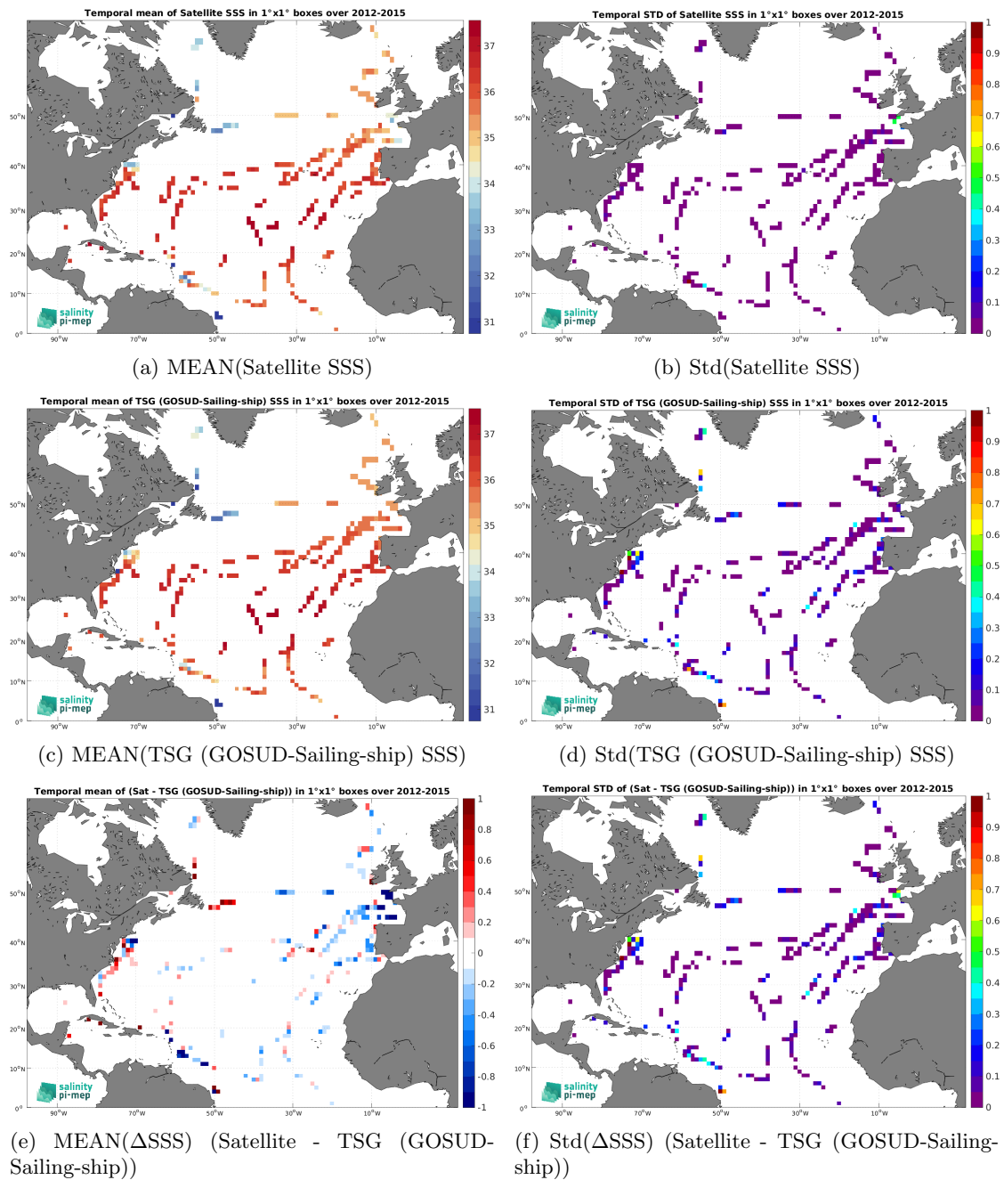
Figure 7: Temporal mean (left) and Std (right) of SSS from Aquarius SSS L3 OR v5 - 7-Day running (NASA-GSFC) (top), TSG (GOSUD-Sailing-ship) (middle), and of \Delta SSS (Satellite - TSG (GOSUD-Sailing-ship)). Only match-up pairs are used to generate these maps.
