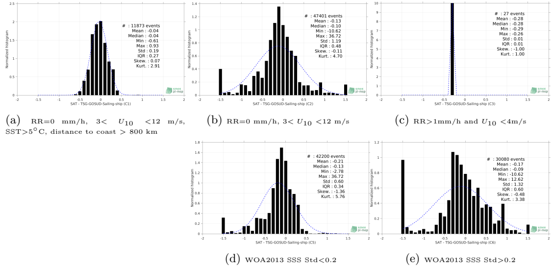
Figure 13: Normalized histogram of \Delta SSS (Aquarius-L3-OR-V5-7DAY-RUNNING-1DEG - TSG-GOSUD-Sailing-ship) for 5 different subdatasets corresponding to: RR=0 mm/h, 3 < U_{10} < 12 m/s, SST>5°C, distance to coast > 800 km (a), RR=0 mm/h, 3 < U_{10} < 12 m/s (b), RR>1mm/h and U_{10} < 4 m/s (c), WOA2013 SSS Std<0.2 (d), WOA2013 SSS Std>0.2 (e).
