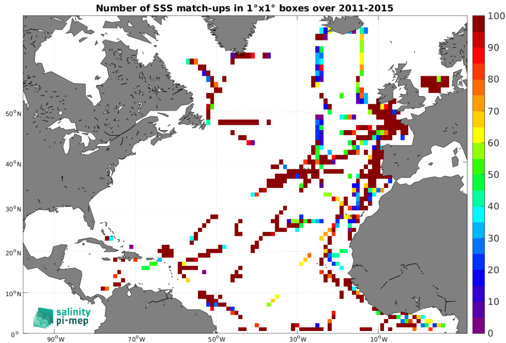
Figure 5: Number of SSS match-ups between TSG (GOSUD-Research-vessel) SSS and the Aquarius SSS L3 OR v5 - 7-Day running (NASA-GSFC) SSS product for the North Atlantic Ocean Pi-MEP region over 1^\circ \times 1^\circ boxes and for the full satellite product period.
