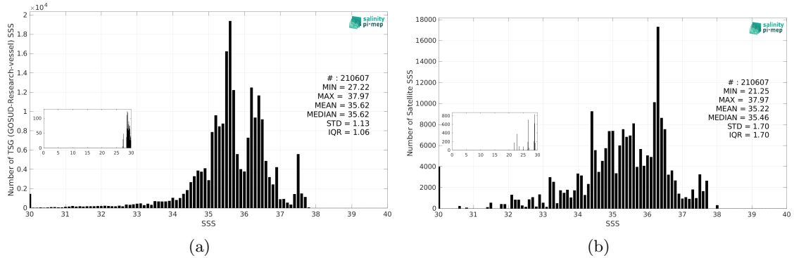
Figure 3: Histograms of SSS from TSG (GOSUD-Research-vessel) (a) and Aquarius SSS L3 OR v5 - 7-Day running (NASA-GSFC) (b) considering all match-up pairs per bins of 0.1 over the North Atlantic Ocean Pi-MEP region and for the full satellite product period.
