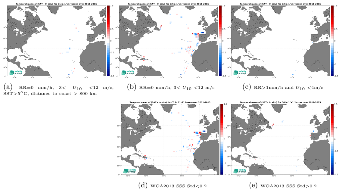
Figure 14: Temporal mean gridded over spatial boxes of size 1^\circ \times 1^\circ of \Delta SSS (Aquarius SSS L3 OR v5 - 7-Day running (NASA-GSFC) - TSG (CSIC-UTM)) for 5 different subdatasets corresponding to:RR=0 mm/h, 3 < U_{10} < 12 m/s, SST >5^\circ\text{C} , distance to coast > 800 km (a), RR=0 mm/h, 3 < U_{10} < 12 m/s (b), RR >1 mm/h and U_{10} < 4 m/s (c), WOA2013 SSS Std <0.2 (d), WOA2013 SSS Std >0.2 (e).
