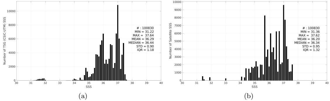
Figure 3: Histograms of SSS from TSG (CSIC-UTM) (a) and Aquarius SSS L3 OR v5 - 7-Day running (NASA-GSFC) (b) considering all match-up pairs per bins of 0.1 over the North Atlantic Ocean Pi-MEP region and for the full satellite product period.
