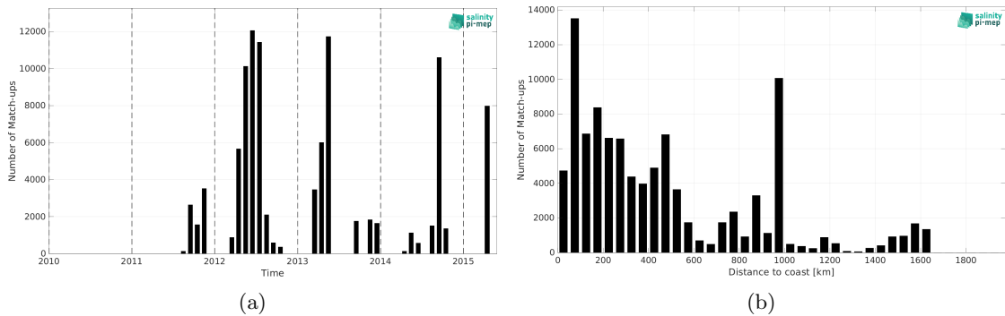
Figure 2: Number of match-ups between TSG (CSIC-UTM) and Aquarius SSS L3 OR v5 - 7-Day running (NASA-GSFC) SSS as a function of time (a) and as function of the distance to coast (b) over the North Atlantic Ocean Pi-MEP region and for the full satellite product period.
