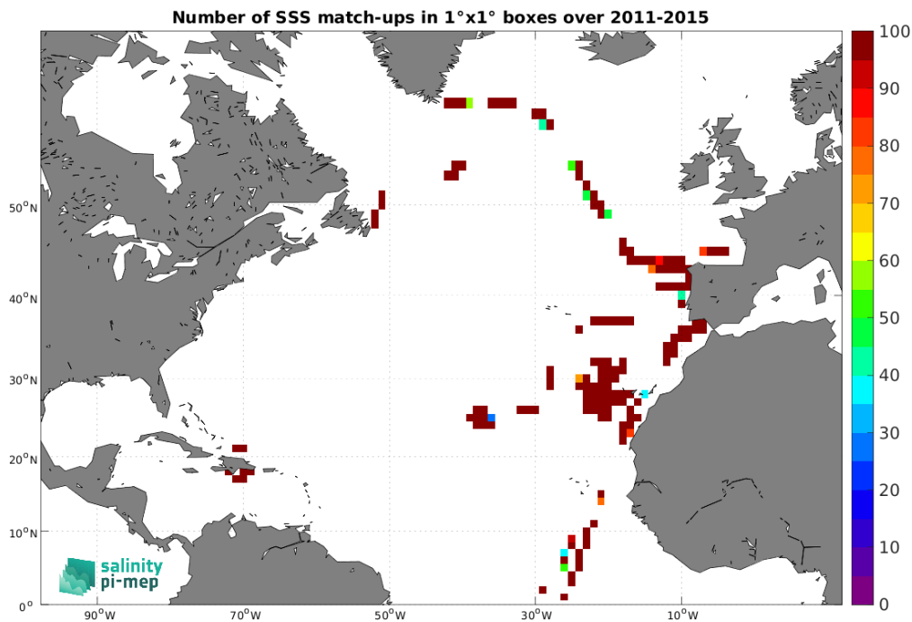
Figure 5: Number of SSS match-ups between TSG (CSIC-UTM) SSS and the Aquarius SSS L3 OR v5 - 7-Day running (NASA-GSFC) SSS product for the North Atlantic Ocean Pi-MEP region over 1^\circ \times 1^\circ boxes and for the full satellite product period.
