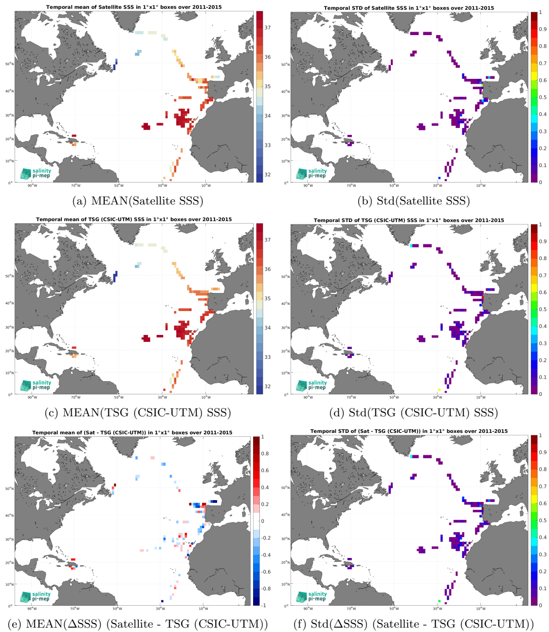
Figure 7: Temporal mean (left) and Std (right) of SSS from Aquarius SSS L3 OR v5 - 7-Day running (NASA-GSFC) (top), TSG (CSIC-UTM) (middle), and of \Delta SSS (Satellite - TSG (CSIC-UTM)). Only match-up pairs are used to generate these maps.
