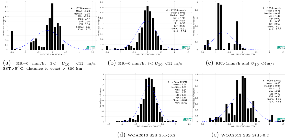
Figure 15: Normalized histogram of \Delta SSS (Aquarius SSS L3 OR v5 - 7-Day running (NASA-GSFC) - TSG (CSIC-UTM)) for 5 different subdatasets corresponding to: RR=0 mm/h, 3 < U_{10} < 12 m/s, SST > 5°C, distance to coast > 800 km (a), RR=0 mm/h, 3 < U_{10} < 12 m/s (b), RR > 1mm/h and U_{10} < 4 m/s (c), WOA2013 SSS Std < 0.2 (d), WOA2013 SSS Std > 0.2 (e).
