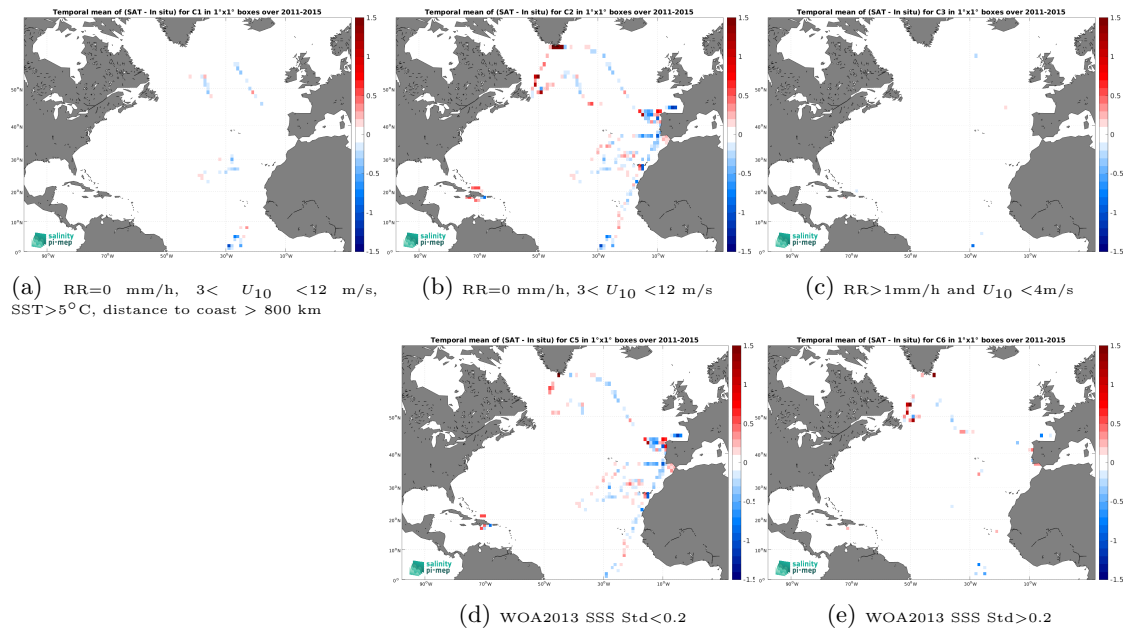
Figure 12: Temporal mean gridded over spatial boxes of size 1^\circ \times 1^\circ of \Delta\text{SSS} (Aquarius SSS L3 OR v5 - 7-Day running (NASA-GSFC) - TSG (CSIC-UTM)) for 5 different subdatasets corresponding to:RR=0 mm/h, 3 < U_{10} < 12 m/s, SST >5^\circ\text{C} , distance to coast > 800 km (a), RR=0 mm/h, 3 < U_{10} < 12 m/s (b), RR >1 mm/h and U_{10} < 4 m/s (c), WOA2013 SSS Std <0.2 (d), WOA2013 SSS Std >0.2 (e).
