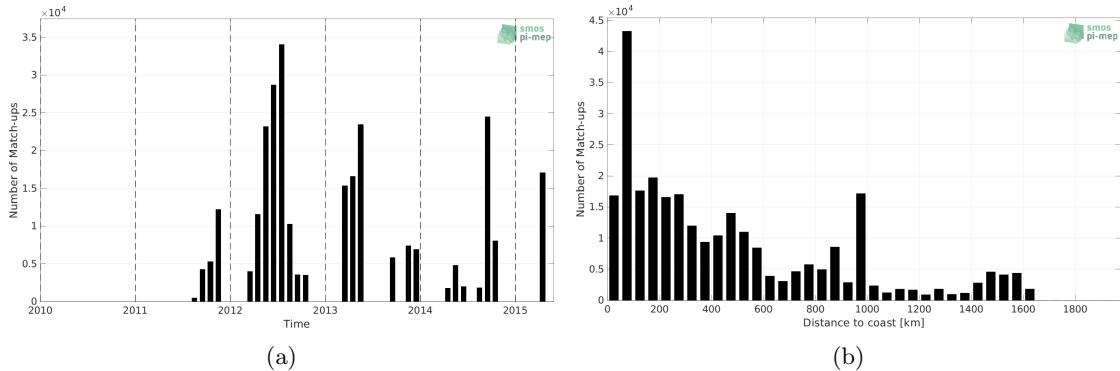
Figure 1: Number of match-ups between TSG (CSIC-UTM) and Aquarius SSS L3 OR v5 - 7-Day running (NASA-GSFC) SSS as a function of time (a) and as function of the distance to coast (b) over the North Atlantic Ocean Pi-MEP region and for the full satellite product period.
