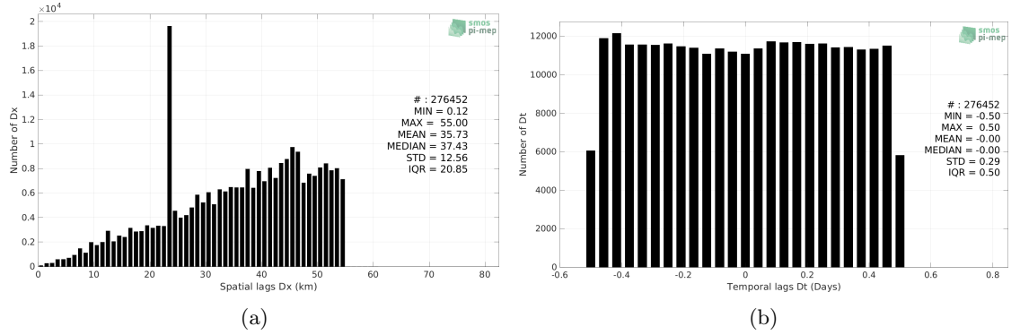
Figure 5: Histograms of the spatial (a) and temporal (b) lags between the location/time of the TSG (CSIC-UTM) measurement and the date of the corresponding Aquarius SSS L3 OR v5 - 7-Day running (NASA-GSFC) SSS pixel.
