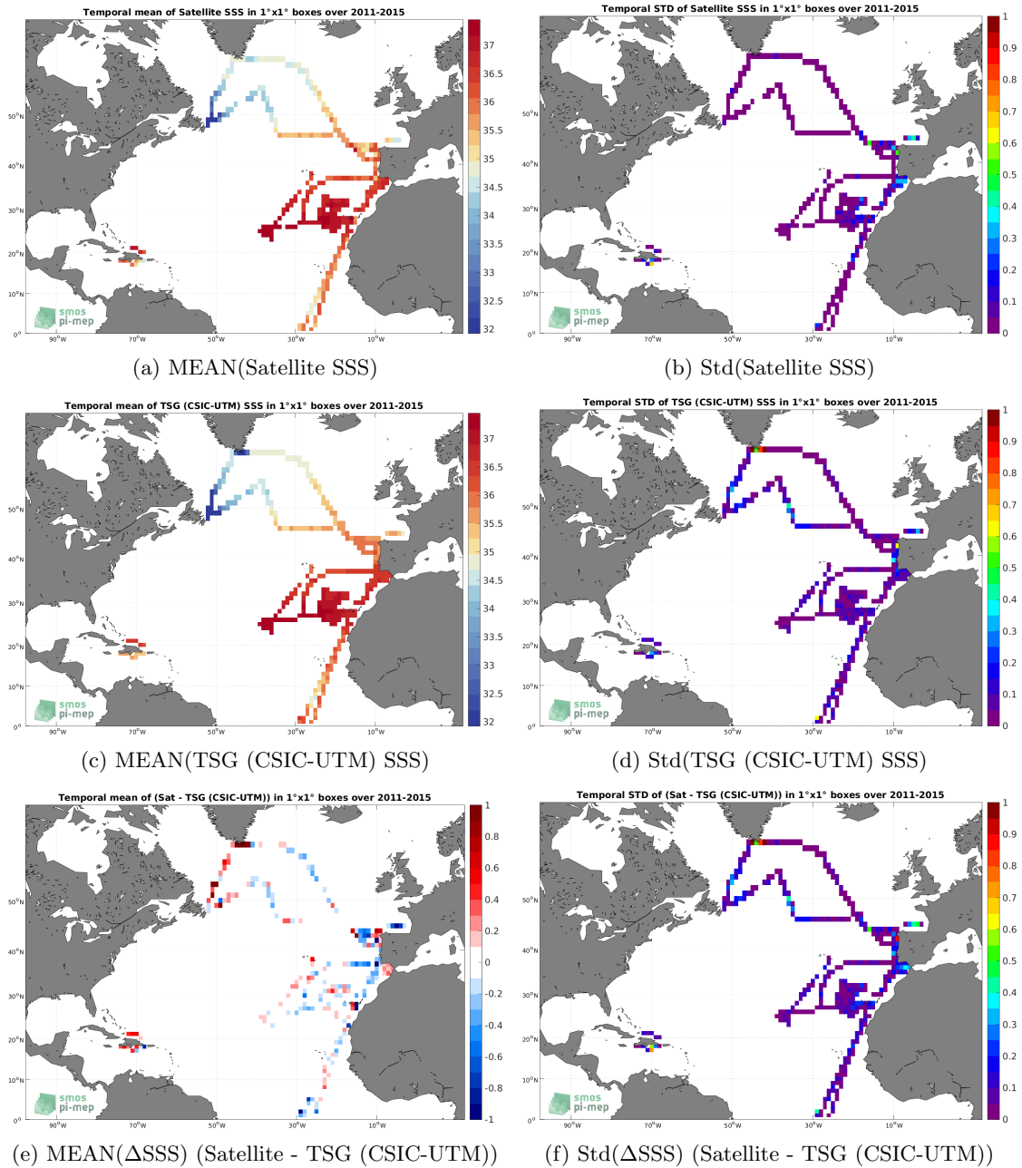
Figure 6: Temporal mean (left) and Std (right) of SSS from Aquarius SSS L3 OR v5 - 7-Day running (NASA-GSFC) (top), TSG (CSIC-UTM) (middle), and of \Delta SSS (Satellite - TSG (CSIC-UTM)). Only match-up pairs are used to generate these maps.
