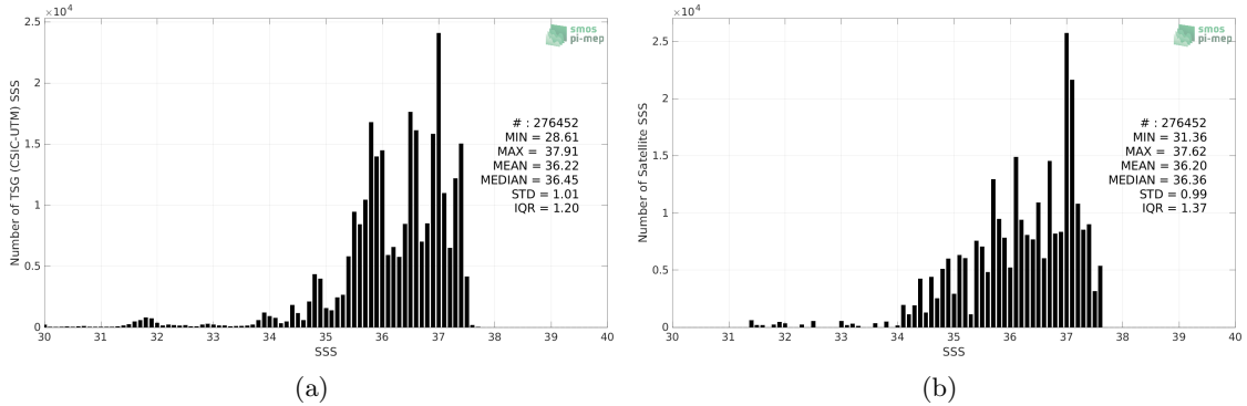
Figure 2: Histograms of SSS from TSG (CSIC-UTM) (a) and Aquarius SSS L3 OR v5 - 7-Day running (NASA-GSFC) (b) considering all match-up pairs per bins of 0.1 over the North Atlantic Ocean Pi-MEP region and for the full satellite product period.
