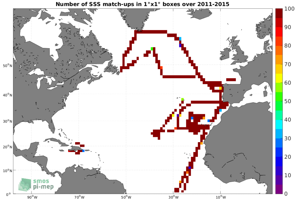
Figure 4: Number of SSS match-ups between TSG (CSIC-UTM) SSS and the Aquarius SSS L3 OR v5 - 7-Day running (NASA-GSFC) SSS product for the North Atlantic Ocean Pi-MEP region over 1^\circ \times 1^\circ boxes and for the full satellite product period.
