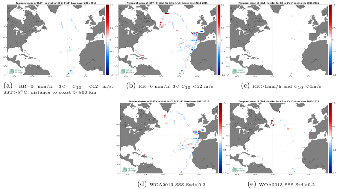
Figure 12: Temporal mean gridded over spatial boxes of size 1^\circ \times 1^\circ of \Delta SSS (Aquarius SSS L3 OR v5 - 7-Day running (NASA-GSFC) - TSG (CSIC-UTM)) for 5 different subdatasets corresponding to:RR=0 mm/h, 3 < U_{10} < 12 m/s, SST >5^\circ\text{C} , distance to coast > 800 km (a), RR=0 mm/h, 3 < U_{10} < 12 m/s (b), RR >1 mm/h and U_{10} < 4 m/s (c), WOA2013 SSS Std <0.2 (d), WOA2013 SSS Std >0.2 (e).
