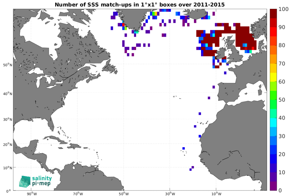
Figure 5: Number of SSS match-ups between ICES SSS and the Aquarius SSS L3 OR v5 - 7-Day running (NASA-GSFC) SSS product for the North Atlantic Ocean Pi-MEP region over 1^\circ \times 1^\circ boxes and for the full satellite product period.
