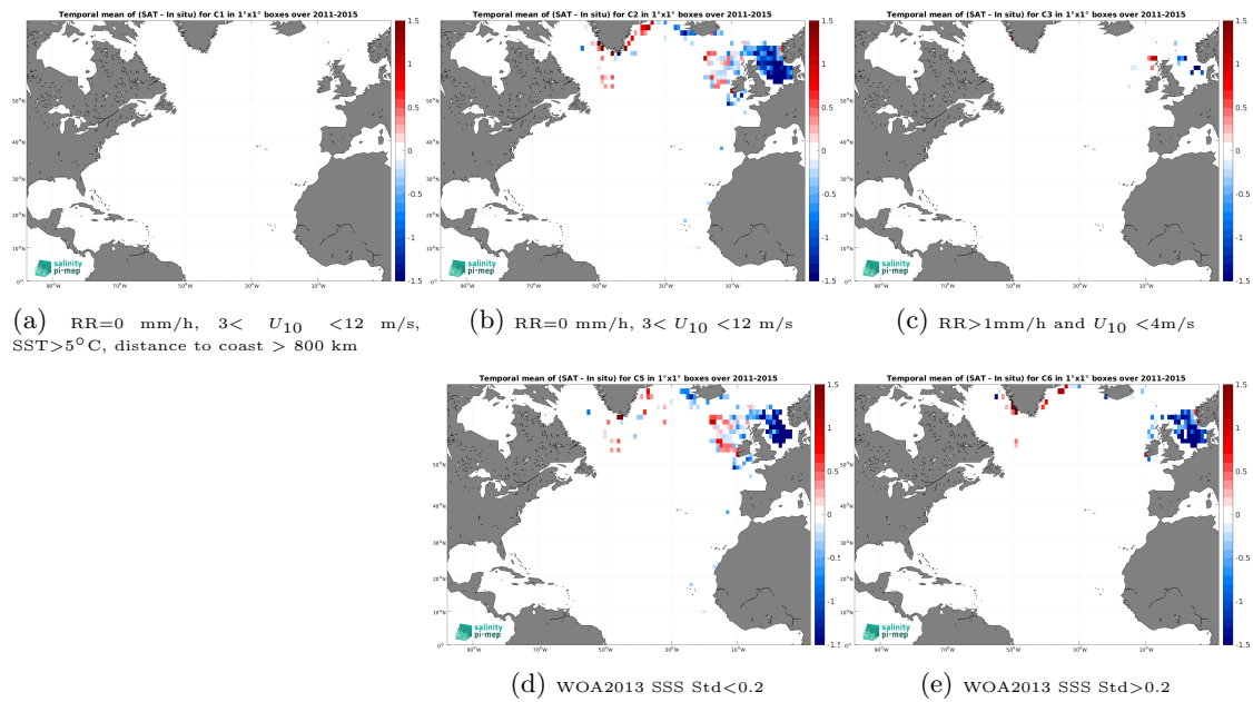
Figure 14: Temporal mean gridded over spatial boxes of size 1^\circ \times 1^\circ of \Delta SSS (Aquarius SSS L3 OR v5 - 7-Day running (NASA-GSFC) - ICES) for 5 different subdatasets corresponding to:RR=0 mm/h, 3 < U_{10} < 12 m/s, SST >5^\circ\text{C} , distance to coast > 800 km (a), RR=0 mm/h, 3 < U_{10} < 12 m/s (b), RR >1 mm/h and U_{10} < 4 m/s (c), WOA2013 SSS Std <0.2 (d), WOA2013 SSS Std >0.2 (e).
