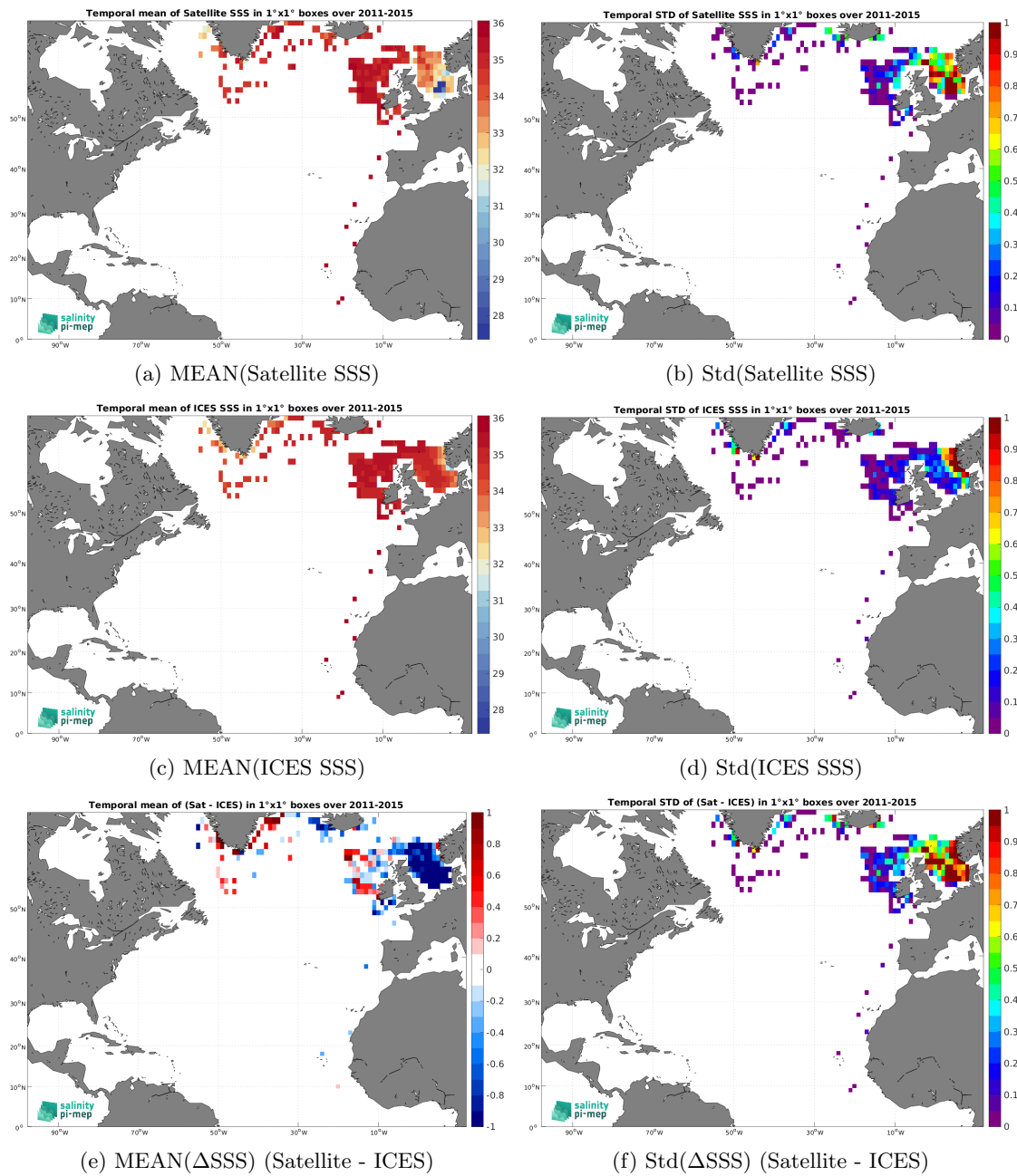
Figure 7: Temporal mean (left) and Std (right) of SSS from Aquarius SSS L3 OR v5 - 7-Day running (NASA-GSFC) (top), ICES (middle), and of \Delta SSS (Satellite - ICES). Only match-up pairs are used to generate these maps.
