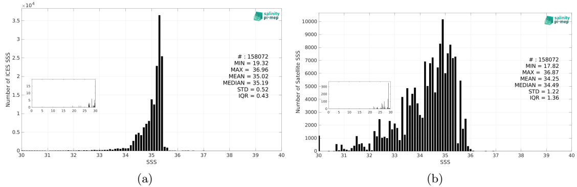
Figure 3: Histograms of SSS from ICES (a) and Aquarius SSS L3 OR v5 - 7-Day running (NASA-GSFC) (b) considering all match-up pairs per bins of 0.1 over the North Atlantic Ocean Pi-MEP region and for the full satellite product period.
