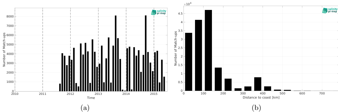
Figure 2: Number of match-ups between ICES and Aquarius SSS L3 OR v5 - 7-Day running (NASA-GSFC) SSS as a function of time (a) and as function of the distance to coast (b) over the North Atlantic Ocean Pi-MEP region and for the full satellite product period.
