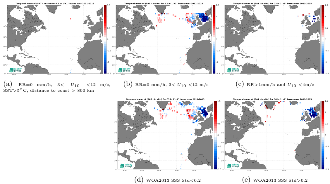
Figure 12: Temporal mean gridded over spatial boxes of size 1^\circ \times 1^\circ of \Delta SSS (Aquarius SSS L3 OR v5 - 7-Day running (NASA-GSFC) - ICES) for 5 different subdatasets corresponding to:RR=0 mm/h, 3 < U_{10} < 12 m/s, SST >5^\circ\text{C} , distance to coast > 800 km (a), RR=0 mm/h, 3 < U_{10} < 12 m/s (b), RR >1 mm/h and U_{10} < 4 m/s (c), WOA2013 SSS Std <0.2 (d), WOA2013 SSS Std >0.2 (e).
