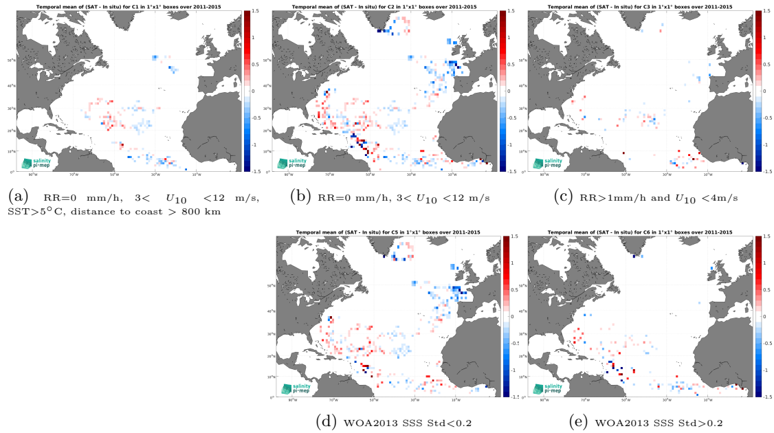
Figure 13: Temporal mean gridded over spatial boxes of size 1^\circ \times 1^\circ of \Delta\text{SSS} (Aquarius SSS L3 OR v5 - 7-Day running (NASA-GSFC) - Surface drifters) for 5 different subdatasets corresponding to:RR=0 mm/h, 3 < U_{10} < 12 m/s, SST >5^\circ\text{C} , distance to coast > 800 km (a), RR=0 mm/h, 3 < U_{10} < 12 m/s (b), RR >1 mm/h and U_{10} < 4 m/s (c), WOA2013 SSS Std <0.2 (d), WOA2013 SSS Std >0.2 (e).
