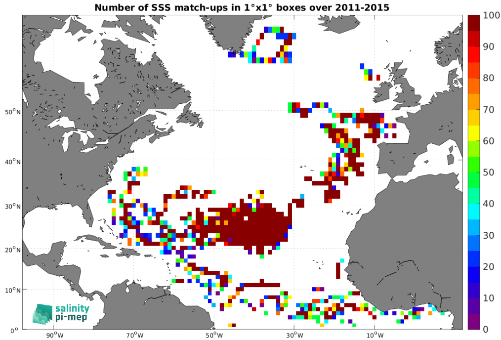
Figure 4: Number of SSS match-ups between Surface drifters SSS and the Aquarius SSS L3 OR v5 - 7-Day running (NASA-GSFC) SSS product for the North Atlantic Ocean Pi-MEP region over 1^\circ \times 1^\circ boxes and for the full satellite product period.
