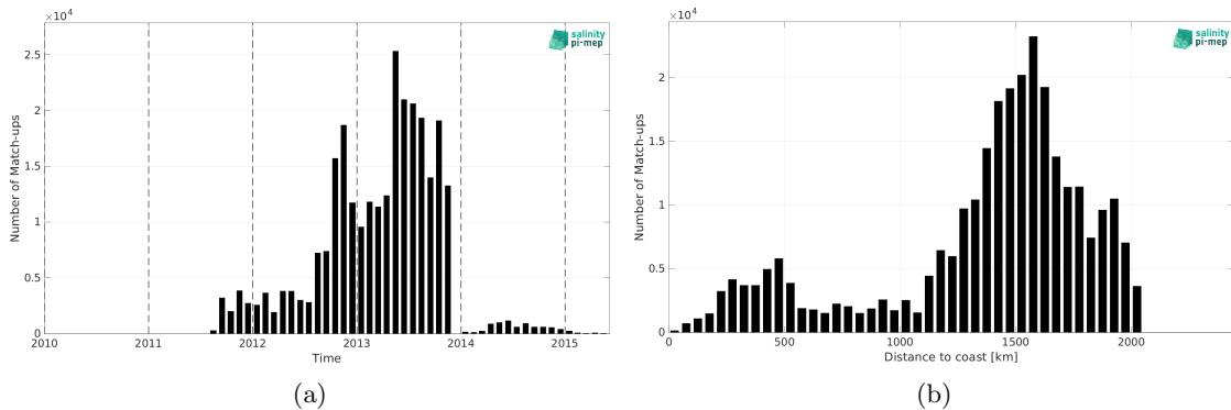
Figure 2: Number of match-ups between Surface drifters and Aquarius SSS L3 OR v5 - 7-Day running (NASA-GSFC) SSS as a function of time (a) and as function of the distance to coast (b) over the North Atlantic Ocean Pi-MEP region and for the full satellite product period.
