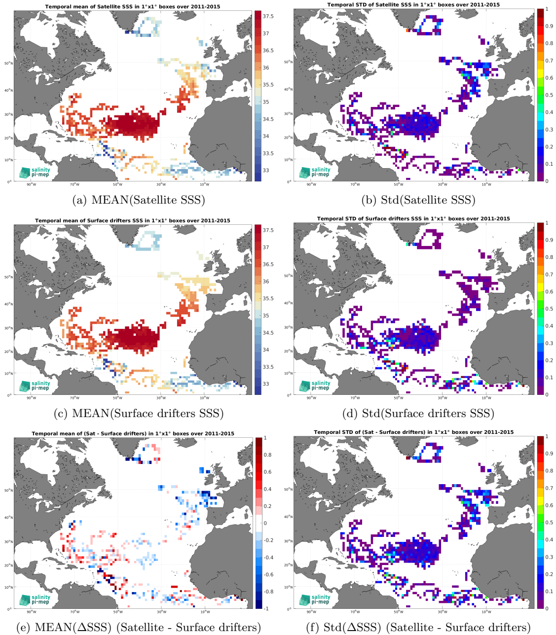
Figure 6: Temporal mean (left) and Std (right) of SSS from Aquarius SSS L3 OR v5 - 7-Day running (NASA-GSFC) (top), Surface drifters (middle), and of \Delta SSS (Satellite - Surface drifters). Only match-up pairs are used to generate these maps.
