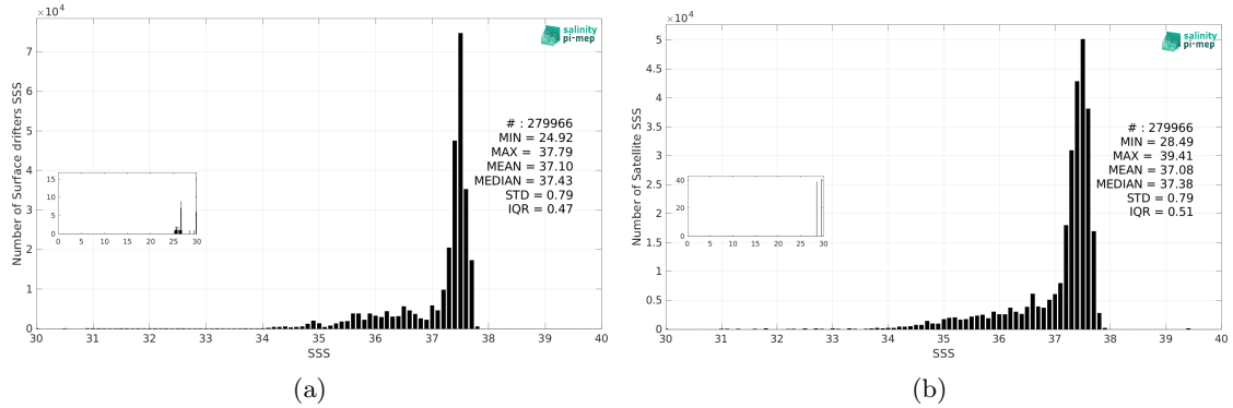
Figure 3: Histograms of SSS from Surface drifters (a) and Aquarius SSS L3 OR v5 - 7-Day running (NASA-GSFC) (b) considering all match-up pairs per bins of 0.1 over the North Atlantic Ocean Pi-MEP region and for the full satellite product period.
