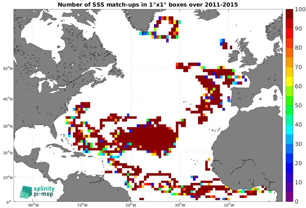
Figure 3: Number of SSS match-ups between Surface drifters SSS and the Aquarius SSS L3 OR v5 - 7-Day running (NASA-GSFC) SSS product for the North Atlantic Ocean Pi-MEP region over 1^\circ \times 1^\circ boxes and for the full satellite product period.
