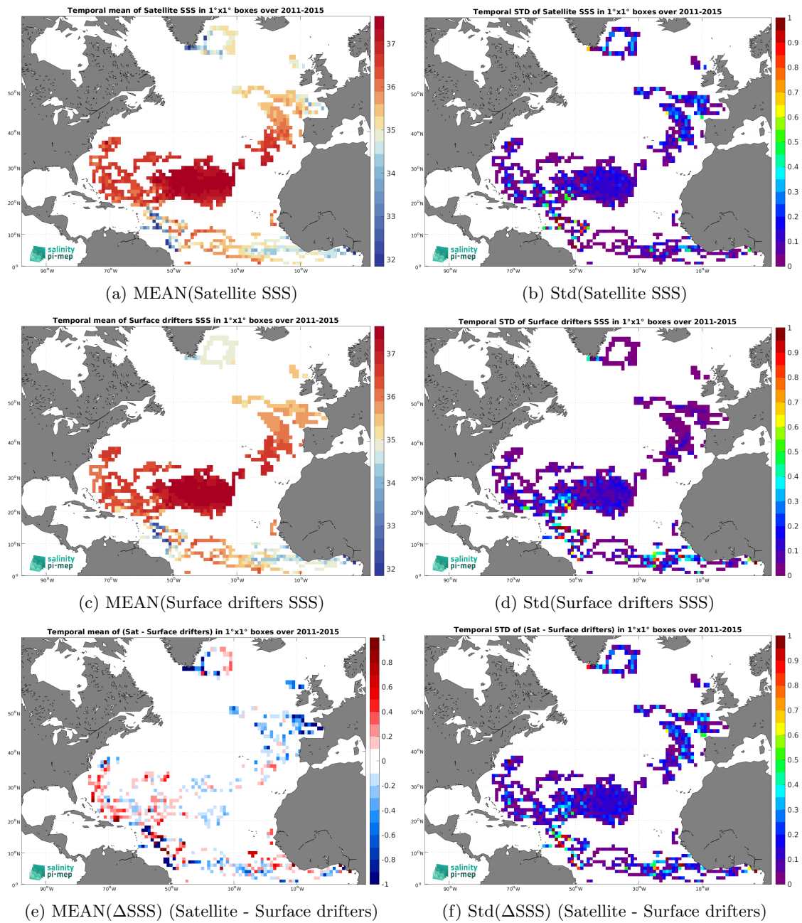
Figure 5: Temporal mean (left) and Std (right) of SSS from Aquarius SSS L3 OR v5 - 7-Day running (NASA-GSFC) (top), Surface drifters (middle), and of \Delta SSS (Satellite - Surface drifters). Only match-up pairs are used to generate these maps.
