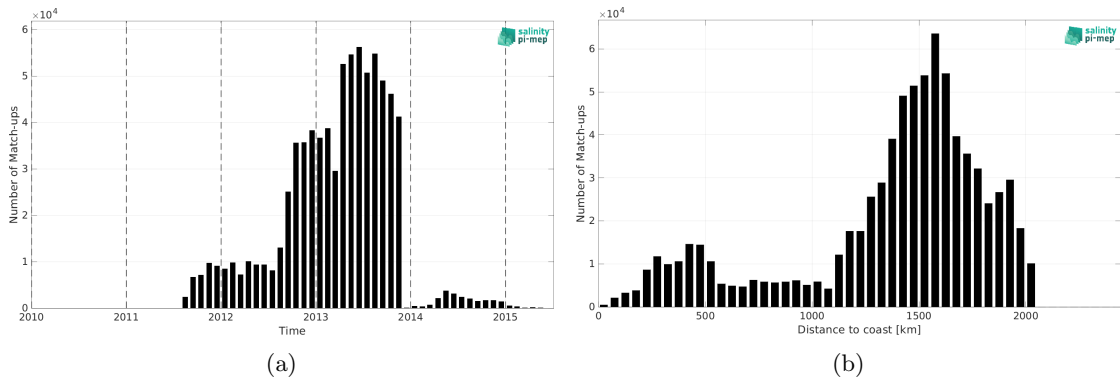
Figure 1: Number of match-ups between Surface drifters and Aquarius SSS L3 OR v5 - 7-Day running (NASA-GSFC) SSS as a function of time (a) and as function of the distance to coast (b) over the North Atlantic Ocean Pi-MEP region and for the full satellite product period.
