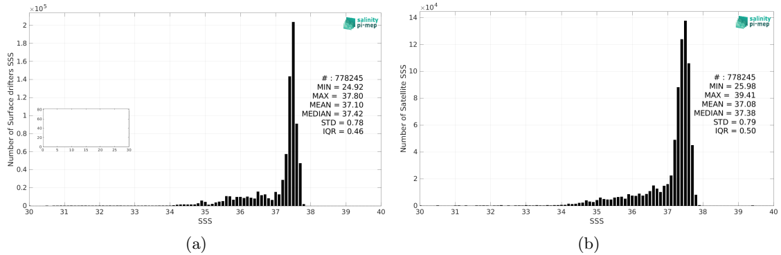
Figure 2: Histograms of SSS from Surface drifters (a) and Aquarius SSS L3 OR v5 - 7-Day running (NASA-GSFC) (b) considering all match-up pairs per bins of 0.1 over the North Atlantic Ocean Pi-MEP region and for the full satellite product period.
