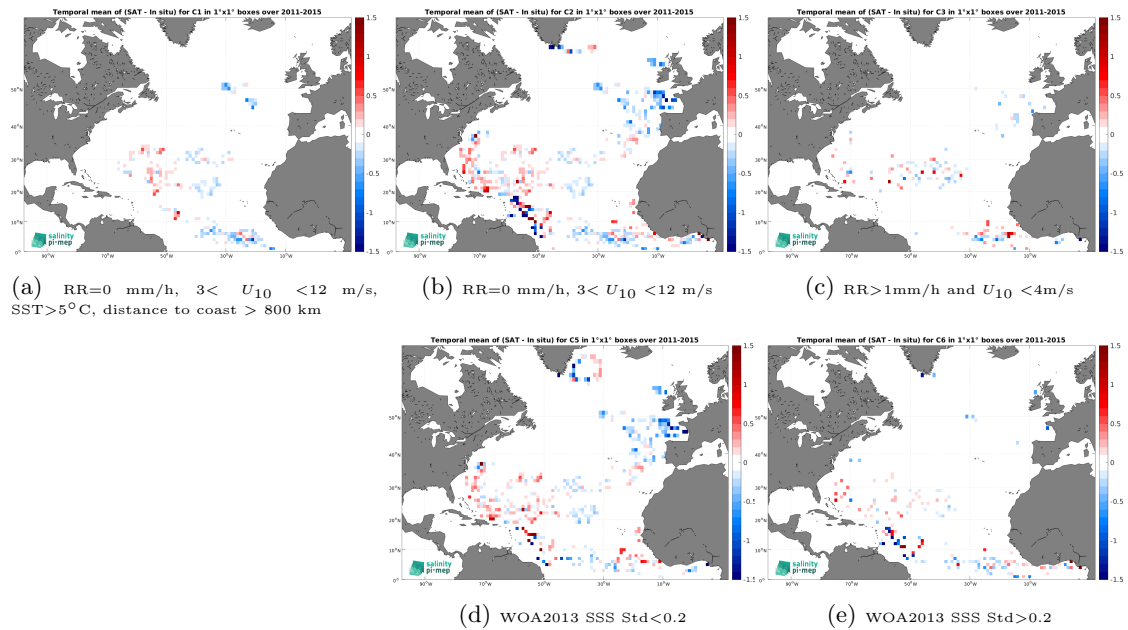
Figure 11: Temporal mean gridded over spatial boxes of size 1^\circ \times 1^\circ of \Delta\text{SSS} (Aquarius SSS L3 OR v5 - 7-Day running (NASA-GSFC) - Surface drifters) for 5 different subdatasets corresponding to:RR=0 mm/h, 3 < U_{10} < 12 m/s, SST >5^\circ\text{C} , distance to coast > 800 km (a), RR=0 mm/h, 3 < U_{10} < 12 m/s (b), RR >1 mm/h and U_{10} < 4 m/s (c), WOA2013 SSS Std <0.2 (d), WOA2013 SSS Std >0.2 (e).
