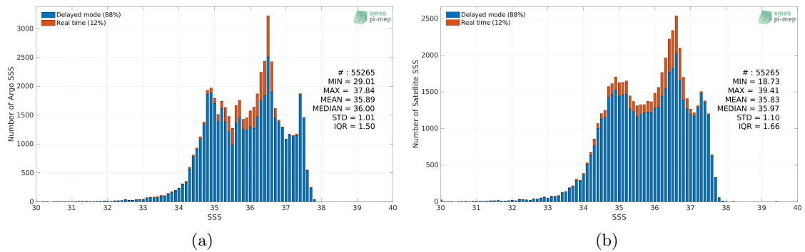
Figure 2: Histograms of SSS from Argo (a) and Aquarius SSS L3 OR v5 - 7-Day running (NASA-GSFC) (b) considering all match-up pairs per bins of 0.1 over the North Atlantic Ocean Pi-MEP region and for the full satellite product period.
