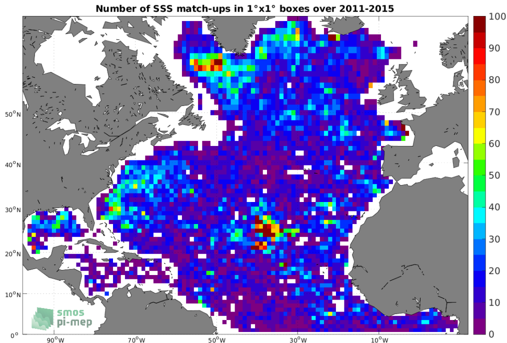
Figure 4: Number of SSS match-ups between Argo SSS and the Aquarius SSS L3 OR v5 - 7-Day running (NASA-GSFC) SSS product for the North Atlantic Ocean Pi-MEP region over 1^\circ \times 1^\circ boxes and for the full satellite product period.
