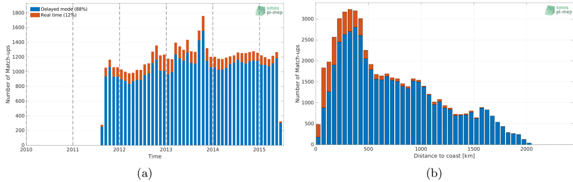
Figure 1: Number of match-ups between Argo and Aquarius SSS L3 OR v5 - 7-Day running (NASA-GSFC) SSS as a function of time (a) and as function of the distance to coast (b) over the North Atlantic Ocean Pi-MEP region and for the full satellite product period.
