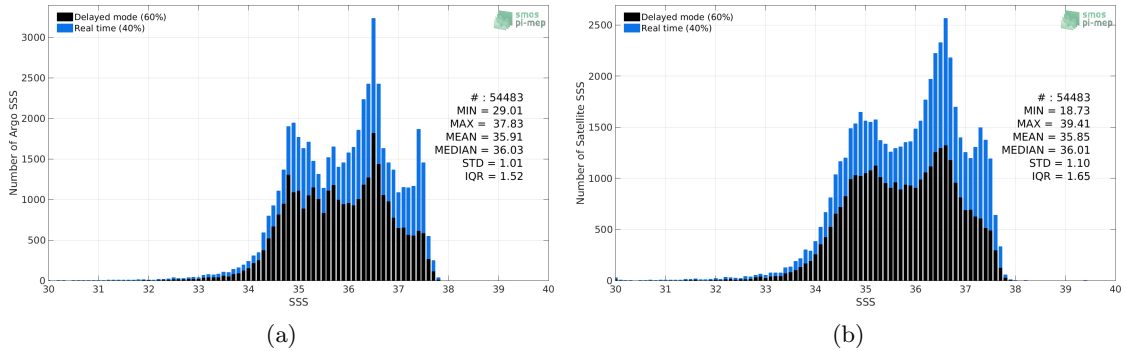
Figure 2: Histograms of SSS from Argo (a) and Aquarius-L3-OR-V5-7DAY-RUNNING-1DEG (b) considering all match-up pairs per bins of 0.1 over the North Atlantic Ocean Pi-MEP region and for the full satellite product period.
