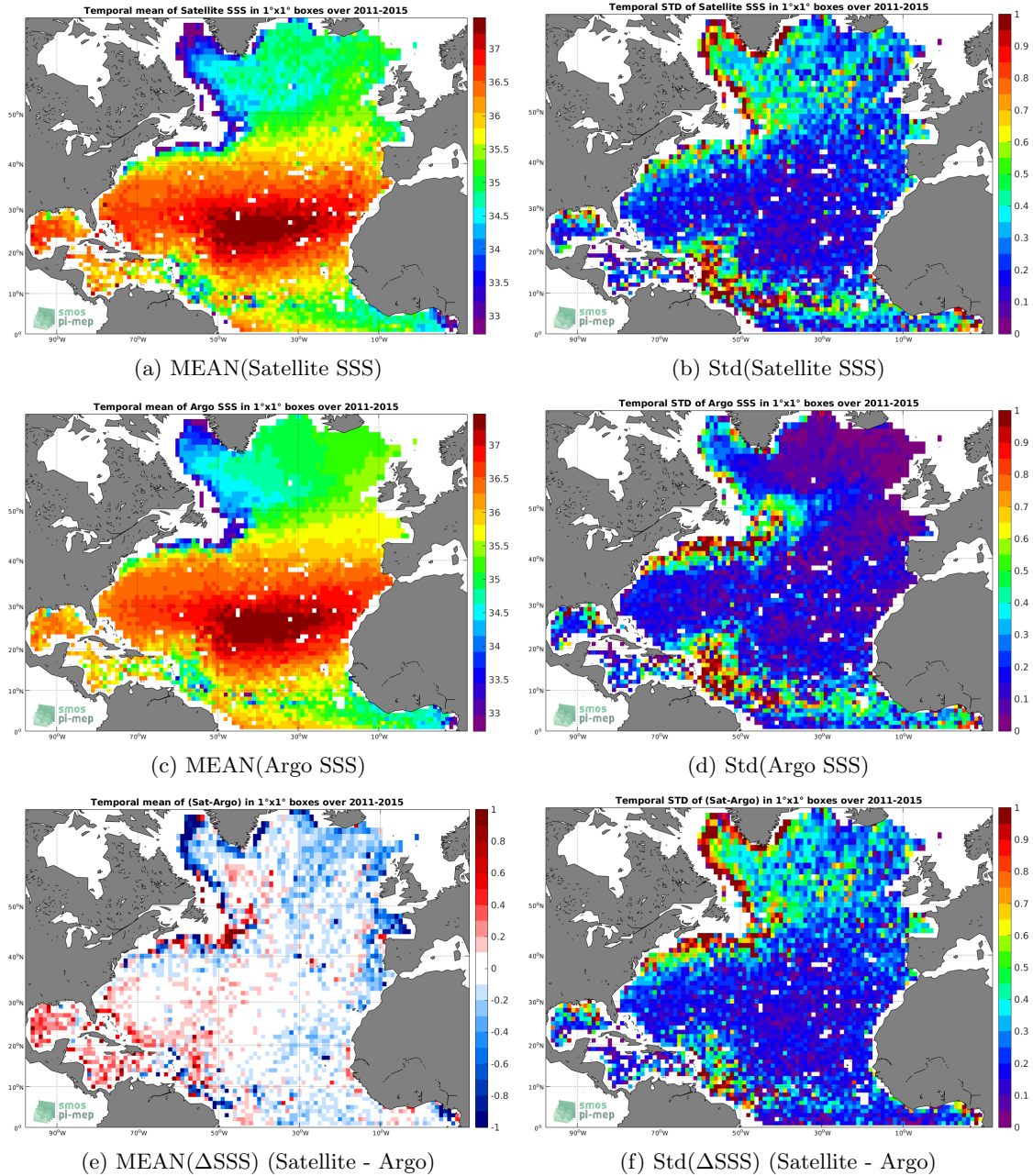
Figure 6: Temporal mean (left) and Std (right) of SSS from Aquarius-L3-OR-V5-7DAY-RUNNING-1DEG (top), Argo (middle), and of \Delta SSS (Satellite - Argo). Only match-up pairs are used to generate these maps.
