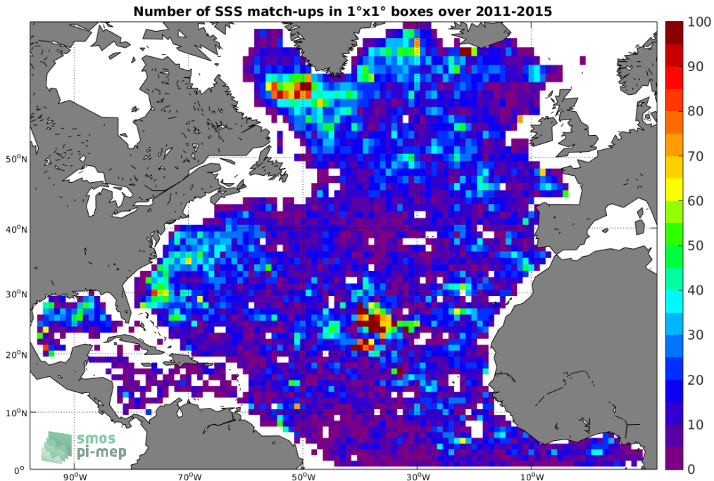
Figure 4: Number of SSS match-ups between Argo SSS and the Aquarius-L3-OR-V5-7DAY-RUNNING-1DEG SSS product for the North Atlantic Ocean Pi-MEP region over 1^\circ \times 1^\circ boxes and for the full satellite product period.
