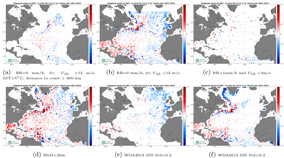
Figure 12: Temporal mean gridded over spatial boxes of size 1^\circ \times 1^\circ of \Delta SSS (Aquarius-L3-OR-V5-7DAY-RUNNING-1DEG - Argo) for 6 different subdatasets corresponding to:RR=0 mm/h, 3 < U_{10} < 12 m/s, SST > 5^\circ C, distance to coast > 800 km (a), RR=0 mm/h, 3 < U_{10} < 12 m/s (b), RR > 1 mm/h and U_{10} < 4 m/s (c),MLD < 20 m (d),WOA2013 SSS Std < 0.2 (e),WOA2013 SSS Std > 0.2 (f).
