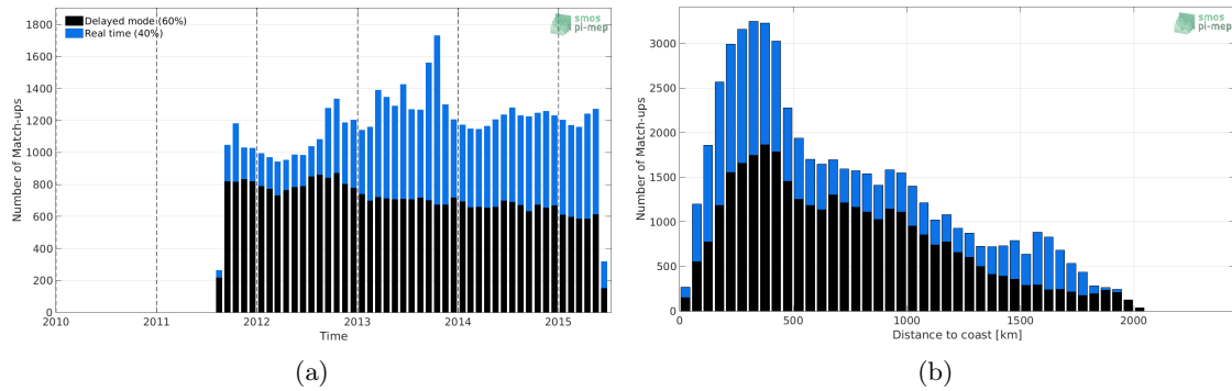
Figure 1: Number of match-ups between Argo and Aquarius-L3-OR-V5-7DAY-RUNNING-1DEG SSS as a function of time (a) and as function of the distance to coast (b) over the North Atlantic Ocean Pi-MEP region and for the full satellite product period.
