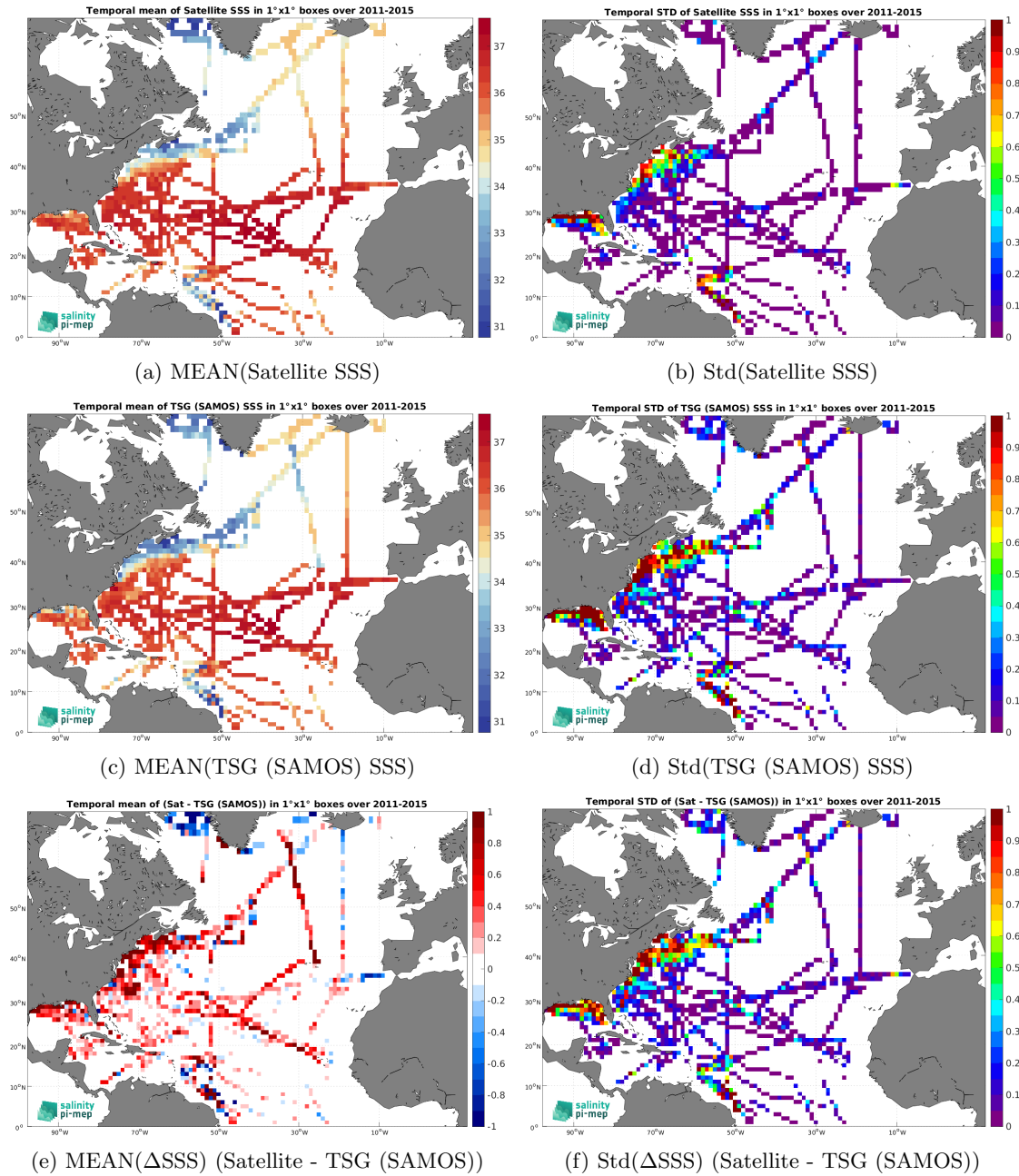
Figure 7: Temporal mean (left) and Std (right) of SSS from Aquarius SSS L3 OR v5 - 7-Day running - Rain mask (NASA-GSFC) (top), TSG (SAMOS) (middle), and of \Delta SSS (Satellite - TSG (SAMOS)). Only match-up pairs are used to generate these maps.
