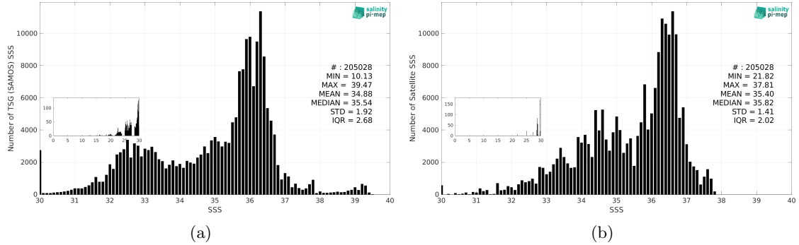
Figure 3: Histograms of SSS from TSG (SAMOS) (a) and Aquarius SSS L3 OR v5 - 7-Day running - Rain mask (NASA-GSFC) (b) considering all match-up pairs per bins of 0.1 over the North Atlantic Ocean Pi-MEP region and for the full satellite product period.
