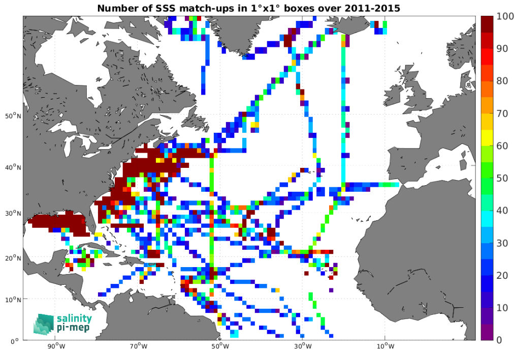
Figure 5: Number of SSS match-ups between TSG (SAMOS) SSS and the Aquarius SSS L3 OR v5 - 7-Day running - Rain mask (NASA-GSFC) SSS product for the North Atlantic Ocean Pi-MEP region over 1^\circ \times 1^\circ boxes and for the full satellite product period.
