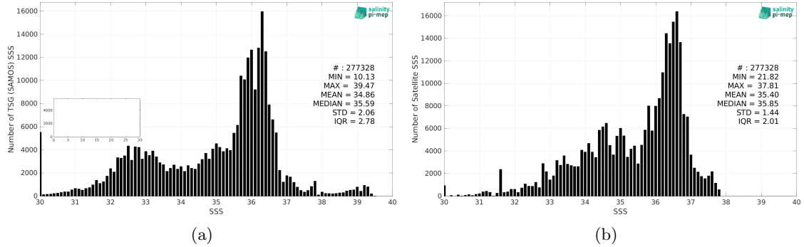
Figure 2: Histograms of SSS from TSG (SAMOS) (a) and Aquarius SSS L3 OR v5 - 7-Day running - Rain mask (NASA-GSFC) (b) considering all match-up pairs per bins of 0.1 over the North Atlantic Ocean Pi-MEP region and for the full satellite product period.
