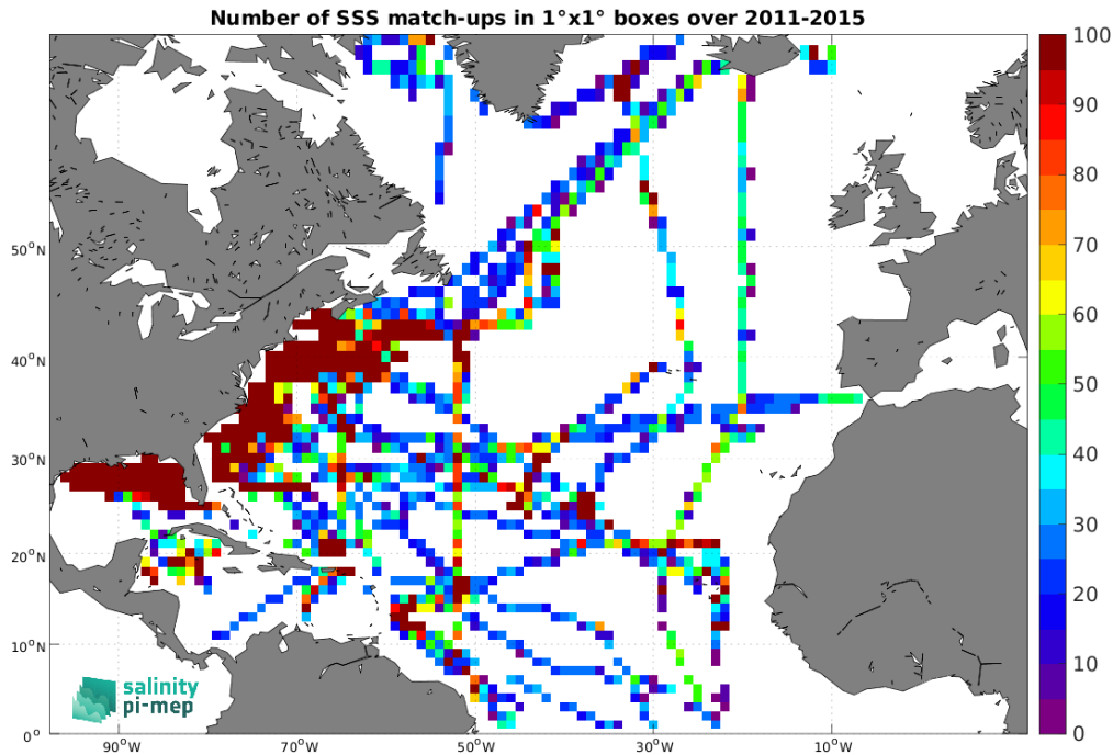
Figure 4: Number of SSS match-ups between TSG (SAMOS) SSS and the Aquarius SSS L3 OR v5 - 7-Day running - Rain mask (NASA-GSFC) SSS product for the North Atlantic Ocean Pi-MEP region over 1^\circ \times 1^\circ boxes and for the full satellite product period.
