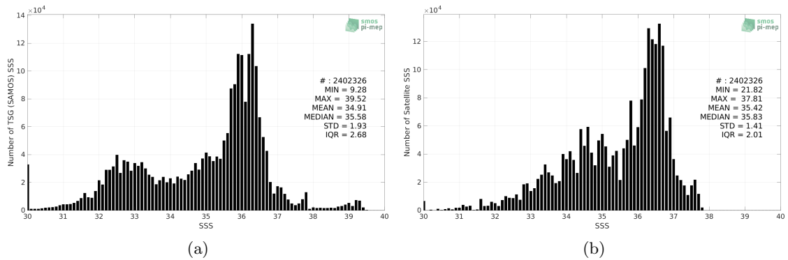
Figure 2: Histograms of SSS from TSG (SAMOS) (a) and Aquarius SSS L3 OR v5 - 7-Day running - Rain mask (NASA-GSFC) (b) considering all match-up pairs per bins of 0.1 over the North Atlantic Ocean Pi-MEP region and for the full satellite product period.
