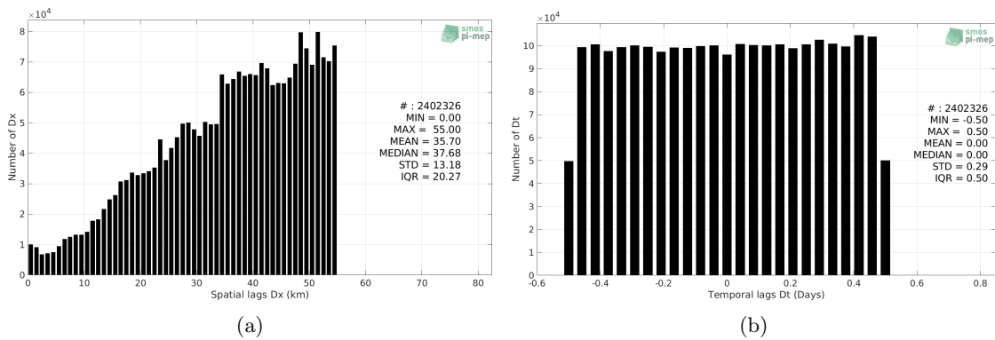
Figure 5: Histograms of the spatial (a) and temporal (b) lags between the location/time of the TSG (SAMOS) measurement and the date of the corresponding Aquarius SSS L3 OR v5 - 7-Day running - Rain mask (NASA-GSFC) SSS pixel.
