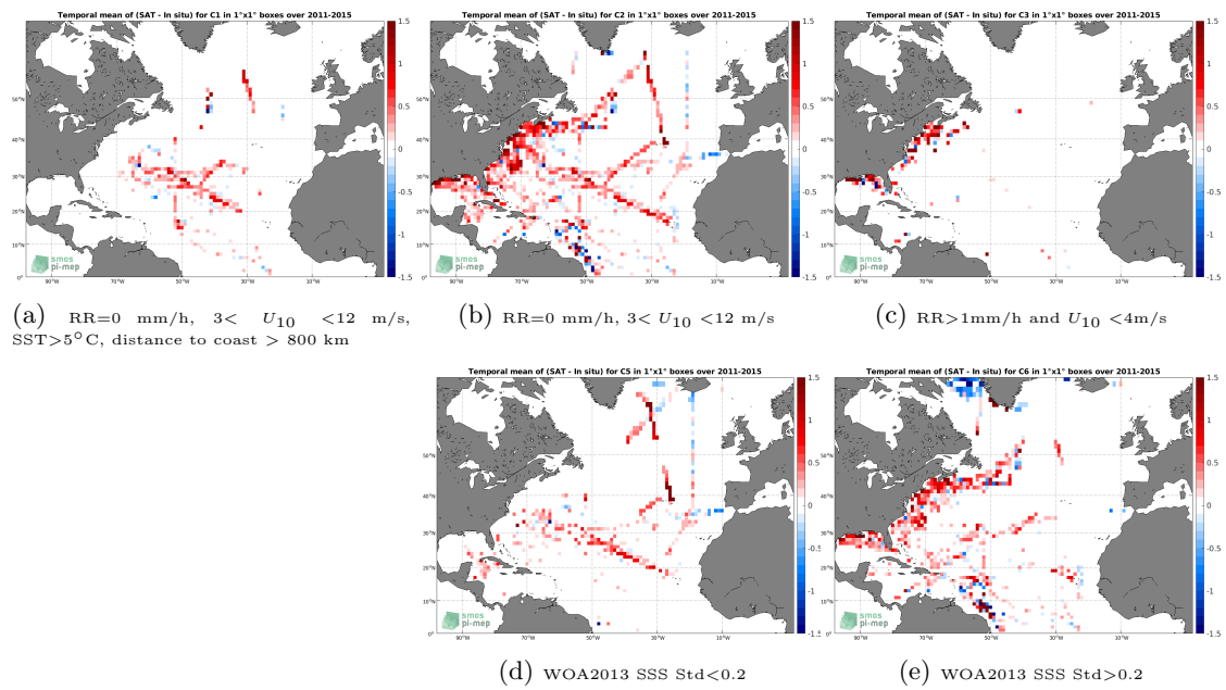
Figure 12: Temporal mean gridded over spatial boxes of size 1^\circ \times 1^\circ of \Delta\text{SSS} (Aquarius SSS L3 OR v5 - 7-Day running - Rain mask (NASA-GSFC) - TSG (SAMOS)) for 5 different subdatasets corresponding to:RR=0 mm/h, 3 < U_{10} < 12 m/s, SST >5^\circ\text{C} , distance to coast > 800 km (a), RR=0 mm/h, 3 < U_{10} < 12 m/s (b), RR >1 mm/h and U_{10} < 4 m/s (c), WOA2013 SSS Std <0.2 (d), WOA2013 SSS Std >0.2 (e).
