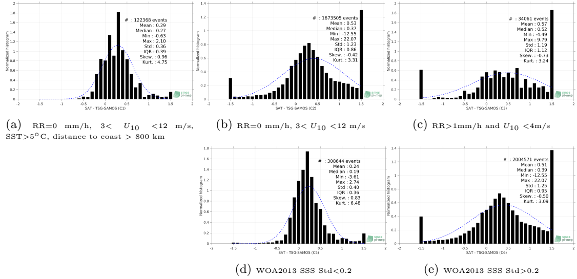
Figure 13: Normalized histogram of \Delta\text{SSS} (Aquarius-L3-OR-V5-7DAY-RUNNING-RAIN-MASK-1DEG - TSG-SAMOS) for 5 different subdatasets corresponding to: RR=0 mm/h, 3 < U_{10} < 12 m/s, SST>5°C, distance to coast > 800 km (a), RR=0 mm/h, 3 < U_{10} < 12 m/s (b), RR>1mm/h and U_{10} < 4 m/s (c), WOA2013 SSS Std<0.2 (d), WOA2013 SSS Std>0.2 (e).
