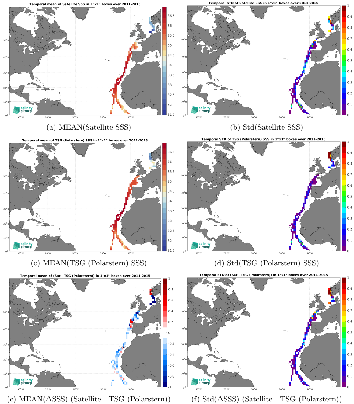
Figure 7: Temporal mean (left) and Std (right) of SSS from Aquarius SSS L3 OR v5 - 7-Day running - Rain mask (NASA-GSFC) (top), TSG (Polarstern) (middle), and of \Delta SSS (Satellite - TSG (Polarstern)). Only match-up pairs are used to generate these maps.
