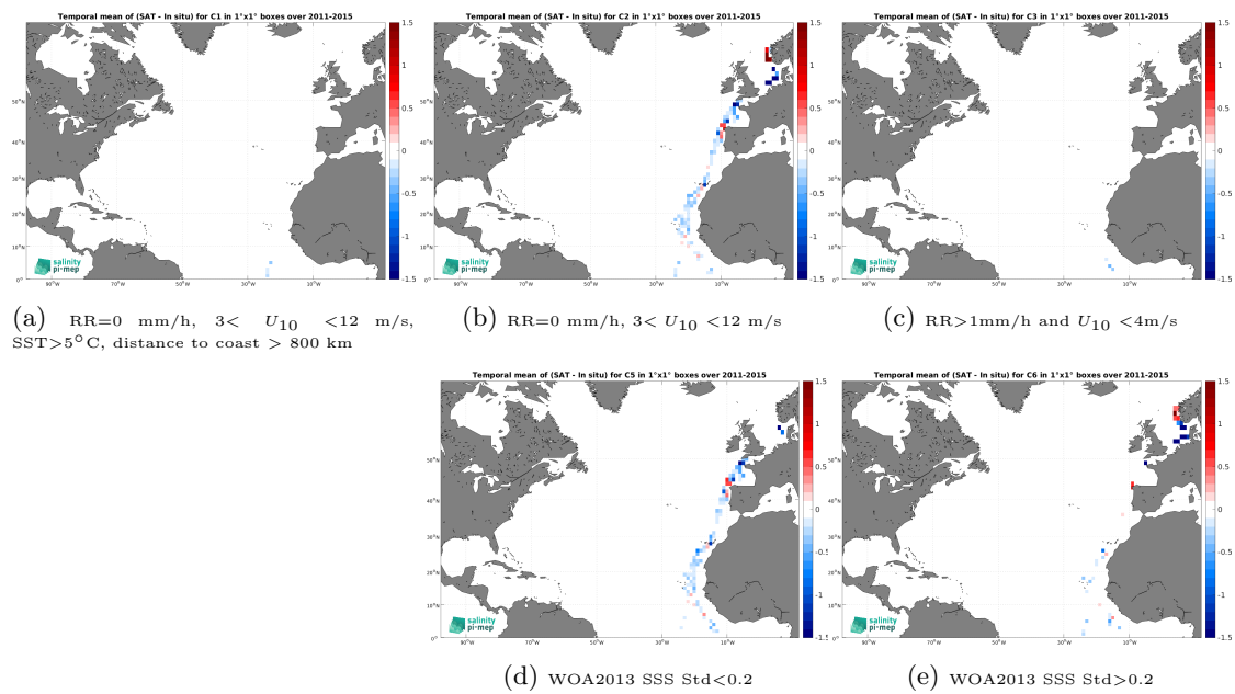
Figure 14: Temporal mean gridded over spatial boxes of size 1^\circ \times 1^\circ of \Delta SSS (Aquarius SSS L3 OR v5 - 7-Day running - Rain mask (NASA-GSFC) - TSG (Polarstern)) for 5 different subdatasets corresponding to:RR=0 mm/h, 3 < U_{10} < 12 m/s, SST >5^\circ\text{C} , distance to coast > 800 km (a), RR=0 mm/h, 3 < U_{10} < 12 m/s (b), RR >1 mm/h and U_{10} < 4 m/s (c), WOA2013 SSS Std <0.2 (d), WOA2013 SSS Std >0.2 (e).
