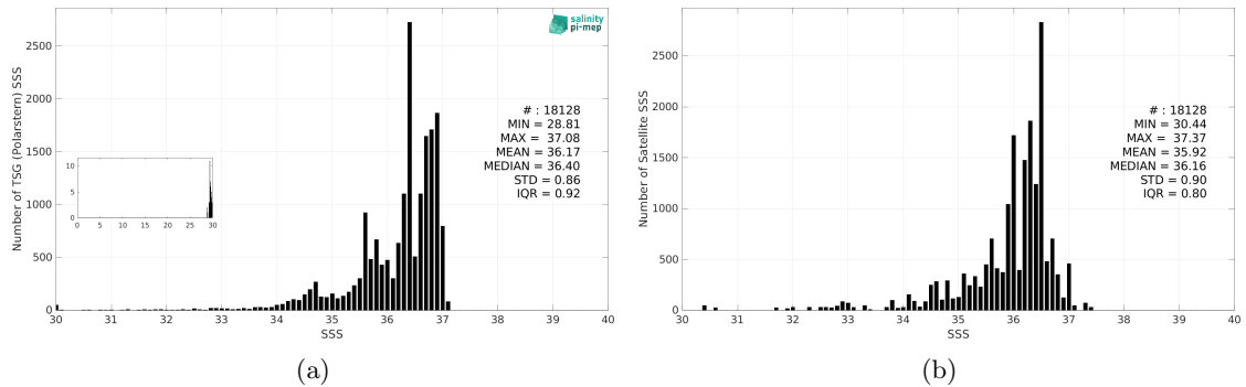
Figure 3: Histograms of SSS from TSG (Polarstern) (a) and Aquarius SSS L3 OR v5 - 7-Day running - Rain mask (NASA-GSFC) (b) considering all match-up pairs per bins of 0.1 over the North Atlantic Ocean Pi-MEP region and for the full satellite product period.
