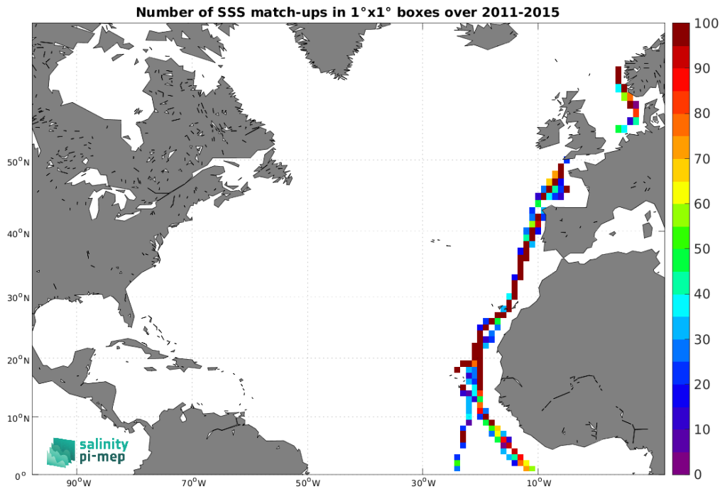
Figure 5: Number of SSS match-ups between TSG (Polarstern) SSS and the Aquarius SSS L3 OR v5 - 7-Day running - Rain mask (NASA-GSFC) SSS product for the North Atlantic Ocean Pi-MEP region over 1^\circ \times 1^\circ boxes and for the full satellite product period.
