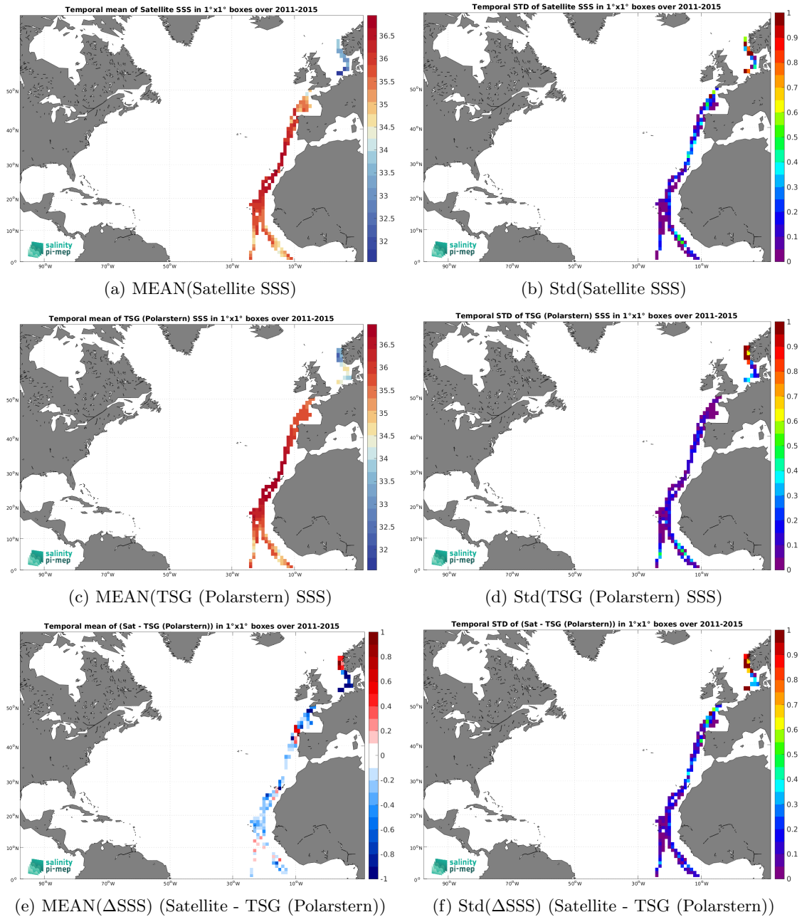
Figure 6: Temporal mean (left) and Std (right) of SSS from Aquarius SSS L3 OR v5 - 7-Day running - Rain mask (NASA-GSFC) (top), TSG (Polarstern) (middle), and of \Delta SSS (Satellite - TSG (Polarstern)). Only match-up pairs are used to generate these maps.
