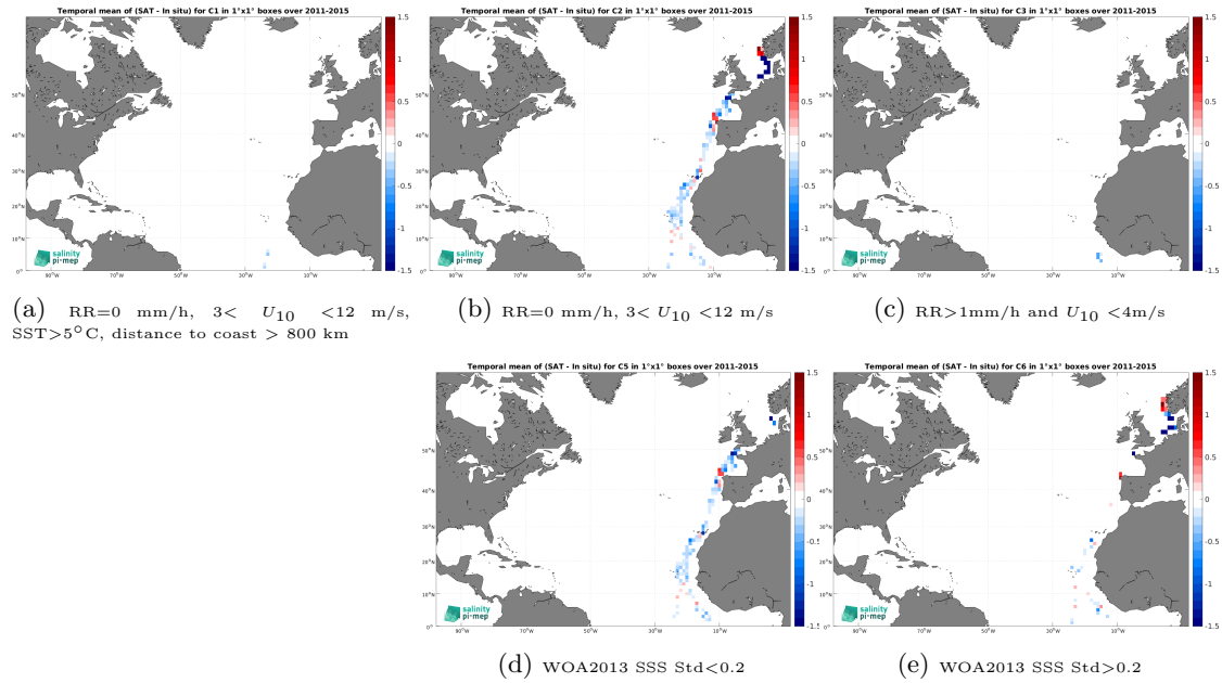
Figure 12: Temporal mean gridded over spatial boxes of size 1^\circ \times 1^\circ of \Delta SSS (Aquarius SSS L3 OR v5 - 7-Day running - Rain mask (NASA-GSFC) - TSG (Polarstern)) for 5 different subdatasets corresponding to:RR=0 mm/h, 3 < U_{10} < 12 m/s, SST >5^\circ\text{C} , distance to coast > 800 km (a), RR=0 mm/h, 3 < U_{10} < 12 m/s (b), RR >1 mm/h and U_{10} < 4 m/s (c), WOA2013 SSS Std <0.2 (d), WOA2013 SSS Std >0.2 (e).
