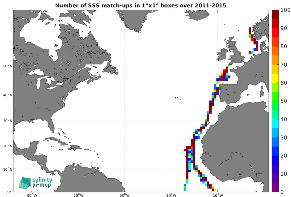
Figure 4: Number of SSS match-ups between TSG (Polarstern) SSS and the Aquarius SSS L3 OR v5 - 7-Day running - Rain mask (NASA-GSFC) SSS product for the North Atlantic Ocean Pi-MEP region over 1^\circ \times 1^\circ boxes and for the full satellite product period.
