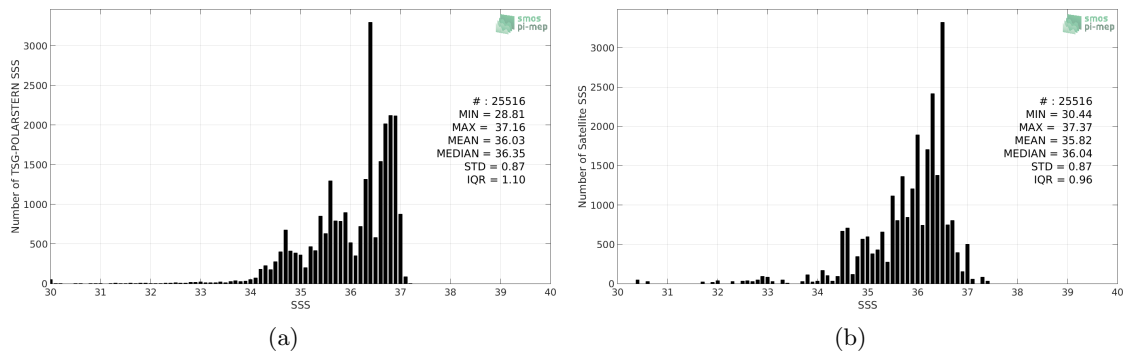
Figure 2: Histograms of SSS from TSG-POLARSTERN (a) and Aquarius-L3-OR-V5-7DAY-RUNNING-RAIN-MASK-1DEG (b) considering all match-up pairs per bins of 0.1 over the North Atlantic Ocean Pi-MEP region and for the full satellite product period.
