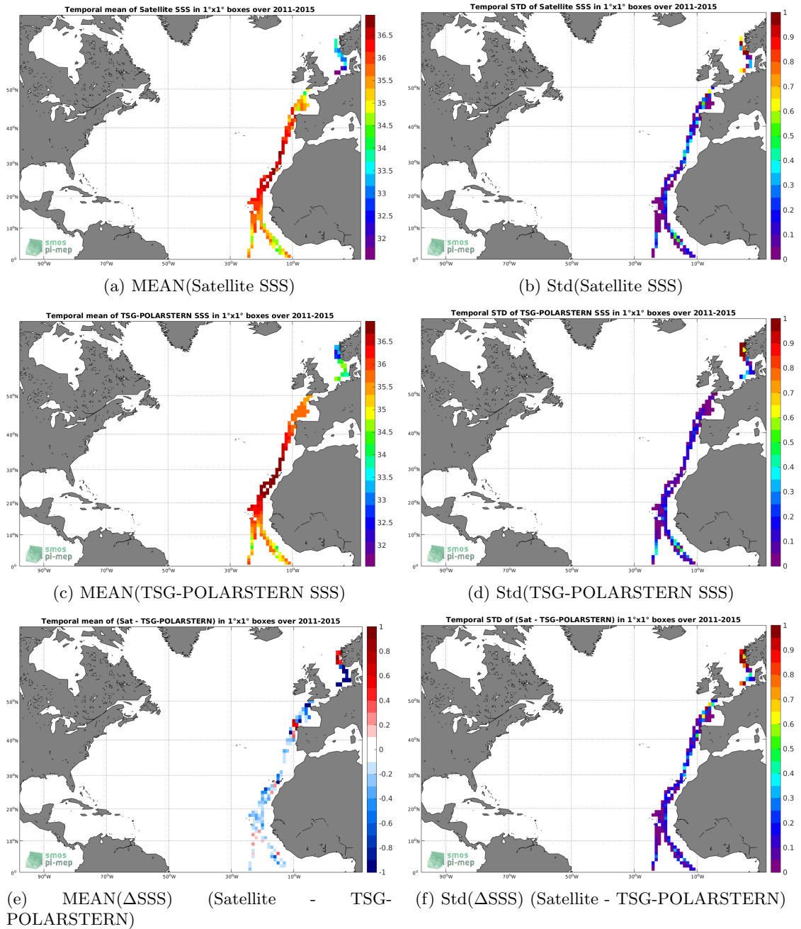
Figure 6: Temporal mean (left) and Std (right) of SSS from Aquarius-L3-OR-V5-7DAY-RUNNING-RAIN-MASK-1DEG (top), TSG-POLARSTERN (middle), and of \Delta SSS (Satellite - TSG-POLARSTERN). Only match-up pairs are used to generate these maps.
