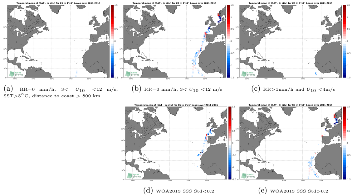
Figure 12: Temporal mean gridded over spatial boxes of size 1^\circ \times 1^\circ of \Delta SSS (Aquarius-L3-OR-V5-7DAY-RUNNING-RAIN-MASK-1DEG - TSG-POLARSTERN) for 5 different subdatasets corresponding to:RR=0 mm/h, 3 < U_{10} < 12 m/s, SST > 5^\circ\text{C} , distance to coast > 800 km (a), RR=0 mm/h, 3 < U_{10} < 12 m/s (b), RR > 1 mm/h and U_{10} < 4 m/s (c), WOA2013 SSS Std < 0.2 (d), WOA2013 SSS Std > 0.2 (e).
