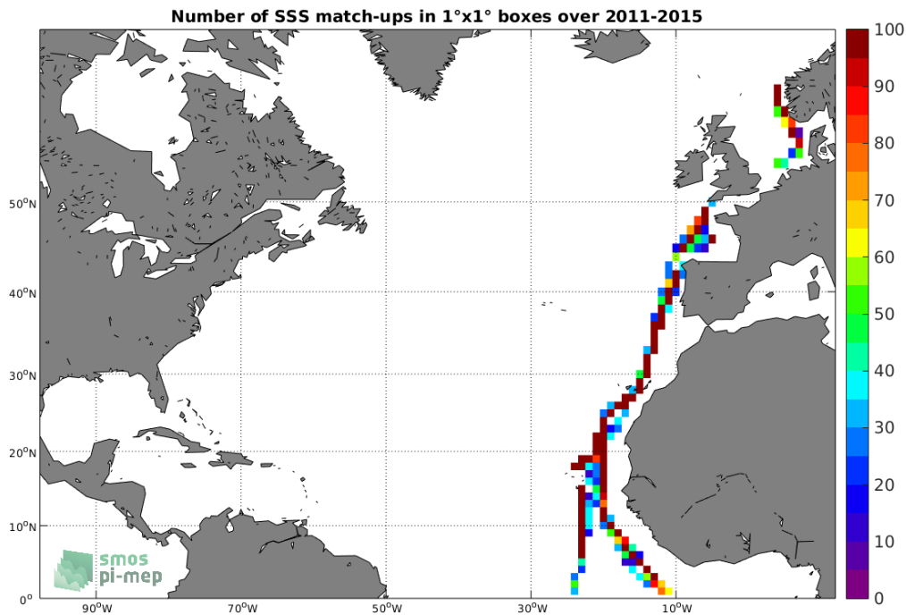
Figure 4: Number of SSS match-ups between TSG-POLARSTERN SSS and the Aquarius-L3-OR-V5-7DAY-RUNNING-RAIN-MASK-1DEG SSS product for the North Atlantic Ocean Pi-MEP region over 1^\circ \times 1^\circ boxes and for the full satellite product period.
