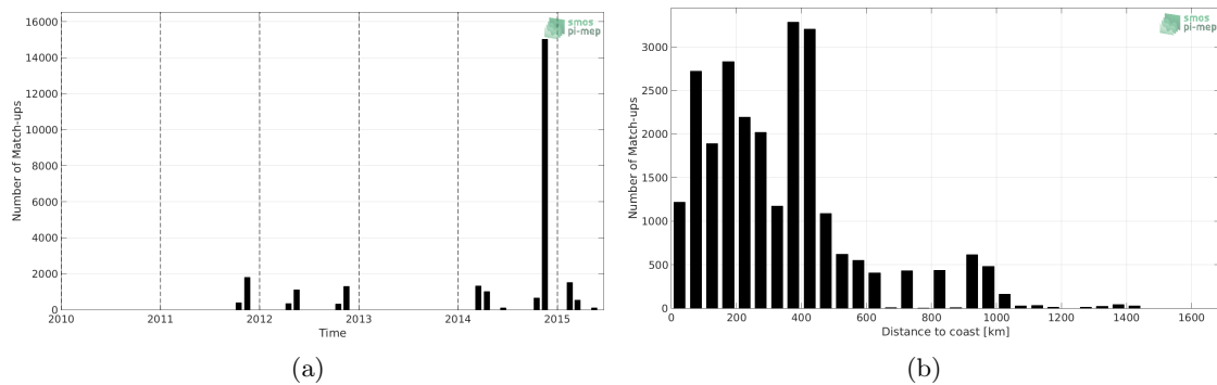
Figure 1: Number of match-ups between TSG-POLARSTERN and Aquarius-L3-OR-V5-7DAY-RUNNING-RAIN-MASK-1DEG SSS as a function of time (a) and as function of the distance to coast (b) over the North Atlantic Ocean Pi-MEP region and for the full satellite product period.
