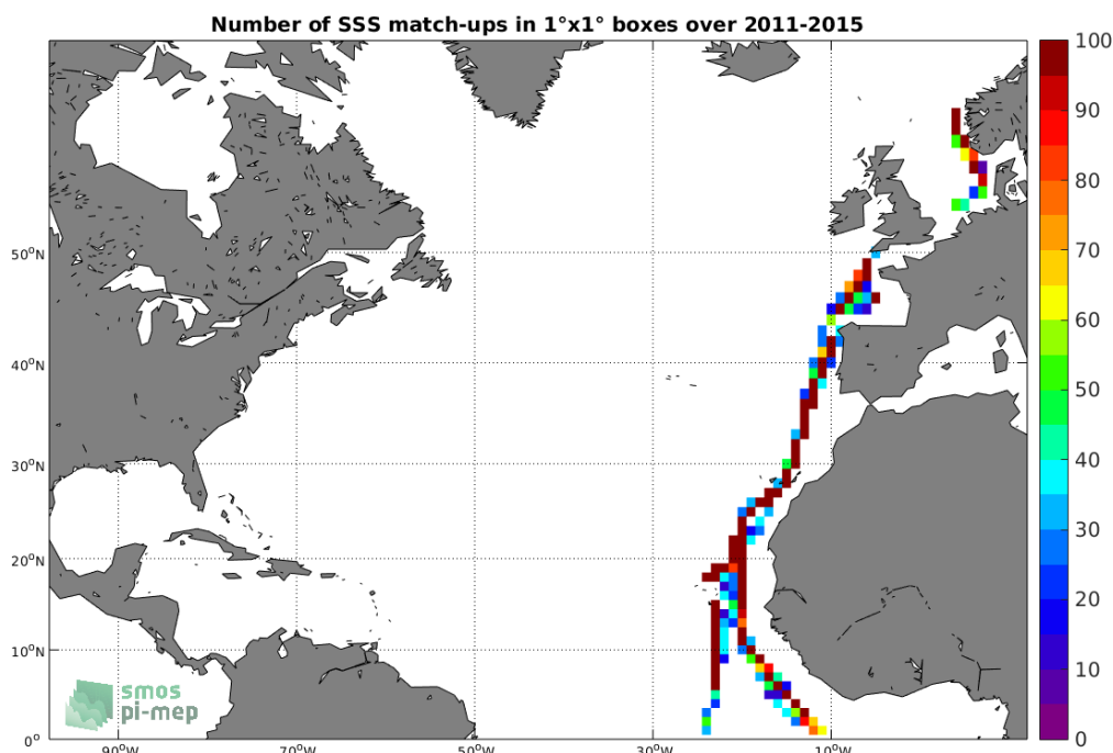
Figure 4: Number of SSS match-ups between TSG-POLARSTERN SSS and the Aquarius-L3-OR-V5-7DAY-RUNNING-RAIN-MASK-1DEG SSS product for the North Atlantic Ocean Pi-MEP region over 1^{\circ} \times 1^{\circ} boxes and for the full satellite product period.
