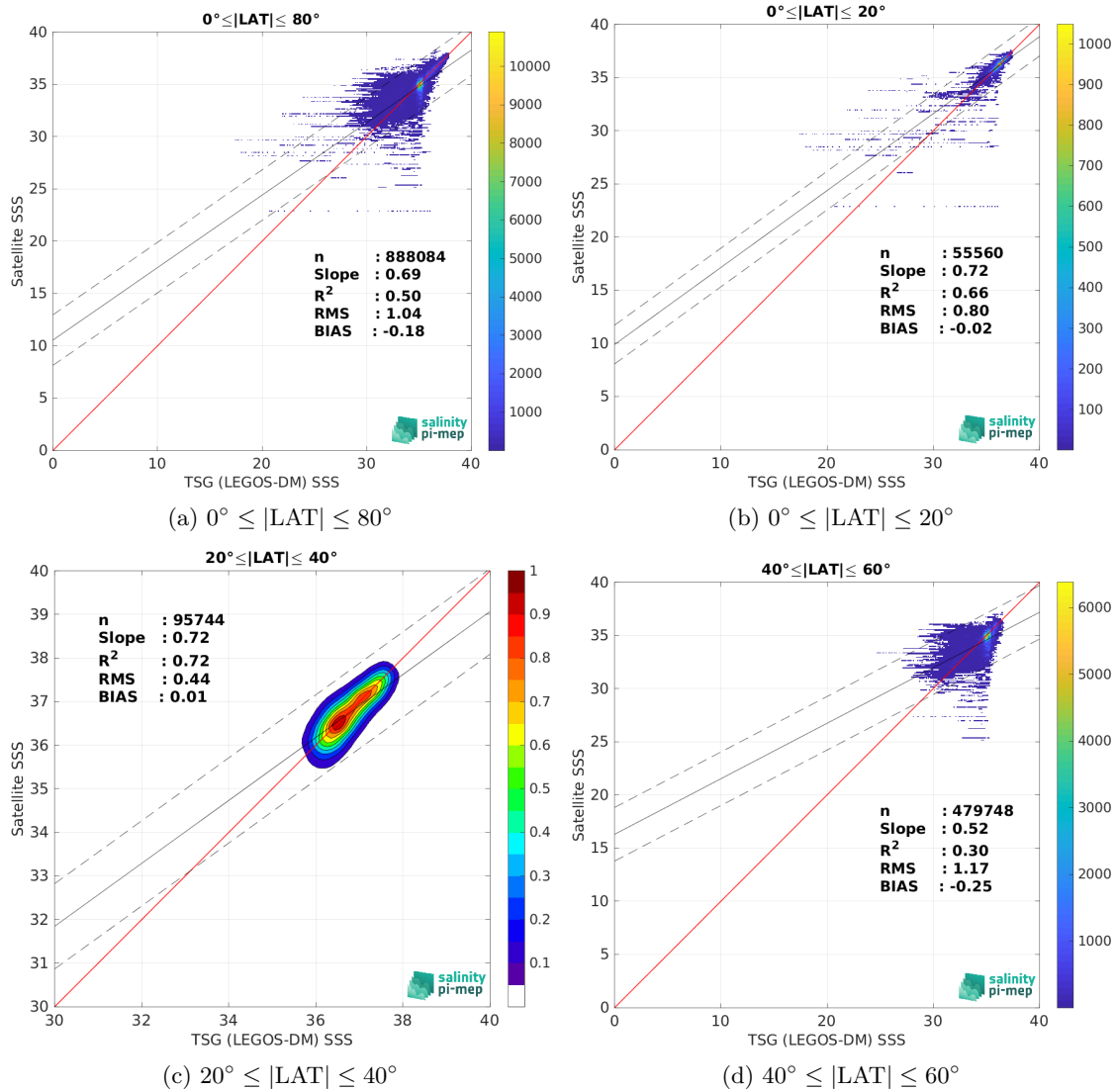
Figure 10: Contour maps of the concentration of Aquarius SSS L3 OR v5 - 7-Day running - Rain mask (NASA-GSFC) SSS (y-axis) versus TSG (LEGOS-DM) SSS (x-axis) at match-up pairs for different latitude bands. For each plot, the red line shows x=y . The black thin and dashed lines indicate a linear fit through the data cloud and the \pm 95\% confidence levels, respectively. The number match-up pairs n , the slope and R^2 coefficient of the linear fit, the root mean square (RMS) and the mean bias between satellite and in situ data are indicated for each latitude band in each plots.
