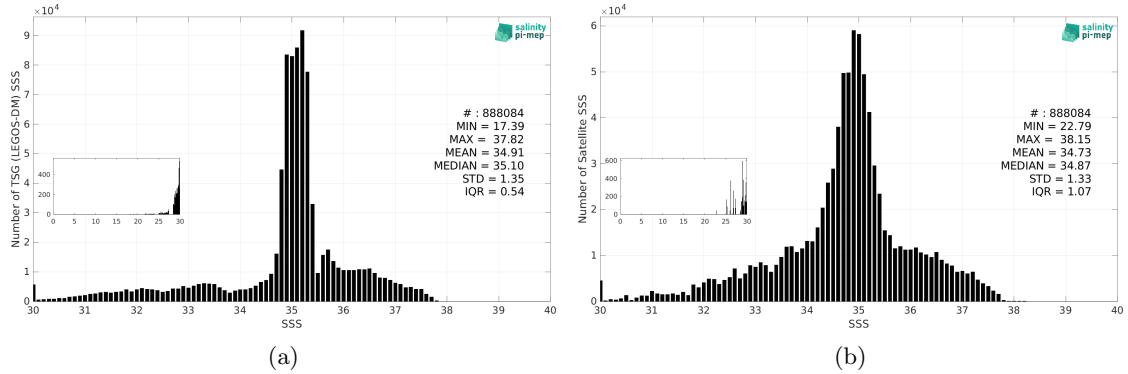
Figure 3: Histograms of SSS from TSG (LEGOS-DM) (a) and Aquarius SSS L3 OR v5 - 7-Day running - Rain mask (NASA-GSFC) (b) considering all match-up pairs per bins of 0.1 over the North Atlantic Ocean Pi-MEP region and for the full satellite product period.
