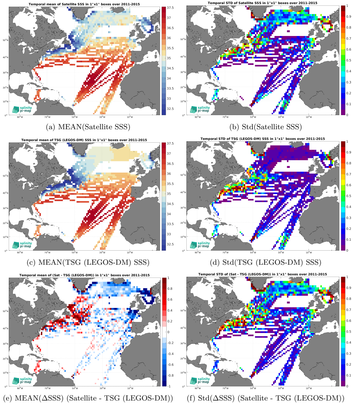
Figure 7: Temporal mean (left) and Std (right) of SSS from Aquarius SSS L3 OR v5 - 7-Day running - Rain mask (NASA-GSFC) (top), TSG (LEGOS-DM) (middle), and of \Delta SSS (Satellite - TSG (LEGOS-DM)). Only match-up pairs are used to generate these maps.
