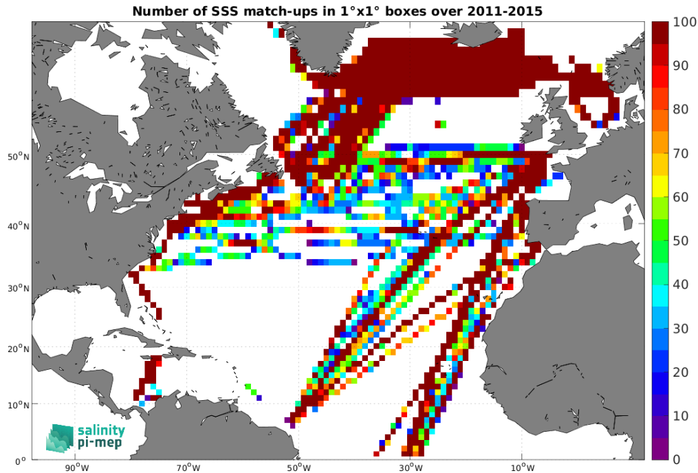
Figure 5: Number of SSS match-ups between TSG (LEGOS-DM) SSS and the Aquarius SSS L3 OR v5 - 7-Day running - Rain mask (NASA-GSFC) SSS product for the North Atlantic Ocean Pi-MEP region over 1^\circ \times 1^\circ boxes and for the full satellite product period.
