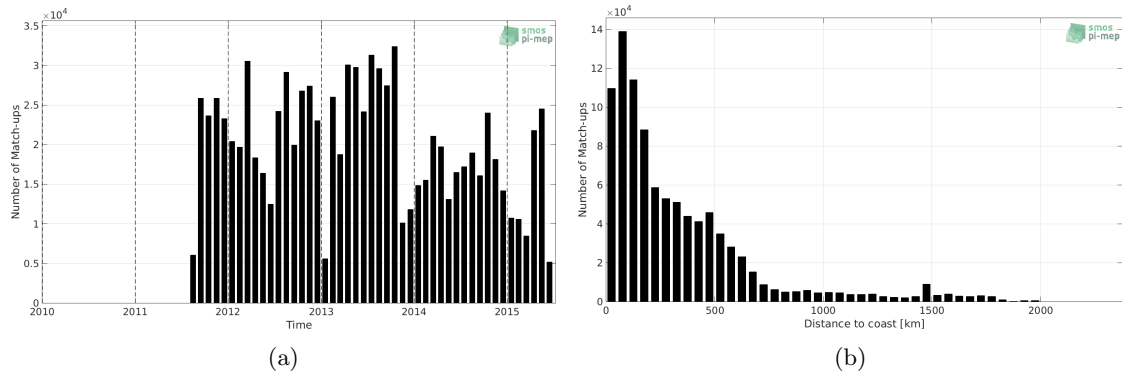
Figure 1: Number of match-ups between TSG-LEGOS-DM and Aquarius-L3-OR-V5-7DAY-RUNNING-RAIN-MASK-1DEG SSS as a function of time (a) and as function of the distance to coast (b) over the North Atlantic Ocean Pi-MEP region and for the full satellite product period.
