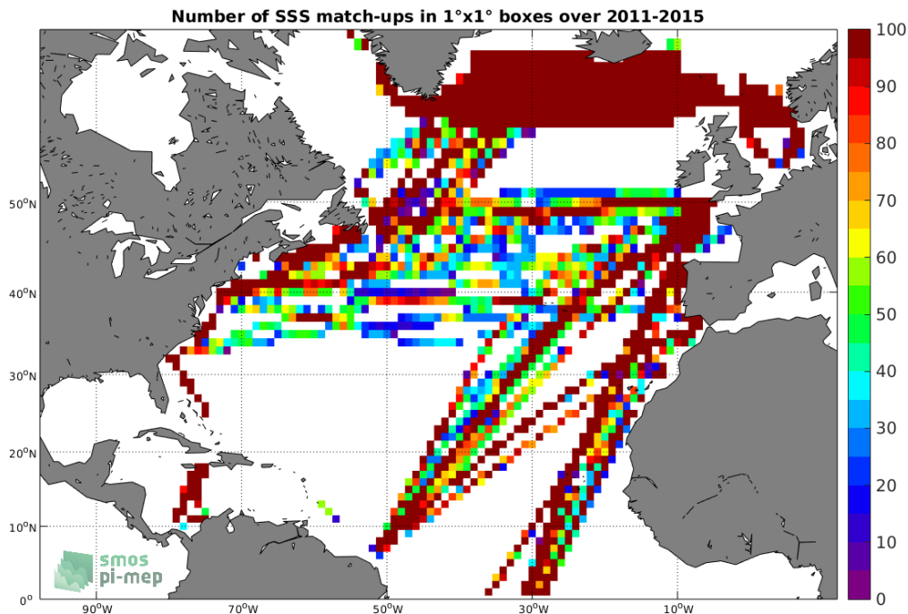
Figure 4: Number of SSS match-ups between TSG-LEGOS-DM SSS and the Aquarius-L3-OR-V5-7DAY-RUNNING-RAIN-MASK-1DEG SSS product for the North Atlantic Ocean Pi-MEP region over 1^\circ \times 1^\circ boxes and for the full satellite product period.
