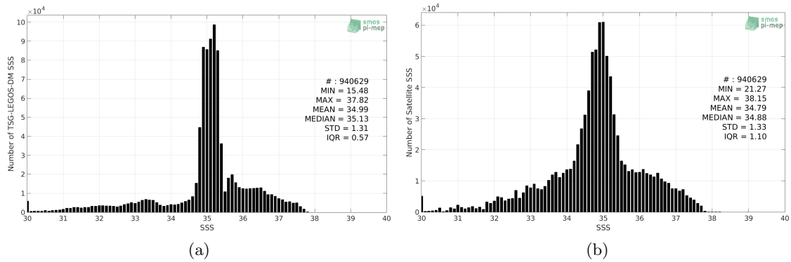
Figure 2: Histograms of SSS from TSG-LEGOS-DM (a) and Aquarius-L3-OR-V5-7DAY-RUNNING-RAIN-MASK-1DEG (b) considering all match-up pairs per bins of 0.1 over the North Atlantic Ocean Pi-MEP region and for the full satellite product period.
