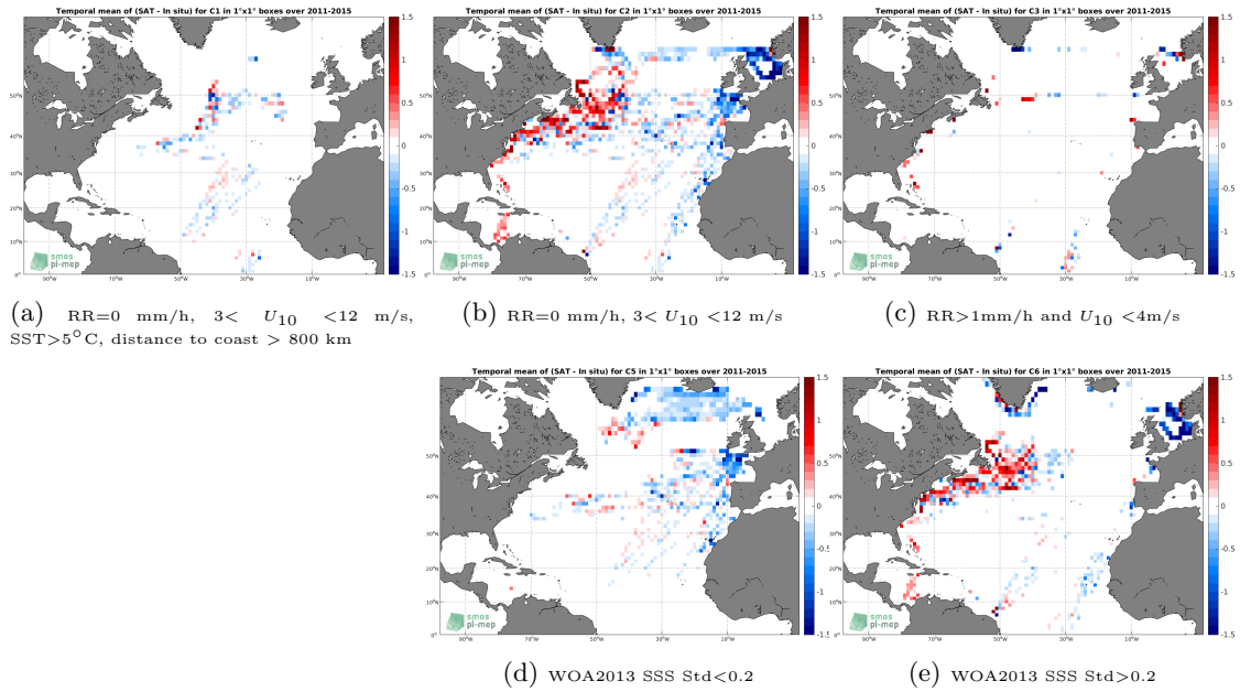
Figure 12: Temporal mean gridded over spatial boxes of size 1^\circ \times 1^\circ of \Delta SSS (Aquarius-L3-OR-V5-7DAY-RUNNING-RAIN-MASK-1DEG - TSG-LEGOS-DM) for 5 different subdatasets corresponding to:RR=0 mm/h, 3 < U_{10} < 12 m/s, SST >5^\circ\text{C} , distance to coast > 800 km (a), RR=0 mm/h, 3 < U_{10} < 12 m/s (b), RR >1 mm/h and U_{10} < 4 m/s (c), WOA2013 SSS Std <0.2 (d), WOA2013 SSS Std >0.2 (e).
