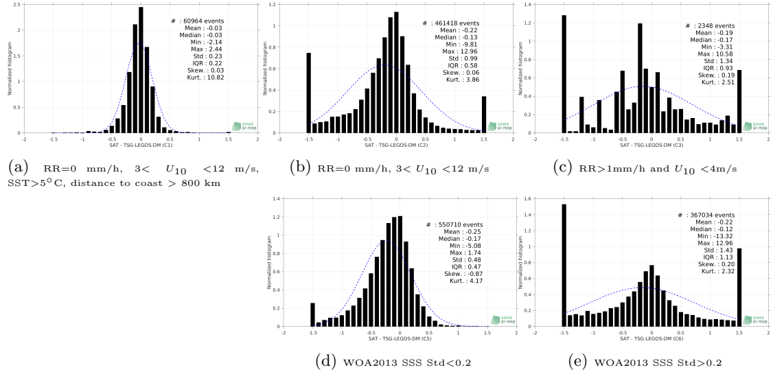
Figure 13: Normalized histogram of \Delta\text{SSS} (Aquarius-L3-OR-V5-7DAY-RUNNING-RAIN-MASK-1DEG - TSG-LEGOS-DM) for 5 different subdatasets corresponding to: RR=0 mm/h, 3 < U_{10} < 12 m/s, SST > 5^\circ\text{C} , distance to coast > 800 km (a), RR=0 mm/h, 3 < U_{10} < 12 m/s (b), RR > 1 mm/h and U_{10} < 4 m/s (c), WOA2013 SSS Std < 0.2 (d), WOA2013 SSS Std > 0.2 (e).
