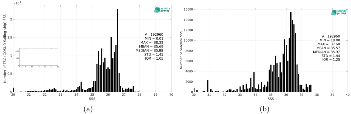
Figure 2: Histograms of SSS from TSG (GOSUD-Sailing-ship) (a) and Aquarius SSS L3 OR v5 - 7-Day running - Rain mask (NASA-GSFC) (b) considering all match-up pairs per bins of 0.1 over the North Atlantic Ocean Pi-MEP region and for the full satellite product period.
