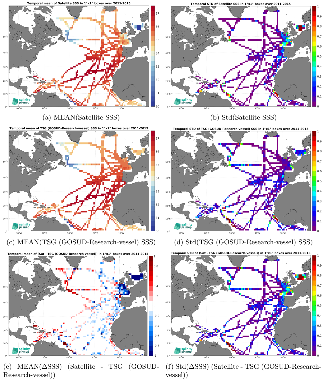
Figure 7: Temporal mean (left) and Std (right) of SSS from Aquarius SSS L3 OR v5 - 7-Day running - Rain mask (NASA-GSFC) (top), TSG (GOSUD-Research-vessel) (middle), and of \Delta SSS (Satellite - TSG (GOSUD-Research-vessel)). Only match-up pairs are used to generate these maps.
