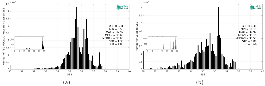
Figure 3: Histograms of SSS from TSG (GOSUD-Research-vessel) (a) and Aquarius SSS L3 OR v5 - 7-Day running - Rain mask (NASA-GSFC) (b) considering all match-up pairs per bins of 0.1 over the North Atlantic Ocean Pi-MEP region and for the full satellite product period.
