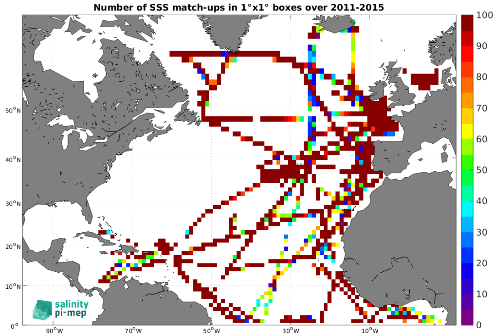
Figure 5: Number of SSS match-ups between TSG (GOSUD-Research-vessel) SSS and the Aquarius SSS L3 OR v5 - 7-Day running - Rain mask (NASA-GSFC) SSS product for the North Atlantic Ocean Pi-MEP region over 1^\circ \times 1^\circ boxes and for the full satellite product period.
