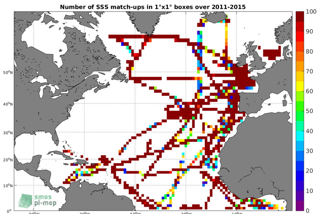
Figure 4: Number of SSS match-ups between TSG-GOSUD-Research-vessel SSS and the Aquarius-L3-OR-V5-7DAY-RUNNING-RAIN-MASK-1DEG SSS product for the North Atlantic Ocean Pi-MEP region over 1°x1° boxes and for the full satellite product period.
