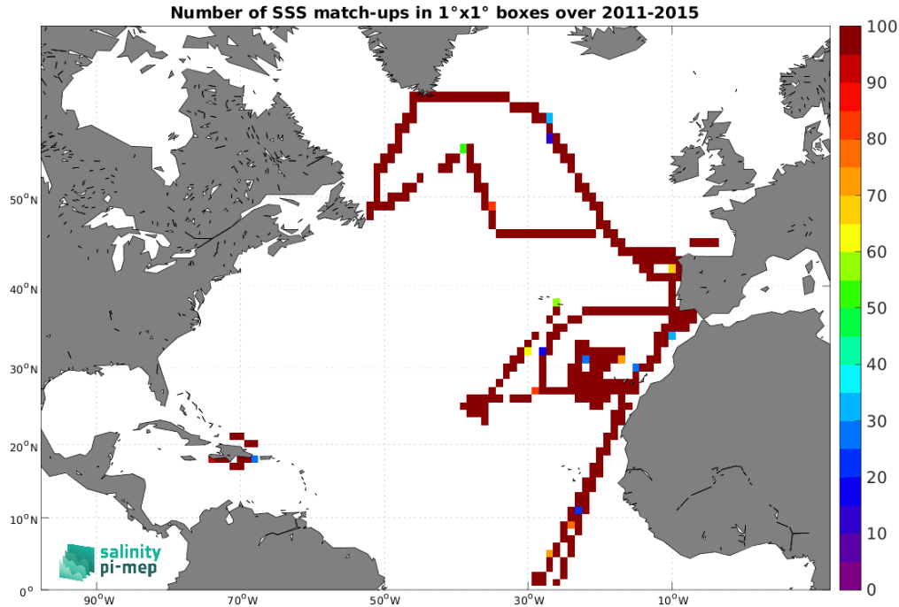
Figure 4: Number of SSS match-ups between TSG (CSIC-UTM) SSS and the Aquarius SSS L3 OR v5 - 7-Day running - Rain mask (NASA-GSFC) SSS product for the North Atlantic Ocean Pi-MEP region over 1^\circ \times 1^\circ boxes and for the full satellite product period.
