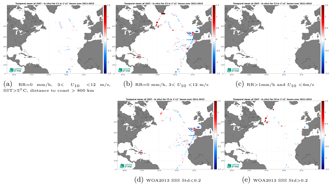
Figure 12: Temporal mean gridded over spatial boxes of size 1^\circ \times 1^\circ of \Delta SSS (Aquarius SSS L3 OR v5 - 7-Day running - Rain mask (NASA-GSFC) - TSG (CSIC-UTM)) for 5 different subdatasets corresponding to:RR=0 mm/h, 3 < U_{10} < 12 m/s, SST >5^\circ\text{C} , distance to coast > 800 km (a), RR=0 mm/h, 3 < U_{10} < 12 m/s (b), RR >1 mm/h and U_{10} < 4 m/s (c), WOA2013 SSS Std <0.2 (d), WOA2013 SSS Std >0.2 (e).
