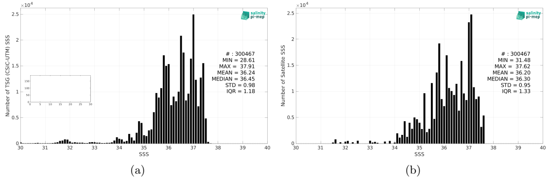
Figure 2: Histograms of SSS from TSG (CSIC-UTM) (a) and Aquarius SSS L3 OR v5 - 7-Day running - Rain mask (NASA-GSFC) (b) considering all match-up pairs per bins of 0.1 over the North Atlantic Ocean Pi-MEP region and for the full satellite product period.
