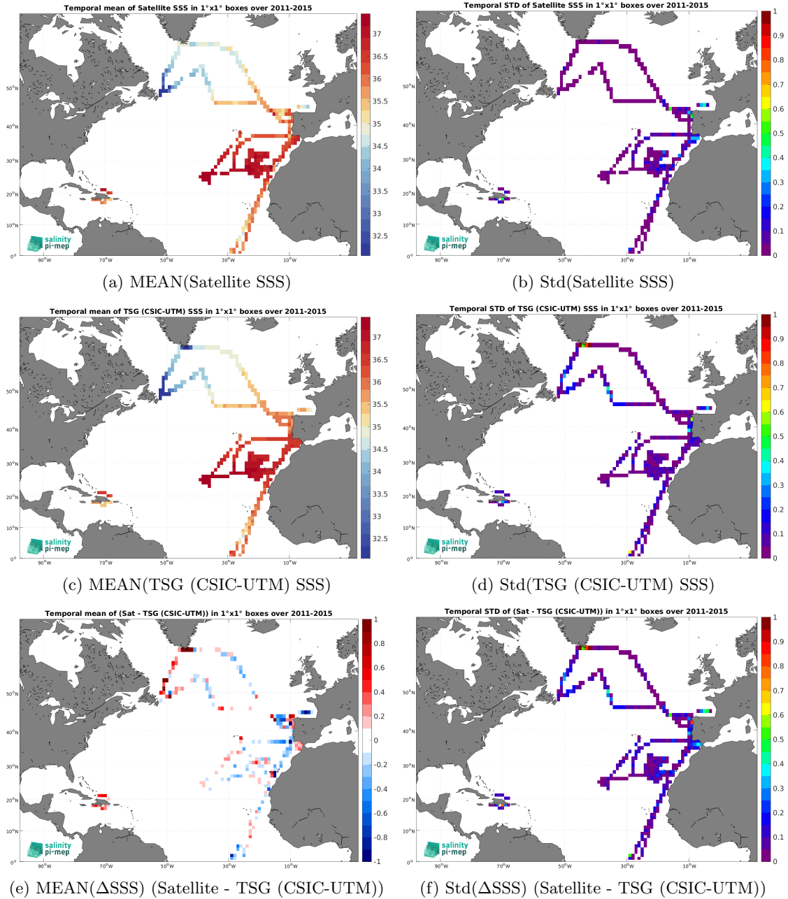
Figure 6: Temporal mean (left) and Std (right) of SSS from Aquarius SSS L3 OR v5 - 7-Day running - Rain mask (NASA-GSFC) (top), TSG (CSIC-UTM) (middle), and of \Delta SSS (Satellite - TSG (CSIC-UTM)). Only match-up pairs are used to generate these maps.
