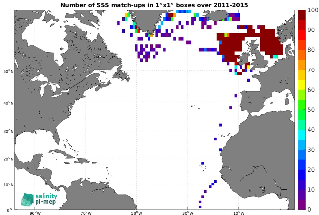
Figure 5: Number of SSS match-ups between ICES SSS and the Aquarius SSS L3 OR v5 - 7-Day running - Rain mask (NASA-GSFC) SSS product for the North Atlantic Ocean Pi-MEP region over 1^\circ \times 1^\circ boxes and for the full satellite product period.
