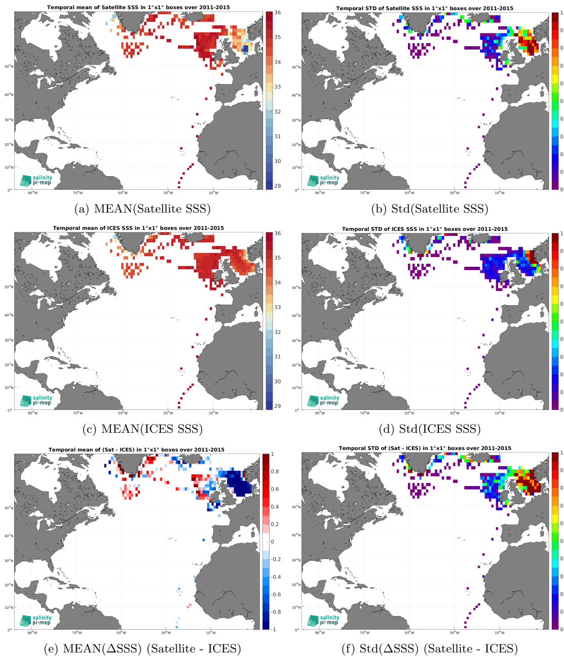
Figure 7: Temporal mean (left) and Std (right) of SSS from Aquarius SSS L3 OR v5 - 7-Day running - Rain mask (NASA-GSFC) (top), ICES (middle), and of \Delta SSS (Satellite - ICES). Only match-up pairs are used to generate these maps.
