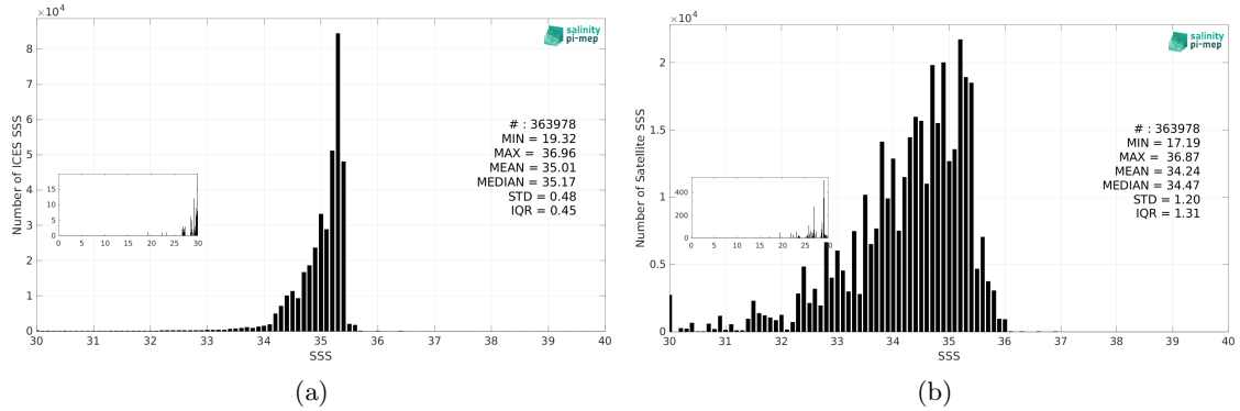
Figure 3: Histograms of SSS from ICES (a) and Aquarius SSS L3 OR v5 - 7-Day running - Rain mask (NASA-GSFC) (b) considering all match-up pairs per bins of 0.1 over the North Atlantic Ocean Pi-MEP region and for the full satellite product period.
