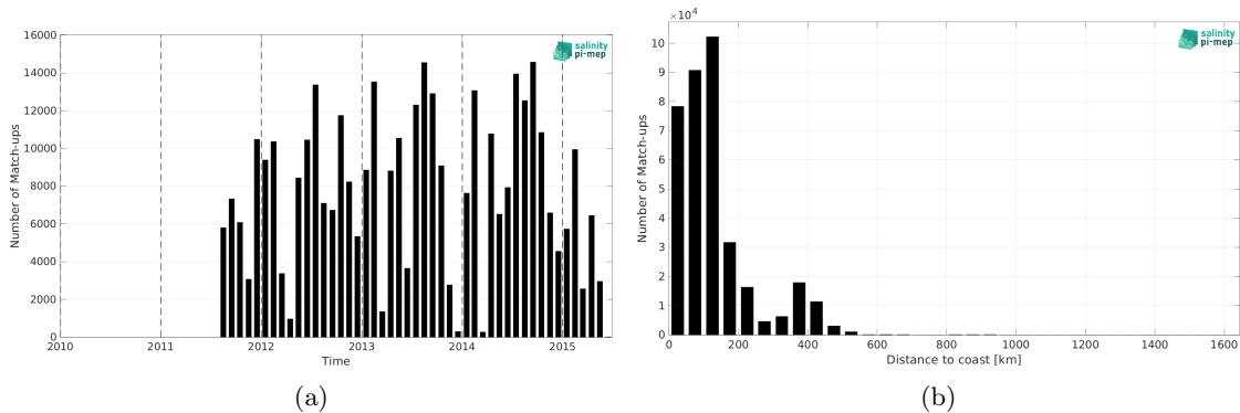
Figure 2: Number of match-ups between ICES and Aquarius SSS L3 OR v5 - 7-Day running - Rain mask (NASA-GSFC) SSS as a function of time (a) and as function of the distance to coast (b) over the North Atlantic Ocean Pi-MEP region and for the full satellite product period.
