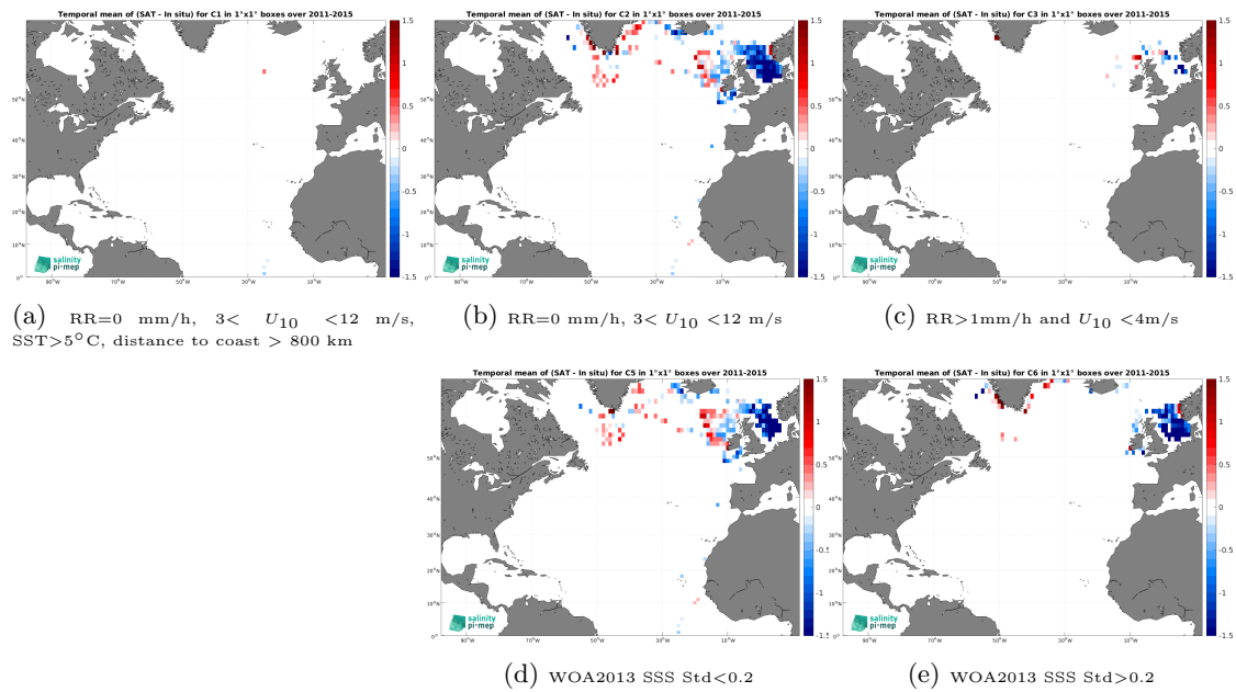
Figure 14: Temporal mean gridded over spatial boxes of size 1^\circ \times 1^\circ of \Delta SSS (Aquarius SSS L3 OR v5 - 7-Day running - Rain mask (NASA-GSFC) - ICES) for 5 different subdatasets corresponding to:RR=0 mm/h, 3 < U_{10} < 12 m/s, SST >5^\circ\text{C} , distance to coast > 800 km (a), RR=0 mm/h, 3 < U_{10} < 12 m/s (b), RR >1 mm/h and U_{10} < 4 m/s (c), WOA2013 SSS Std <0.2 (d), WOA2013 SSS Std >0.2 (e).
