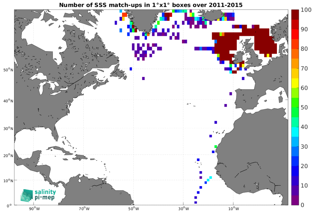
Figure 4: Number of SSS match-ups between ICES SSS and the Aquarius SSS L3 OR v5 - 7-Day running - Rain mask (NASA-GSFC) SSS product for the North Atlantic Ocean Pi-MEP region over 1^\circ \times 1^\circ boxes and for the full satellite product period.
