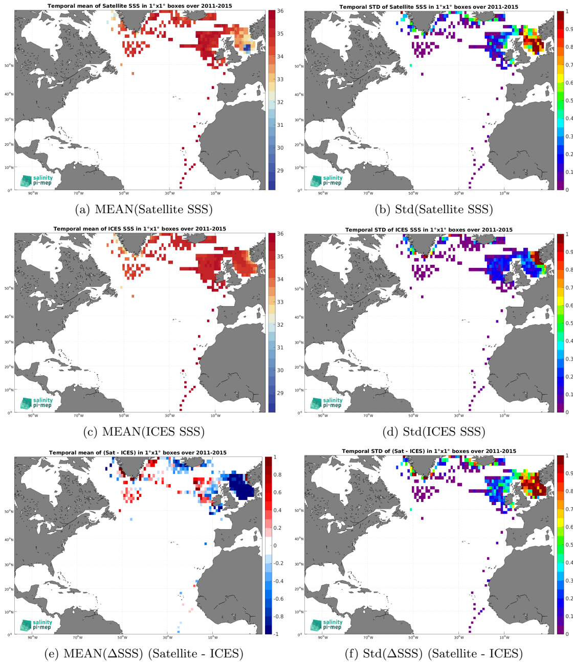
Figure 6: Temporal mean (left) and Std (right) of SSS from Aquarius SSS L3 OR v5 - 7-Day running - Rain mask (NASA-GSFC) (top), ICES (middle), and of \Delta SSS (Satellite - ICES). Only match-up pairs are used to generate these maps.
