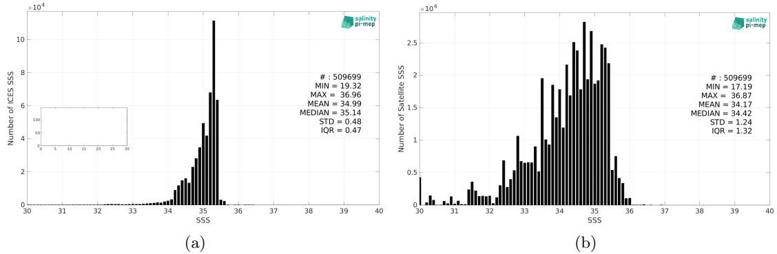
Figure 2: Histograms of SSS from ICES (a) and Aquarius SSS L3 OR v5 - 7-Day running - Rain mask (NASA-GSFC) (b) considering all match-up pairs per bins of 0.1 over the North Atlantic Ocean Pi-MEP region and for the full satellite product period.
