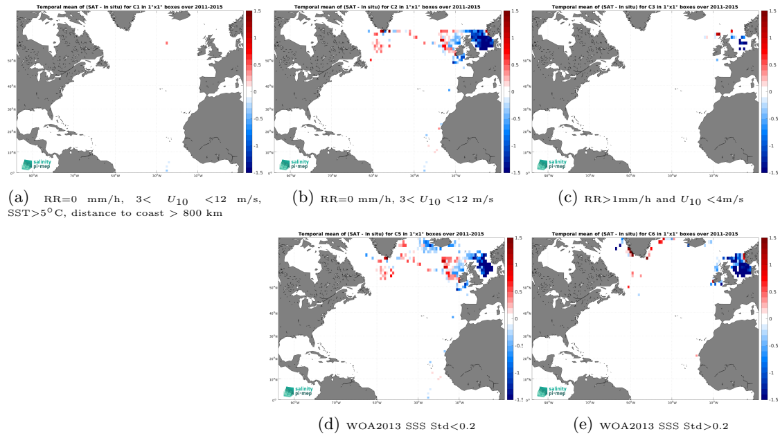
Figure 12: Temporal mean gridded over spatial boxes of size 1^\circ \times 1^\circ of \Delta SSS (Aquarius SSS L3 OR v5 - 7-Day running - Rain mask (NASA-GSFC) - ICES) for 5 different subdatasets corresponding to:RR=0 mm/h, 3 < U_{10} < 12 m/s, SST >5^\circ\text{C} , distance to coast > 800 km (a), RR=0 mm/h, 3 < U_{10} < 12 m/s (b), RR >1 mm/h and U_{10} < 4 m/s (c), WOA2013 SSS Std <0.2 (d), WOA2013 SSS Std >0.2 (e).
