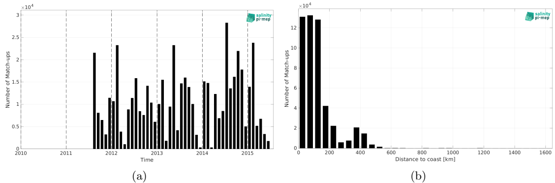
Figure 1: Number of match-ups between ICES and Aquarius SSS L3 OR v5 - 7-Day running - Rain mask (NASA-GSFC) SSS as a function of time (a) and as function of the distance to coast (b) over the North Atlantic Ocean Pi-MEP region and for the full satellite product period.
