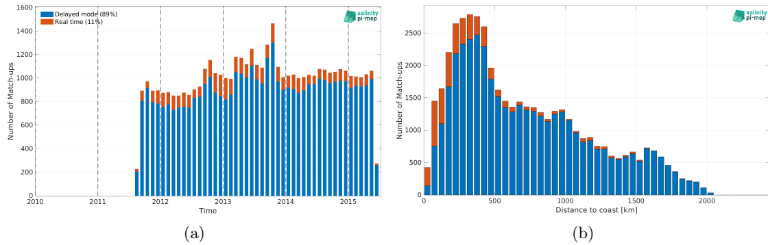
Figure 2: Number of match-ups between Argo and Aquarius SSS L3 OR v5 - 7-Day running - Rain mask (NASA-GSFC) SSS as a function of time (a) and as function of the distance to coast (b) over the North Atlantic Ocean Pi-MEP region and for the full satellite product period.
