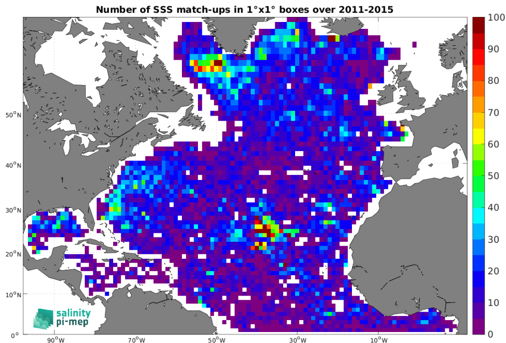
Figure 5: Number of SSS match-ups between Argo SSS and the Aquarius SSS L3 OR v5 - 7-Day running - Rain mask (NASA-GSFC) SSS product for the North Atlantic Ocean Pi-MEP region over 1^\circ \times 1^\circ boxes and for the full satellite product period.
