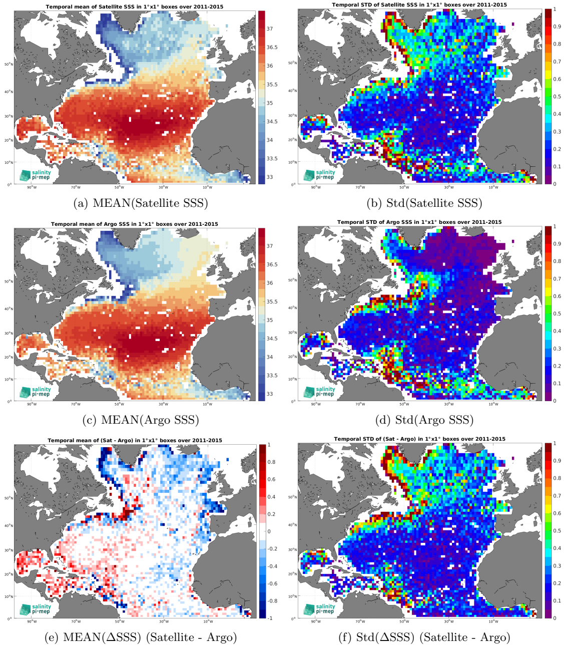
Figure 7: Temporal mean (left) and Std (right) of SSS from Aquarius SSS L3 OR v5 - 7-Day running - Rain mask (NASA-GSFC) (top), Argo (middle), and of \Delta SSS (Satellite - Argo). Only match-up pairs are used to generate these maps.
