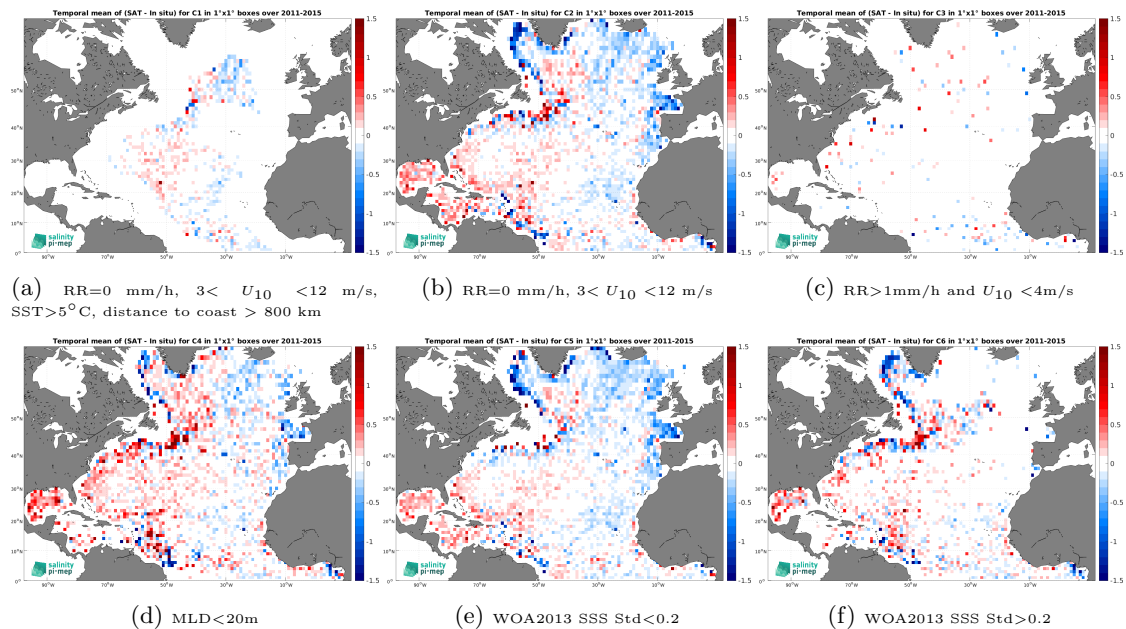
Figure 14: Temporal mean gridded over spatial boxes of size 1^\circ \times 1^\circ of \Delta SSS (Aquarius SSS L3 OR v5 - 7-Day running - Rain mask (NASA-GSFC) - Argo) for 6 different subdatasets corresponding to: RR=0 mm/h, 3 < U_{10} < 12 m/s, SST > 5^\circ\text{C} , distance to coast > 800 km (a), RR=0 mm/h, 3 < U_{10} < 12 m/s (b), RR > 1 mm/h and U_{10} < 4 m/s (c), MLD < 20 m (d), WOA2013 SSS Std < 0.2 (e), WOA2013 SSS Std > 0.2 (f).
