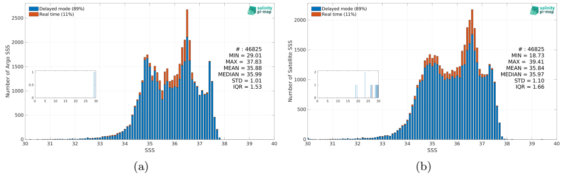
Figure 3: Histograms of SSS from Argo (a) and Aquarius SSS L3 OR v5 - 7-Day running - Rain mask (NASA-GSFC) (b) considering all match-up pairs per bins of 0.1 over the North Atlantic Ocean Pi-MEP region and for the full satellite product period.
