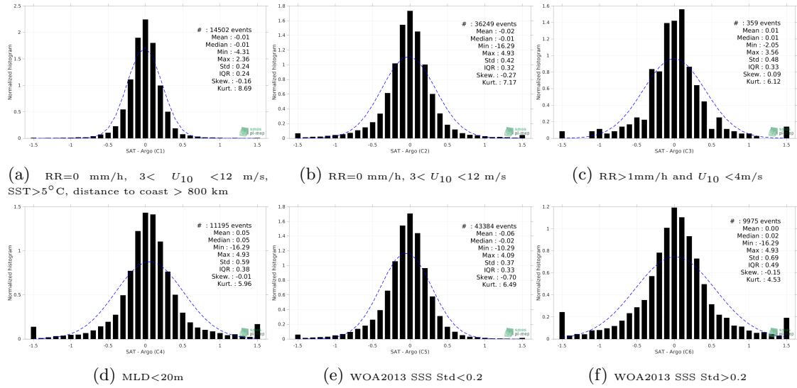
Figure 13: Normalized histogram of \Delta\text{SSS} (Aquarius SSS L3 OR v5 - 7-Day running - Rain mask (NASA-GSFC) - Argo) for 6 different subdatasets corresponding to: RR=0 mm/h, 3 < U_{10} < 12 m/s, SST>5°C, distance to coast > 800 km (a), RR=0 mm/h, 3 < U_{10} < 12 m/s (b), RR>1mm/h and U_{10} < 4 m/s (c), MLD<20m (d), WOA2013 SSS Std<0.2 (e), WOA2013 SSS Std>0.2 (f).
