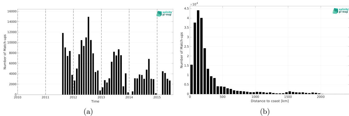
Figure 2: Number of match-ups between TSG (SAMOS) and Aquarius SSS L3 OR v5 - Monthly (NASA-GSFC) SSS as a function of time (a) and as function of the distance to coast (b) over the North Atlantic Ocean Pi-MEP region and for the full satellite product period.
