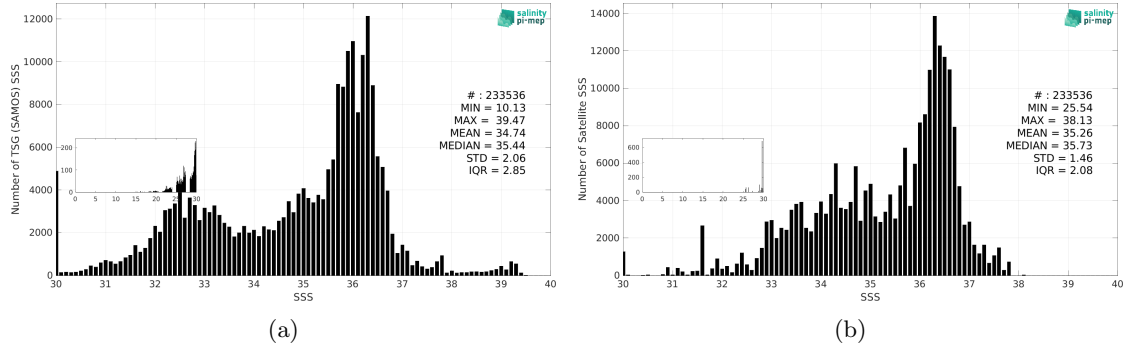
Figure 3: Histograms of SSS from TSG (SAMOS) (a) and Aquarius SSS L3 OR v5 - Monthly (NASA-GSFC) (b) considering all match-up pairs per bins of 0.1 over the North Atlantic Ocean Pi-MEP region and for the full satellite product period.
