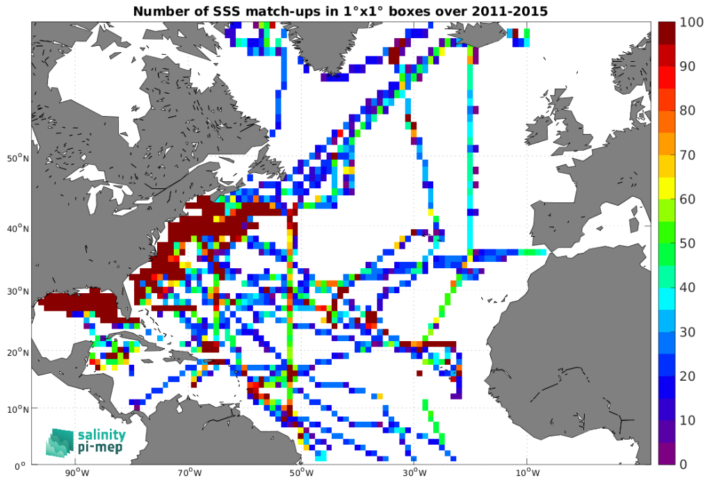
Figure 5: Number of SSS match-ups between TSG (SAMOS) SSS and the Aquarius SSS L3 OR v5 - Monthly (NASA-GSFC) SSS product for the North Atlantic Ocean Pi-MEP region over 1^\circ \times 1^\circ boxes and for the full satellite product period.
